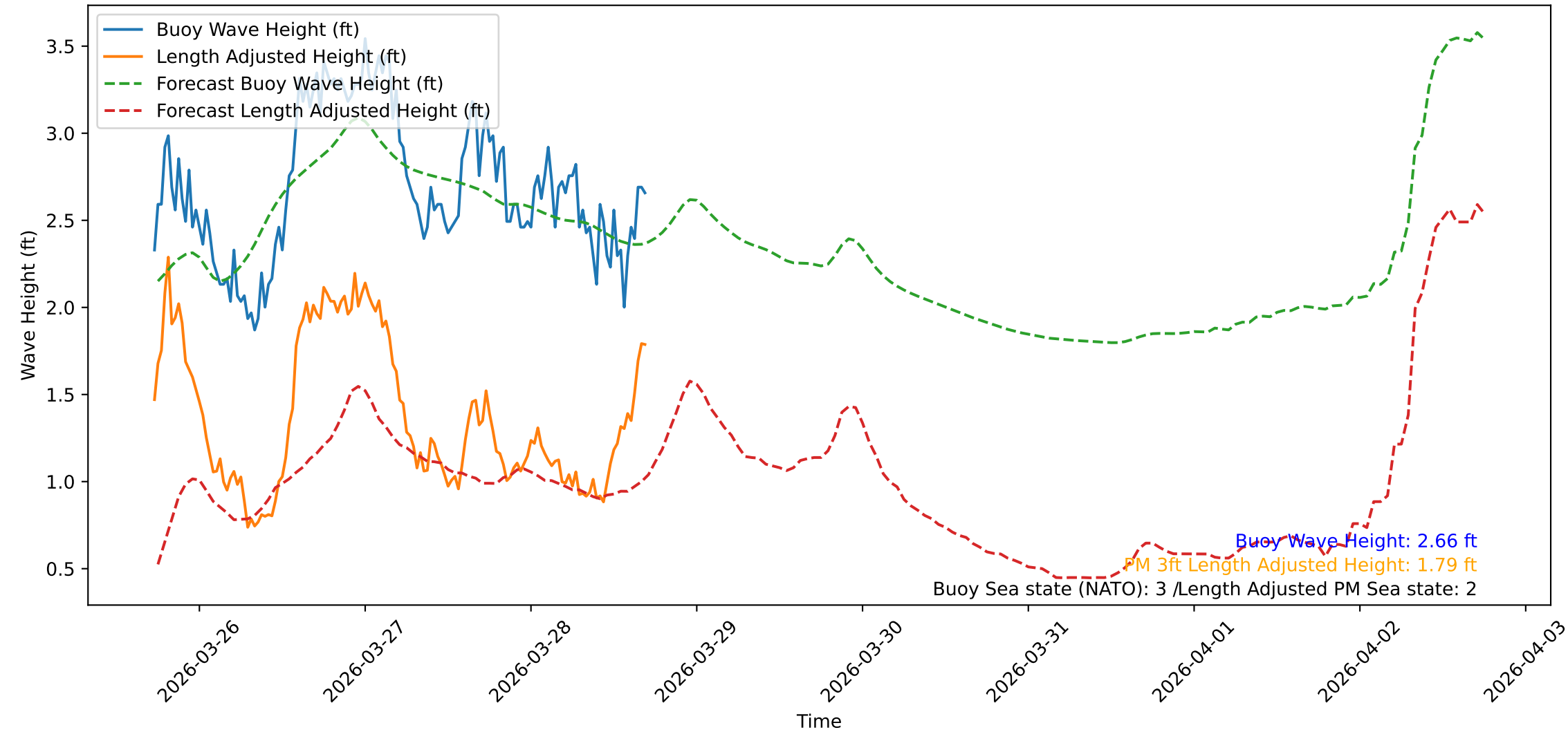
Wave Heights over Time for Green Beach at 2026-03-28 17:31:10
