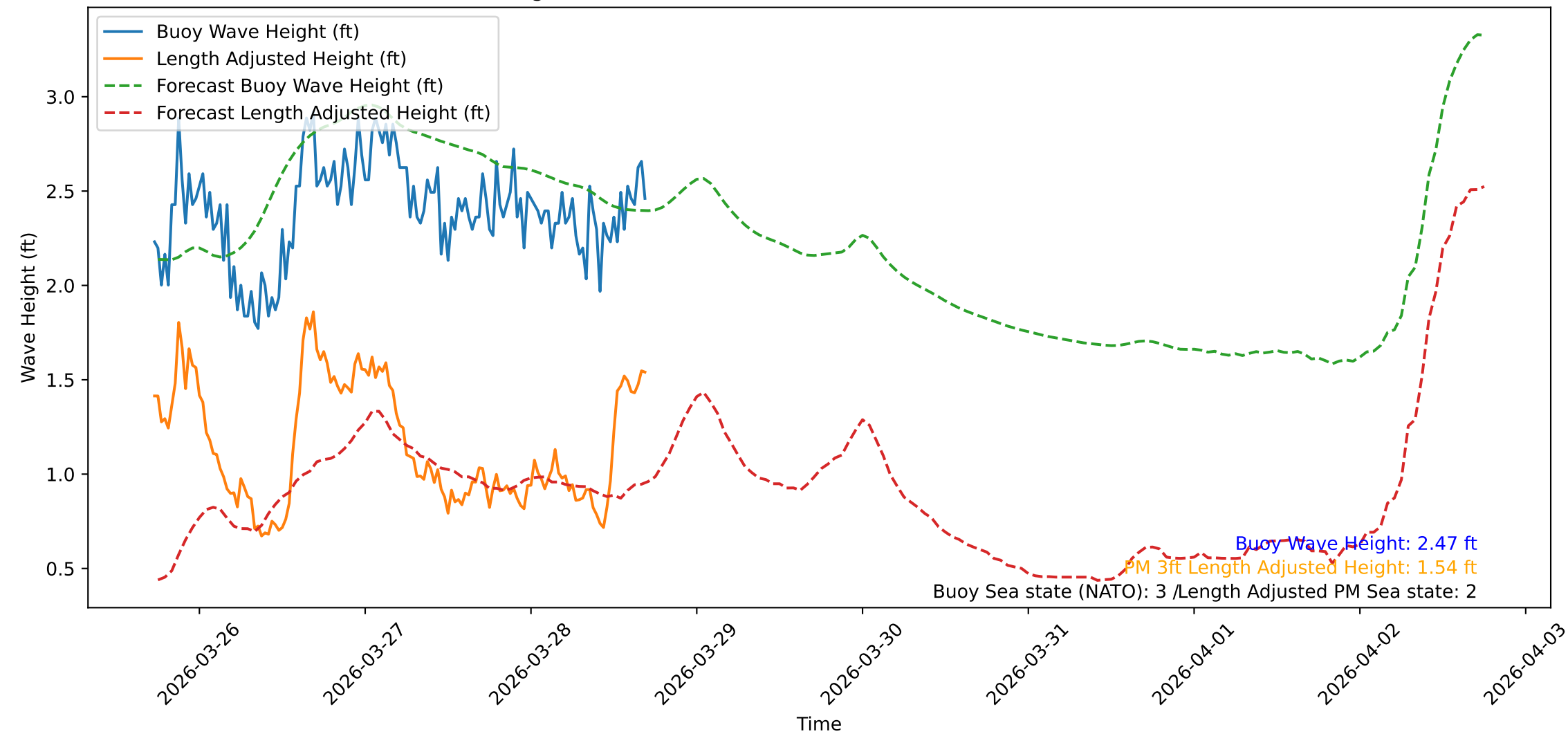
Wave Heights over Time for Oceanside Harbor at 2026-03-28 17:30:32
