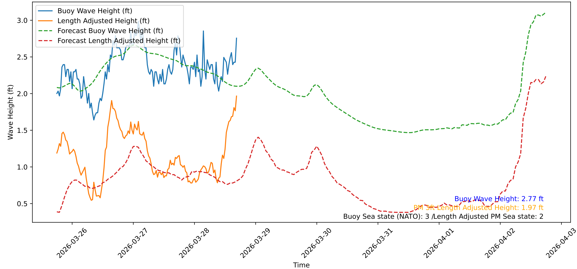
Wave Heights over Time for Red Beach at 2026-03-28 17:30:48
