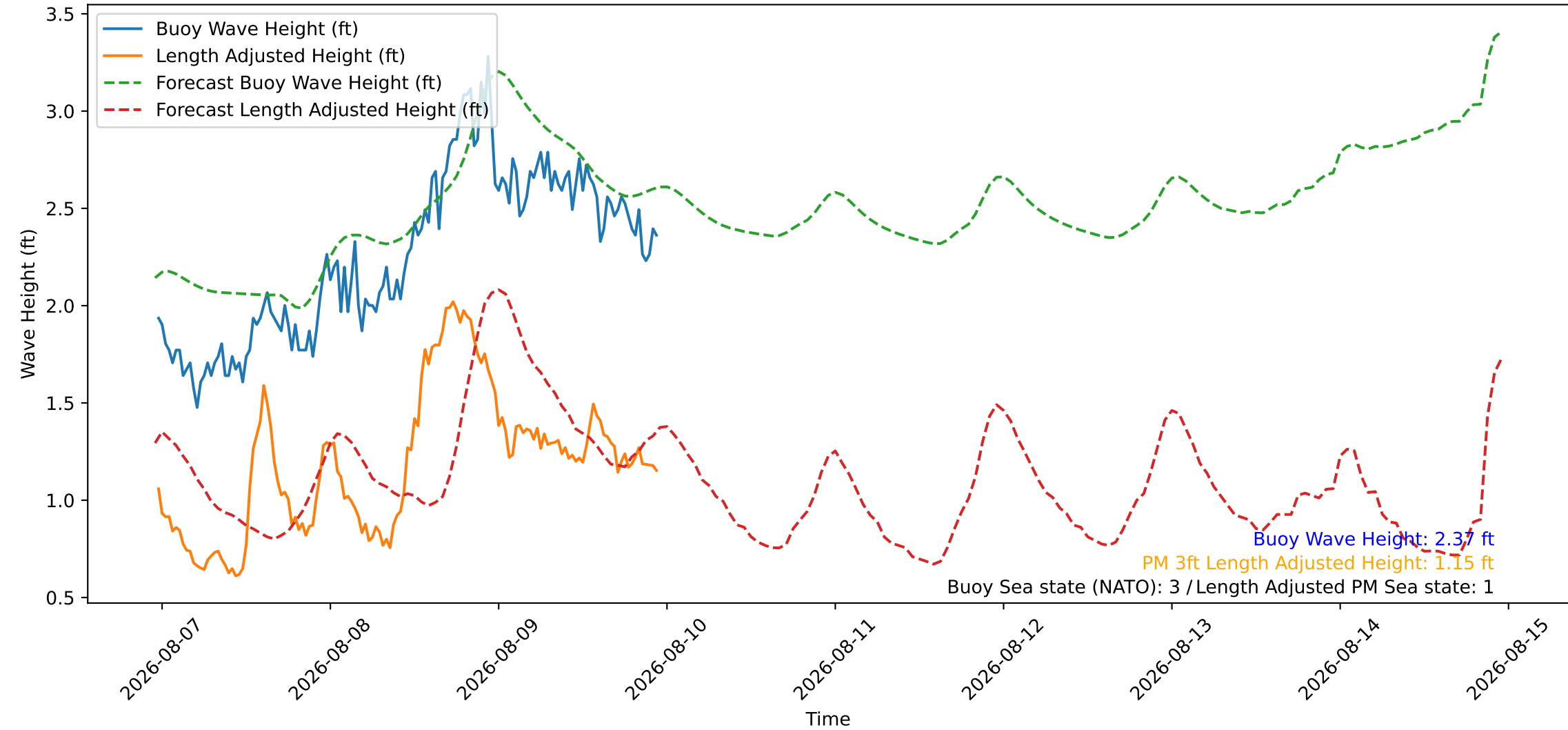
Wave Heights over Time for Red Beach at 2026-08-09 23:20:48
