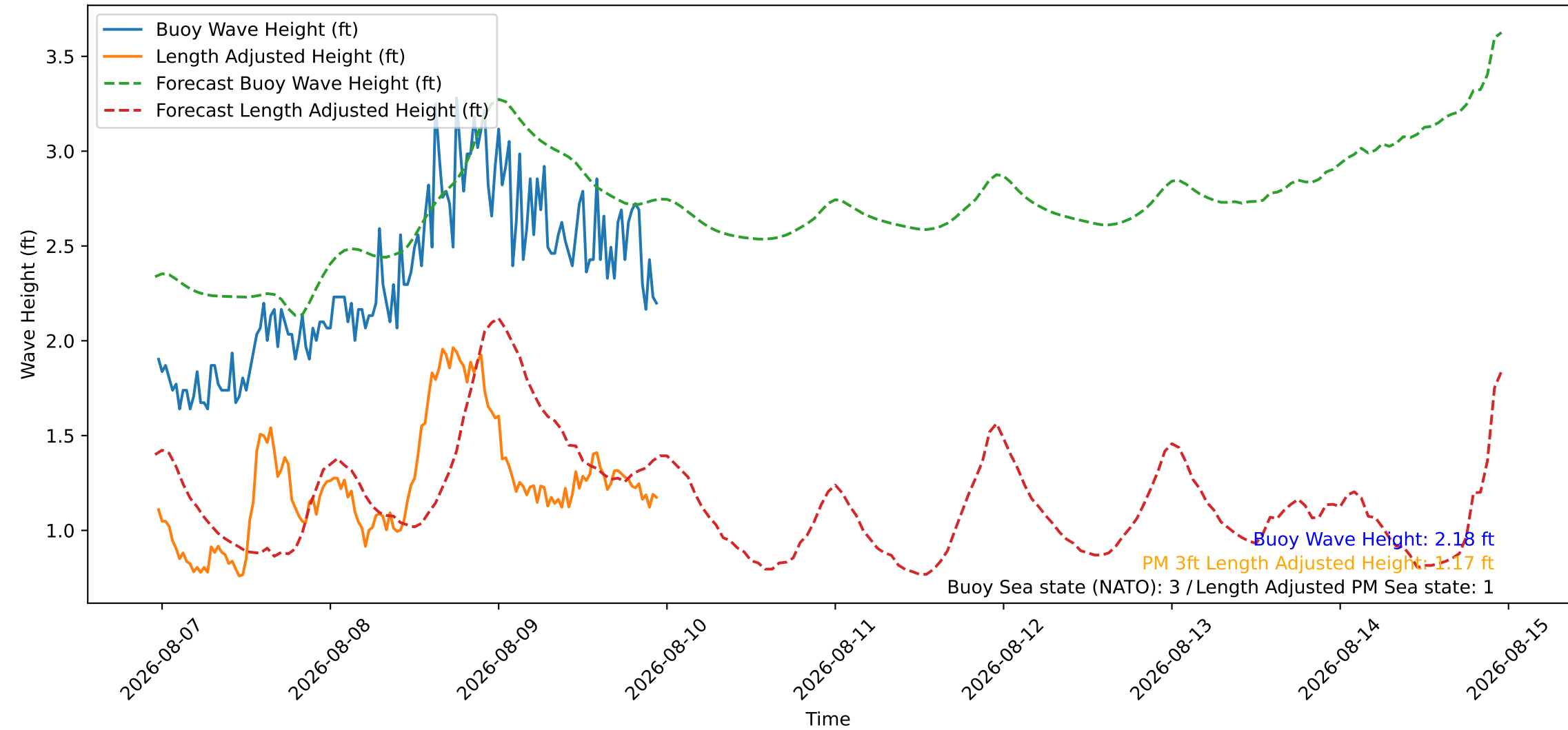
Wave Heights over Time for Oceanside Harbor at 2026-08-09 23:20:26
