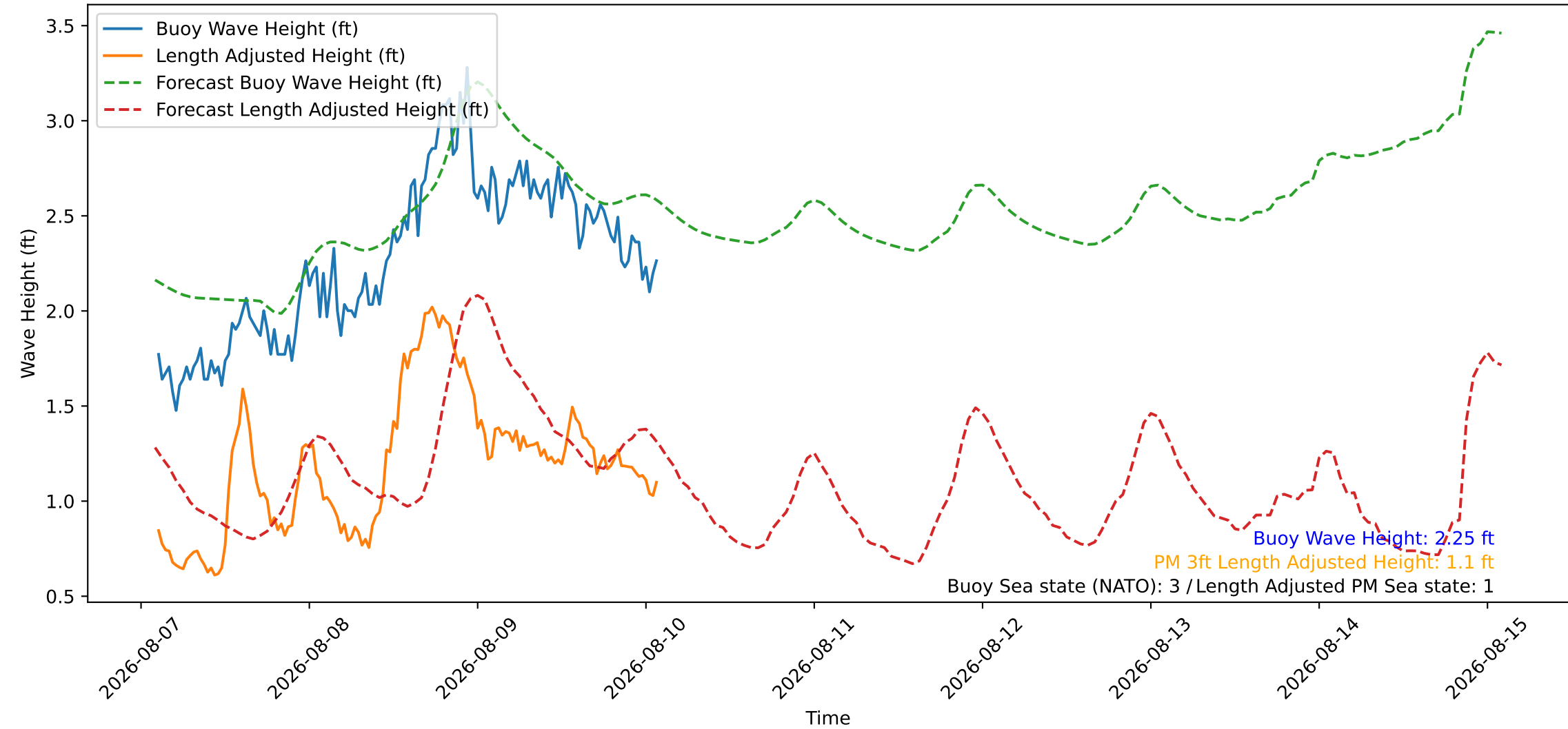
Wave Heights over Time for Red Beach at 2026-08-10 02:20:48
