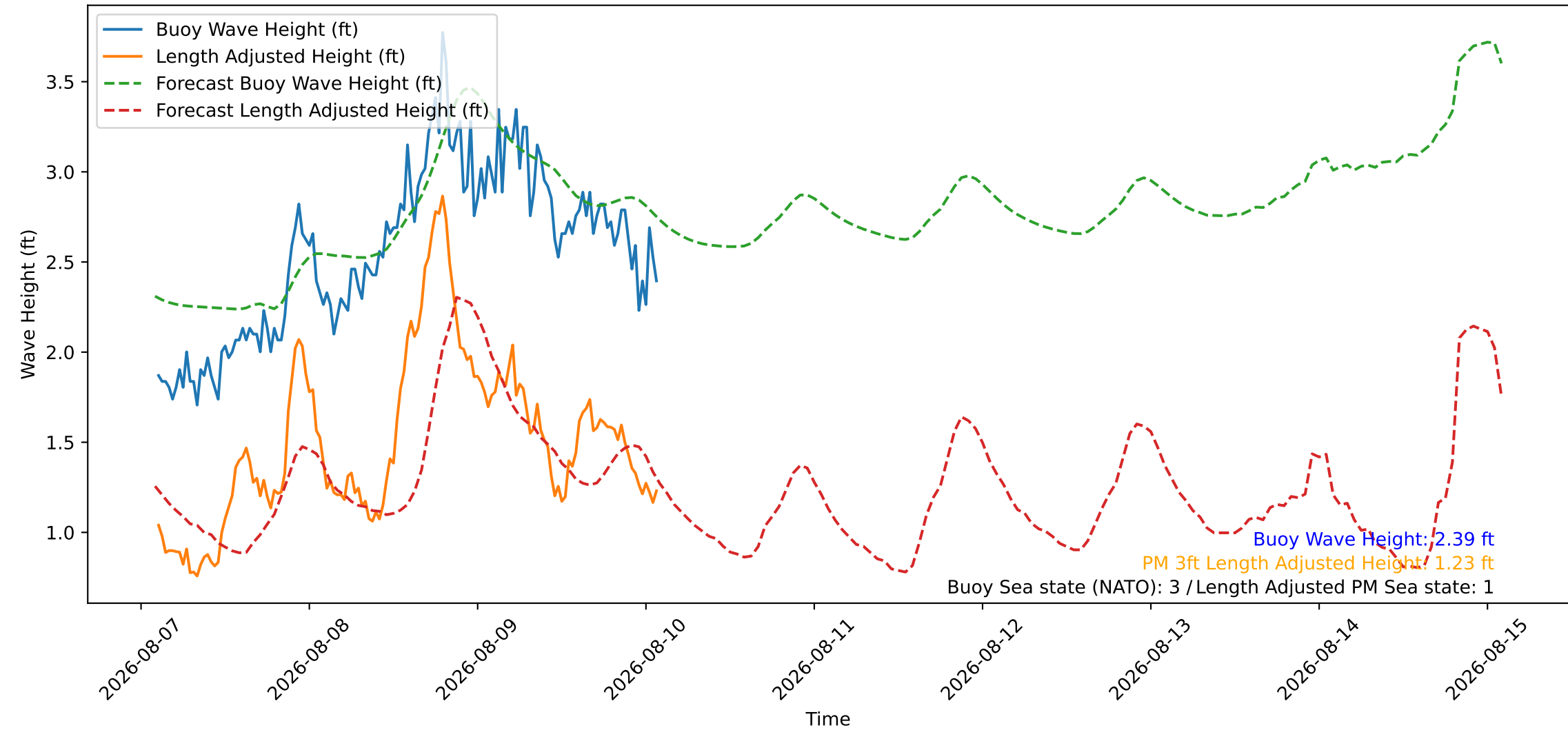
Wave Heights over Time for Green Beach at 2026-08-10 02:21:11
