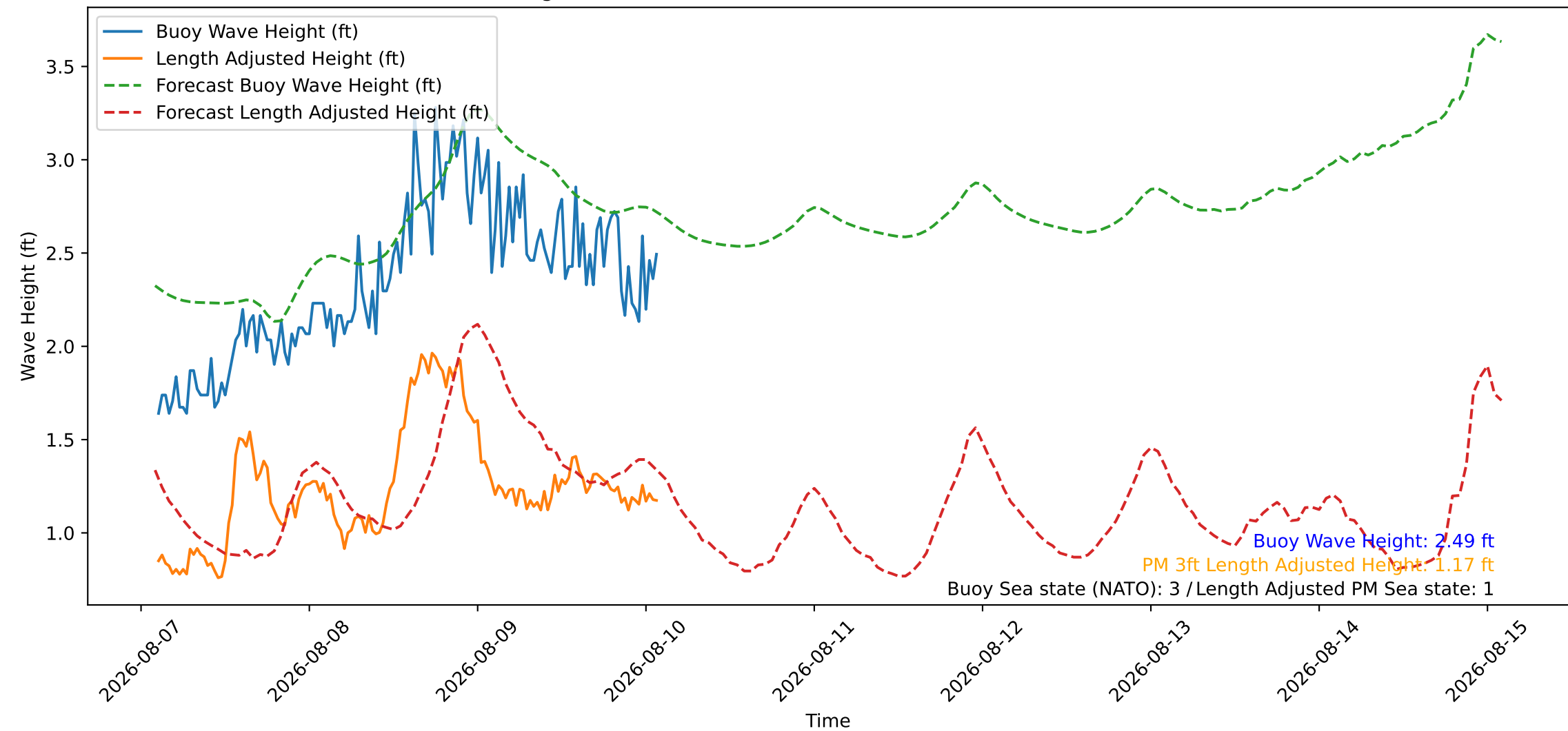
Wave Heights over Time for Oceanside Harbor at 2026-08-10 02:20:27
