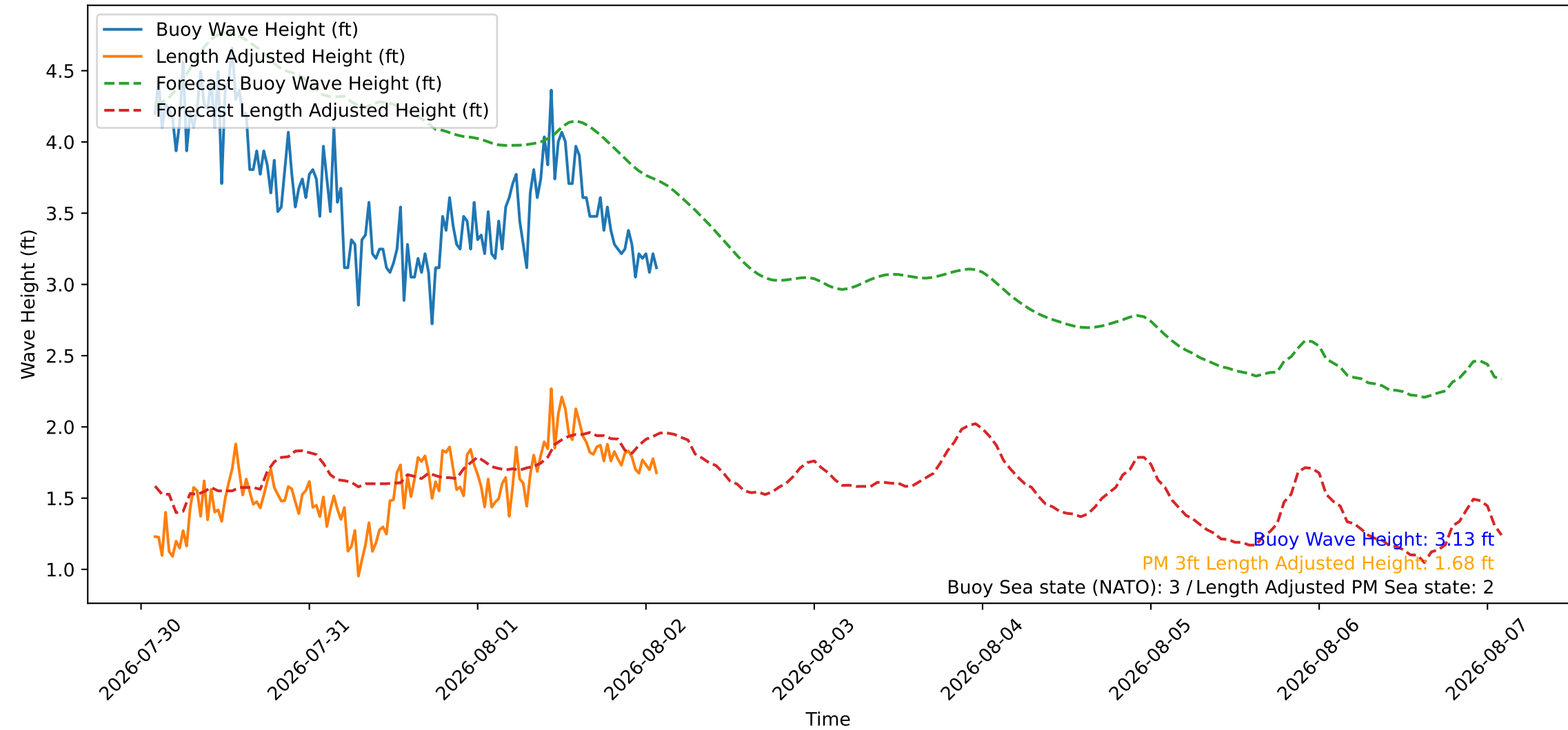
Wave Heights over Time for Oceanside Harbor at 2026-08-02 02:10:26
