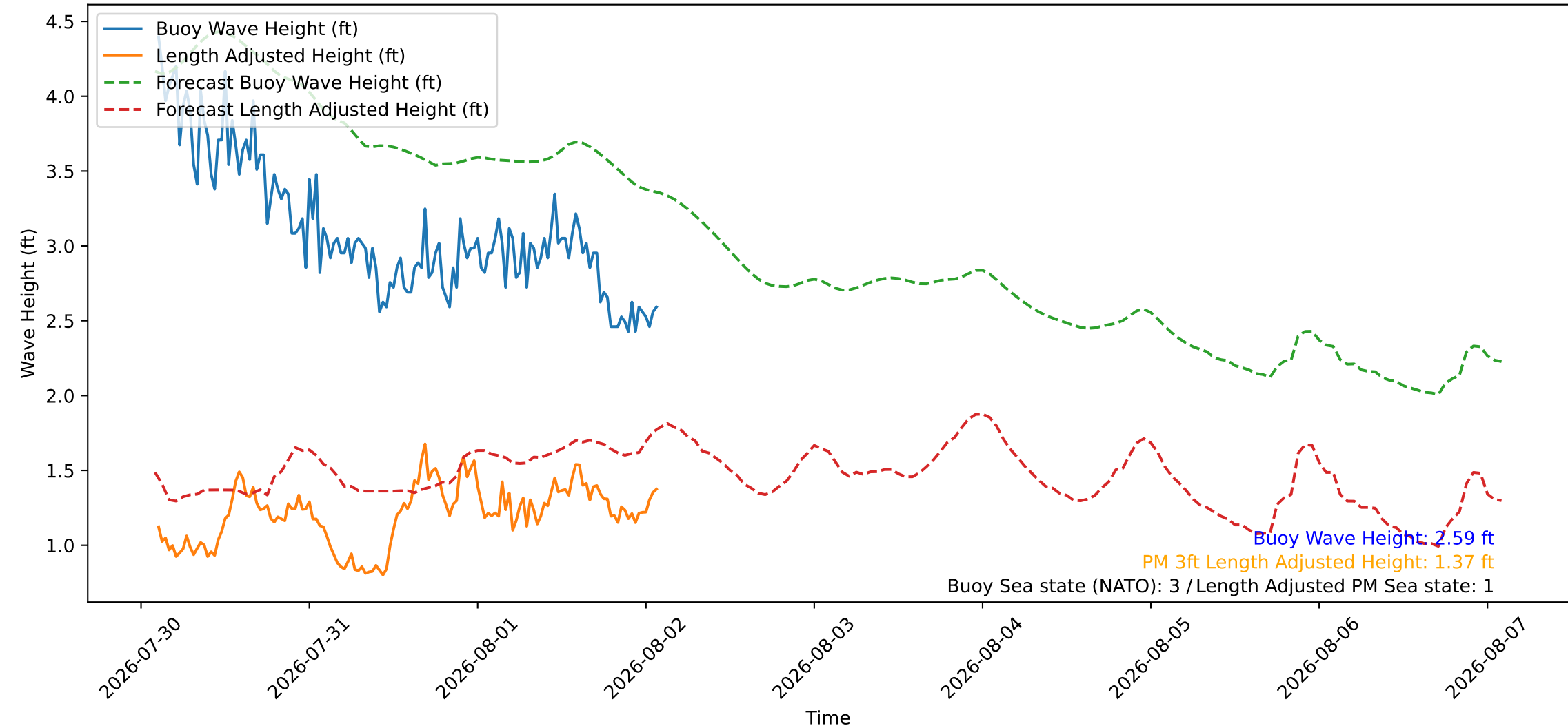
Wave Heights over Time for Red Beach at 2026-08-02 02:10:46
