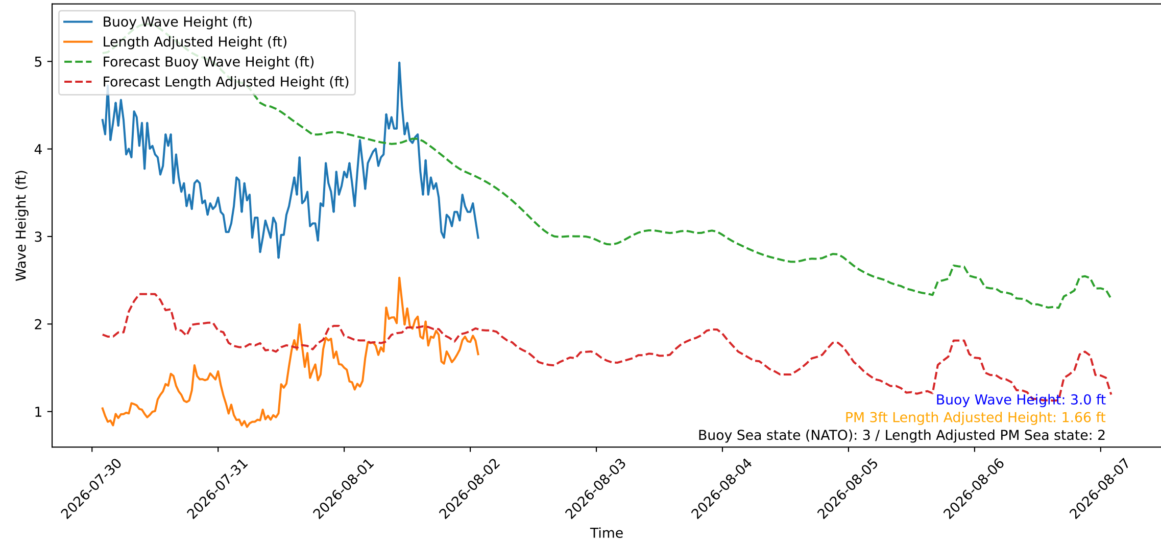
Wave Heights over Time for Green Beach at 2026-08-02 02:11:08
