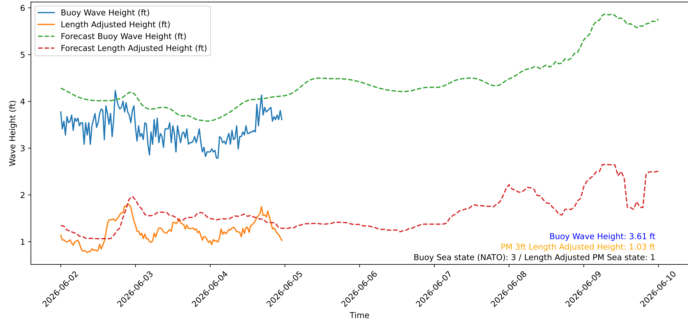
Wave Heights over Time for Green Beach at 2026-06-05 00:01:08
