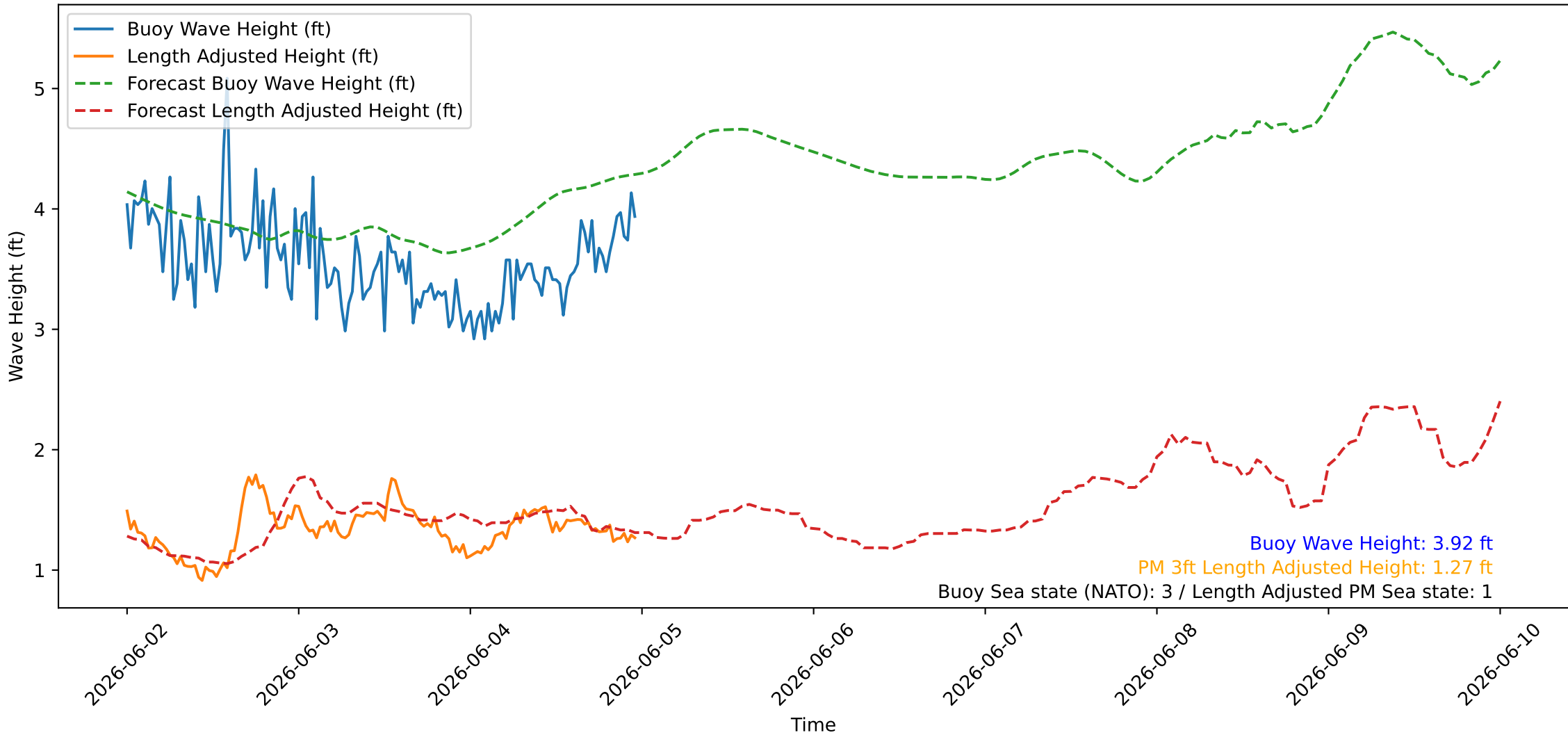
Wave Heights over Time for Oceanside Harbor at 2026-06-05 00:00:26
