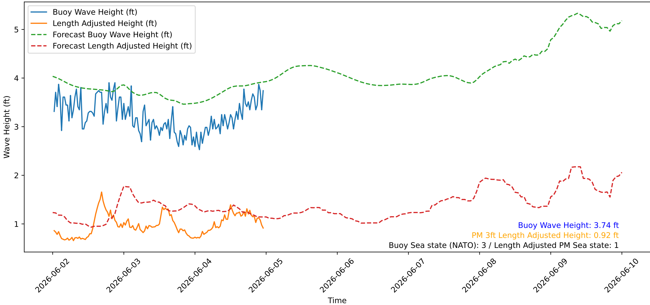
Wave Heights over Time for Red Beach at 2026-06-05 00:00:46
