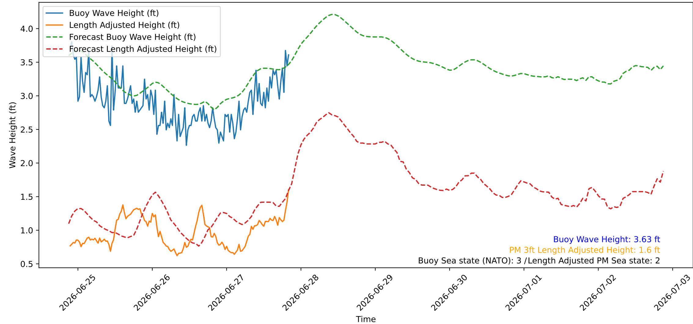
Wave Heights over Time for Red Beach at 2026-06-27 21:00:46
