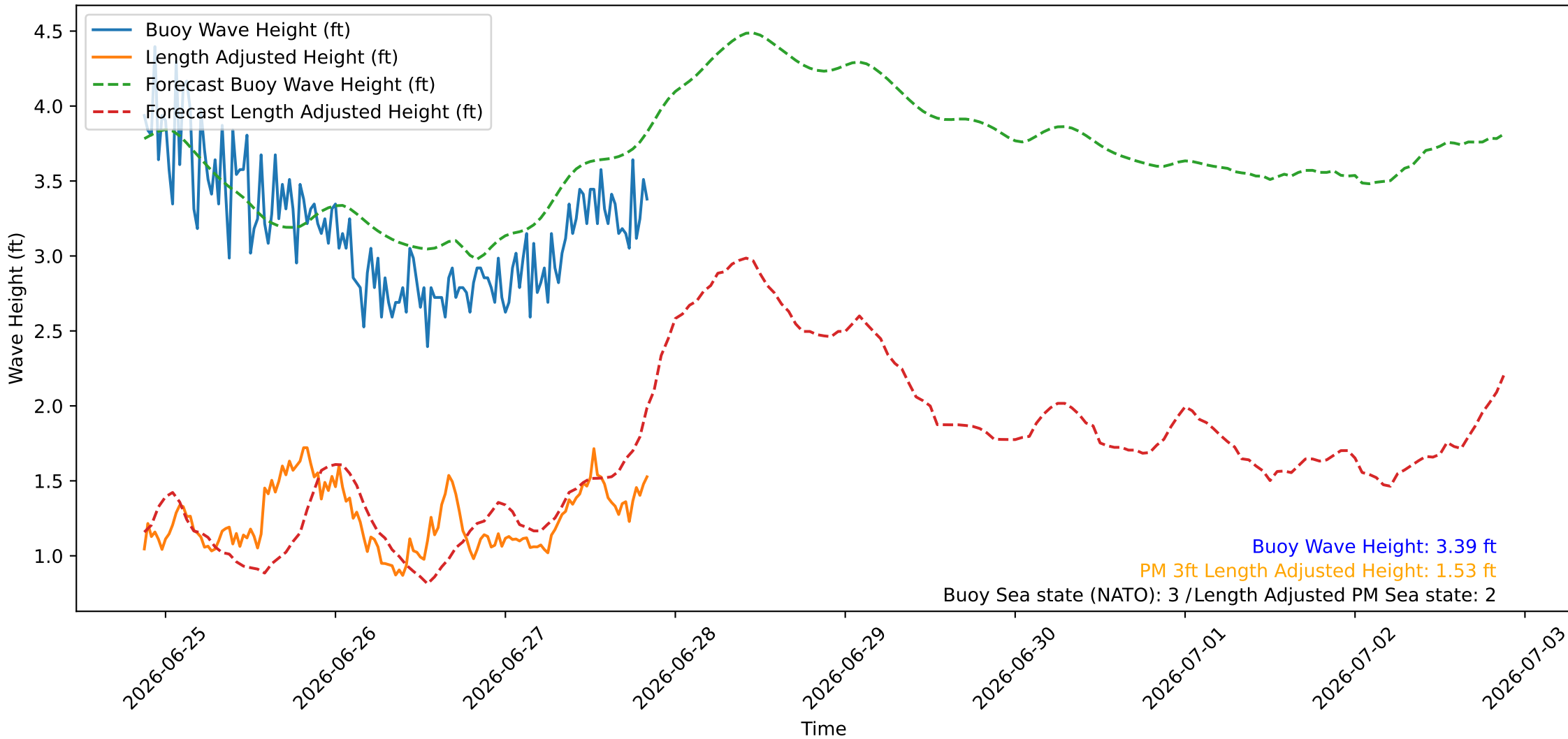
Wave Heights over Time for Oceanside Harbor at 2026-06-27 21:00:26
