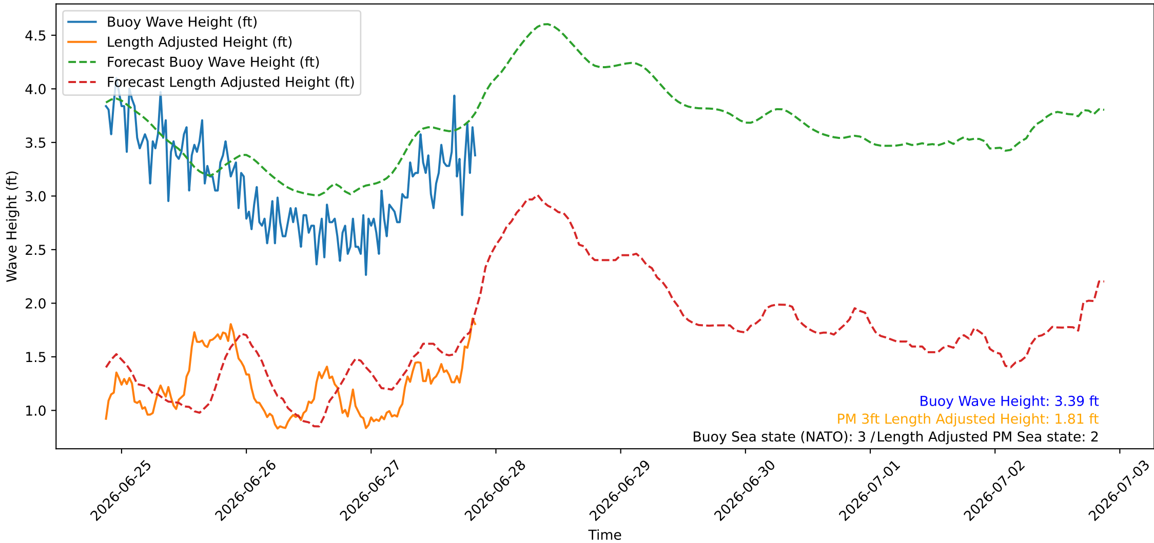
Wave Heights over Time for Green Beach at 2026-06-27 21:01:08
