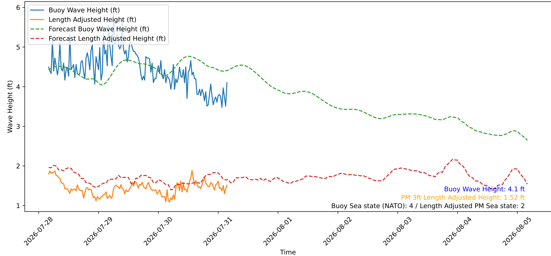
Wave Heights over Time for Oceanside Harbor at 2026-07-31 04:10:26
