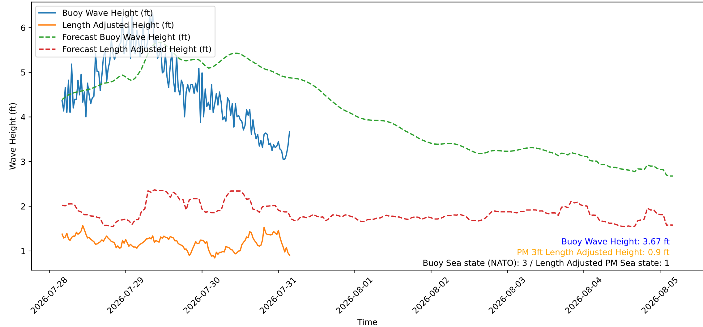
Wave Heights over Time for Green Beach at 2026-07-31 04:11:08
