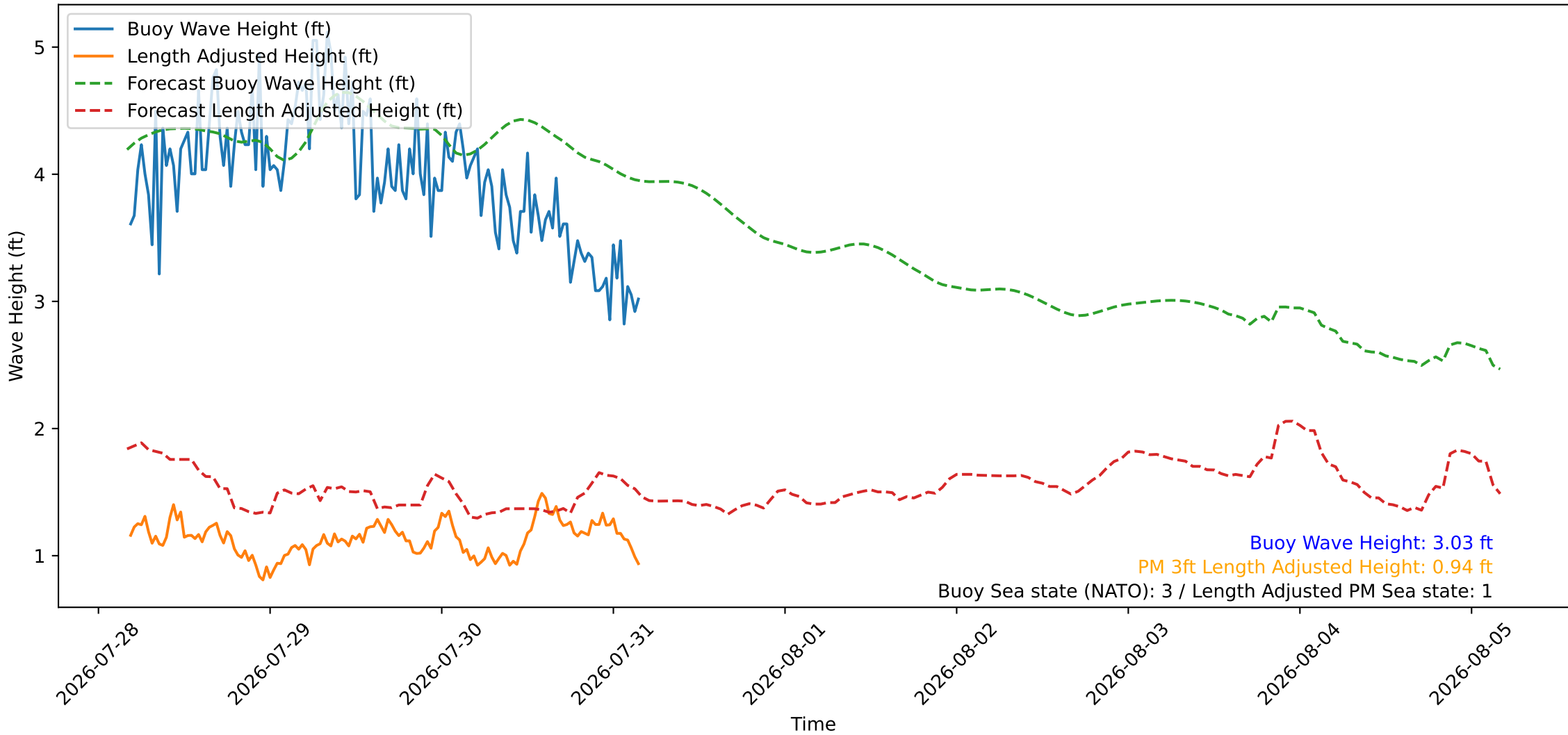
Wave Heights over Time for Red Beach at 2026-07-31 04:10:46
