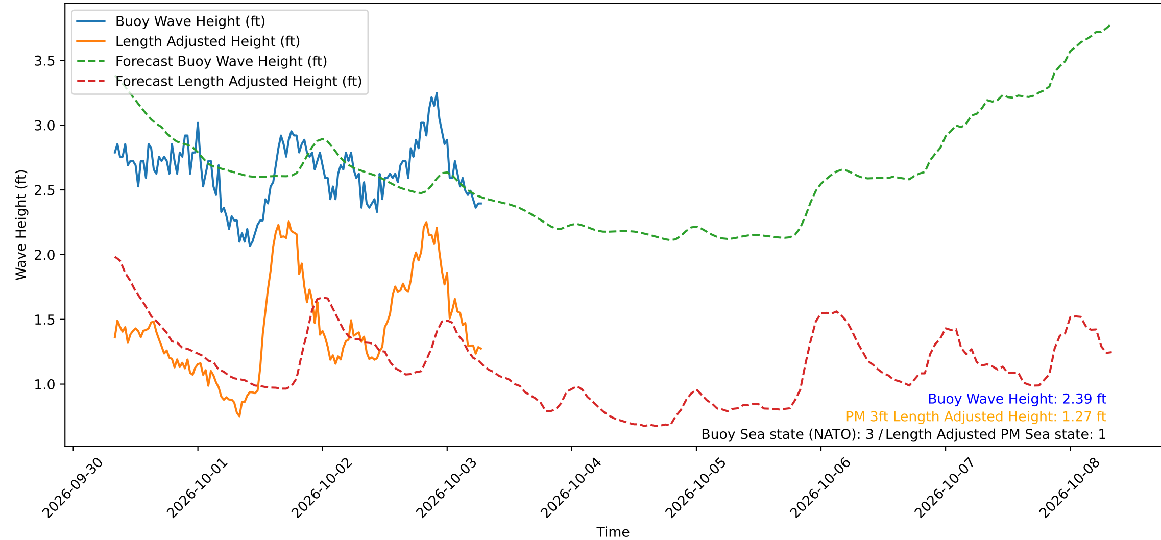
Wave Heights over Time for Red Beach at 2026-10-03 07:30:49
