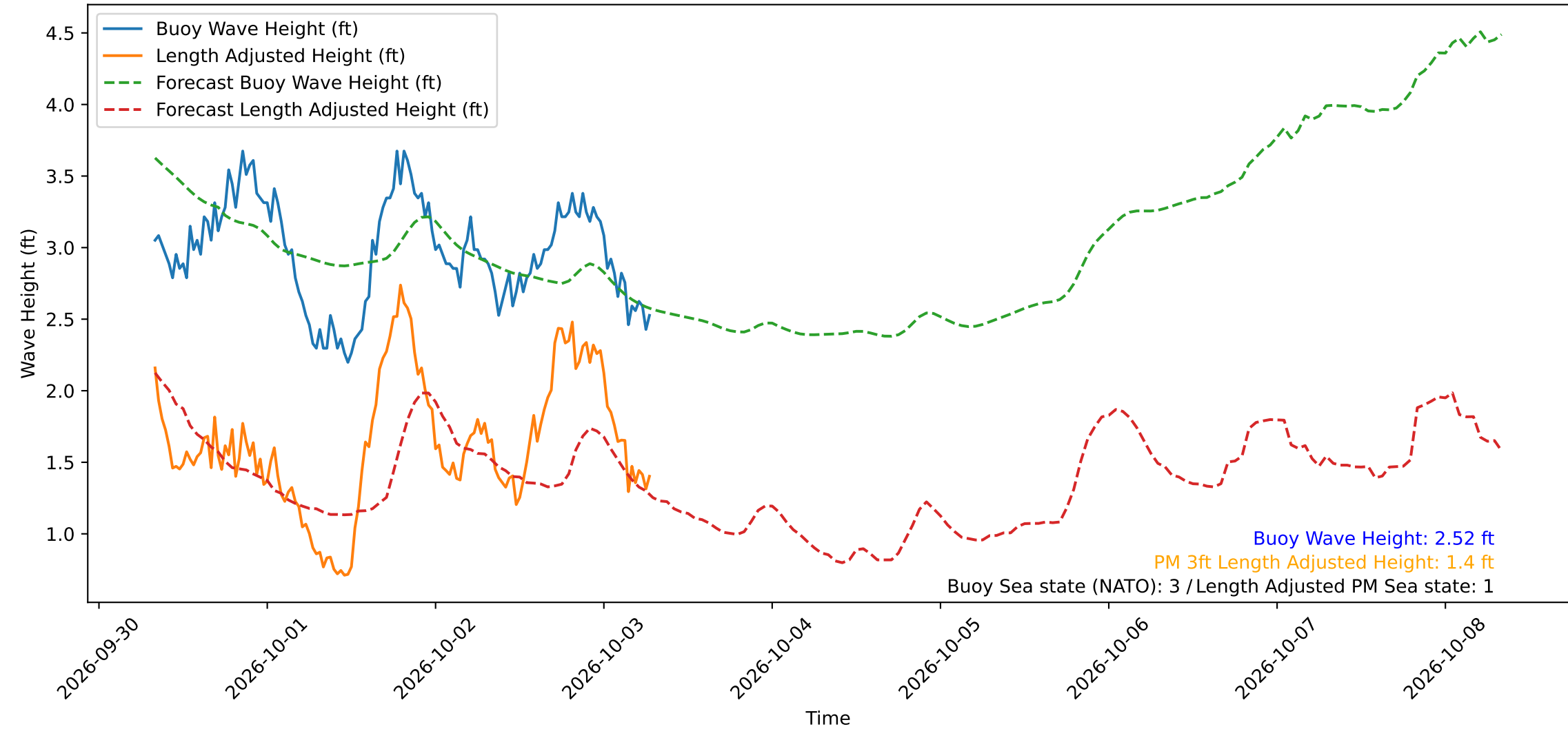
Wave Heights over Time for Green Beach at 2026-10-03 07:31:11
