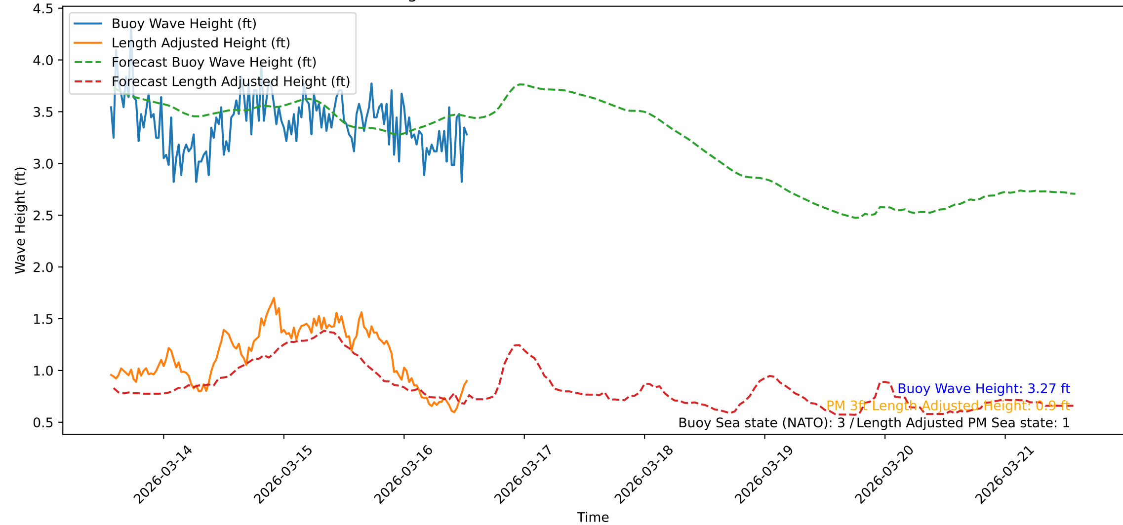
Wave Heights over Time for Green Beach at 2026-03-16 13:31:44
