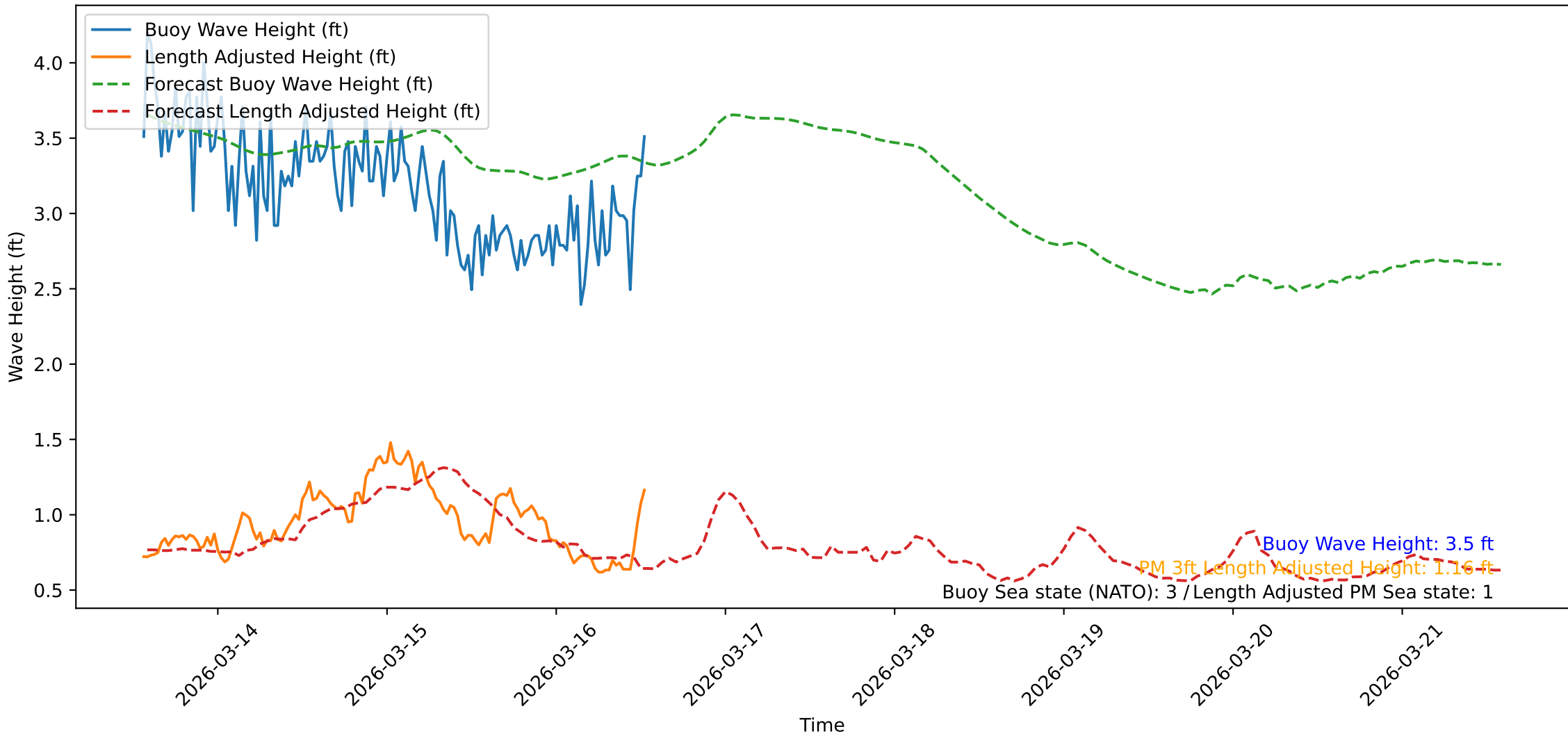
Wave Heights over Time for Oceanside Harbor at 2026-03-16 13:30:45
