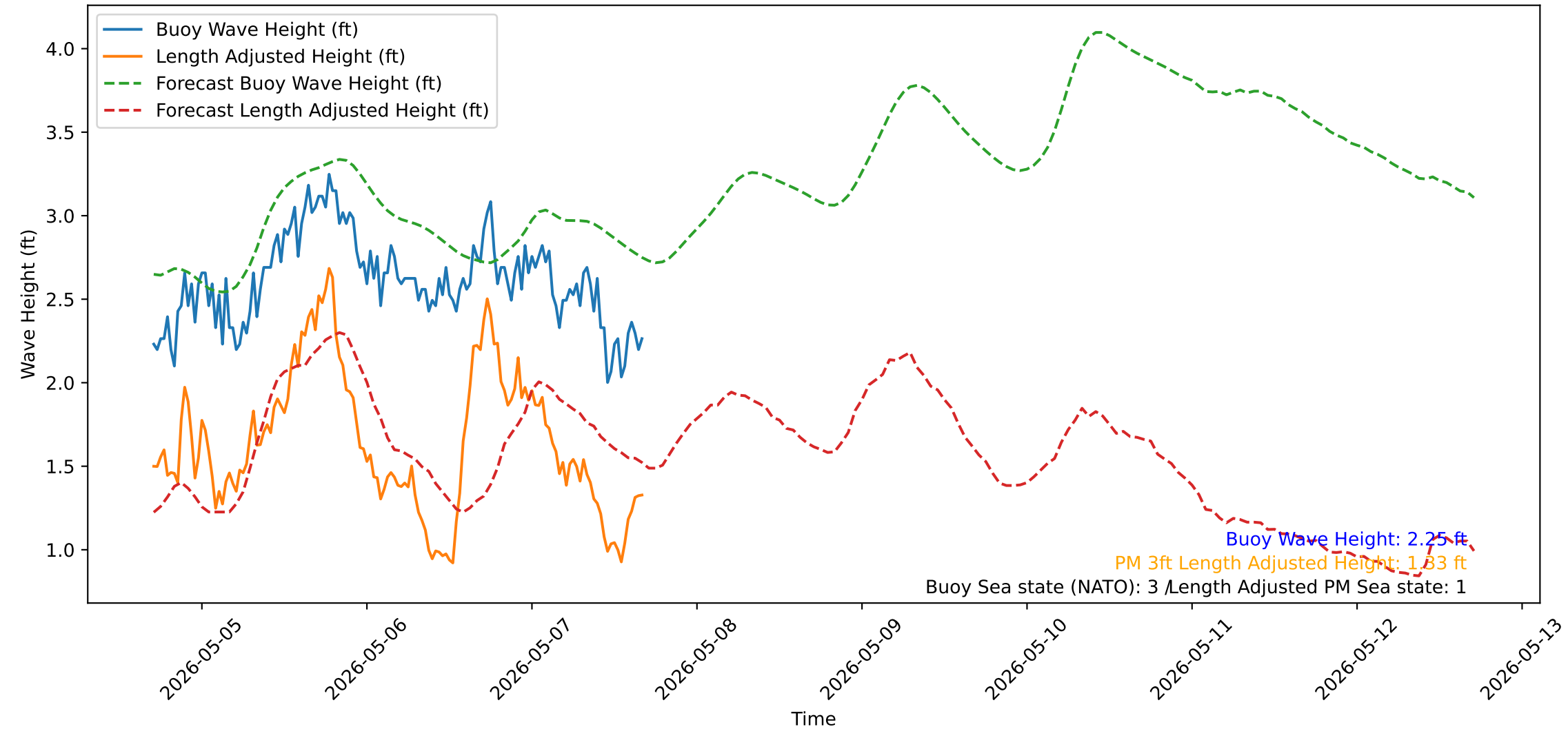
Wave Heights over Time for Oceanside Harbor at 2026-05-07 16:50:31
