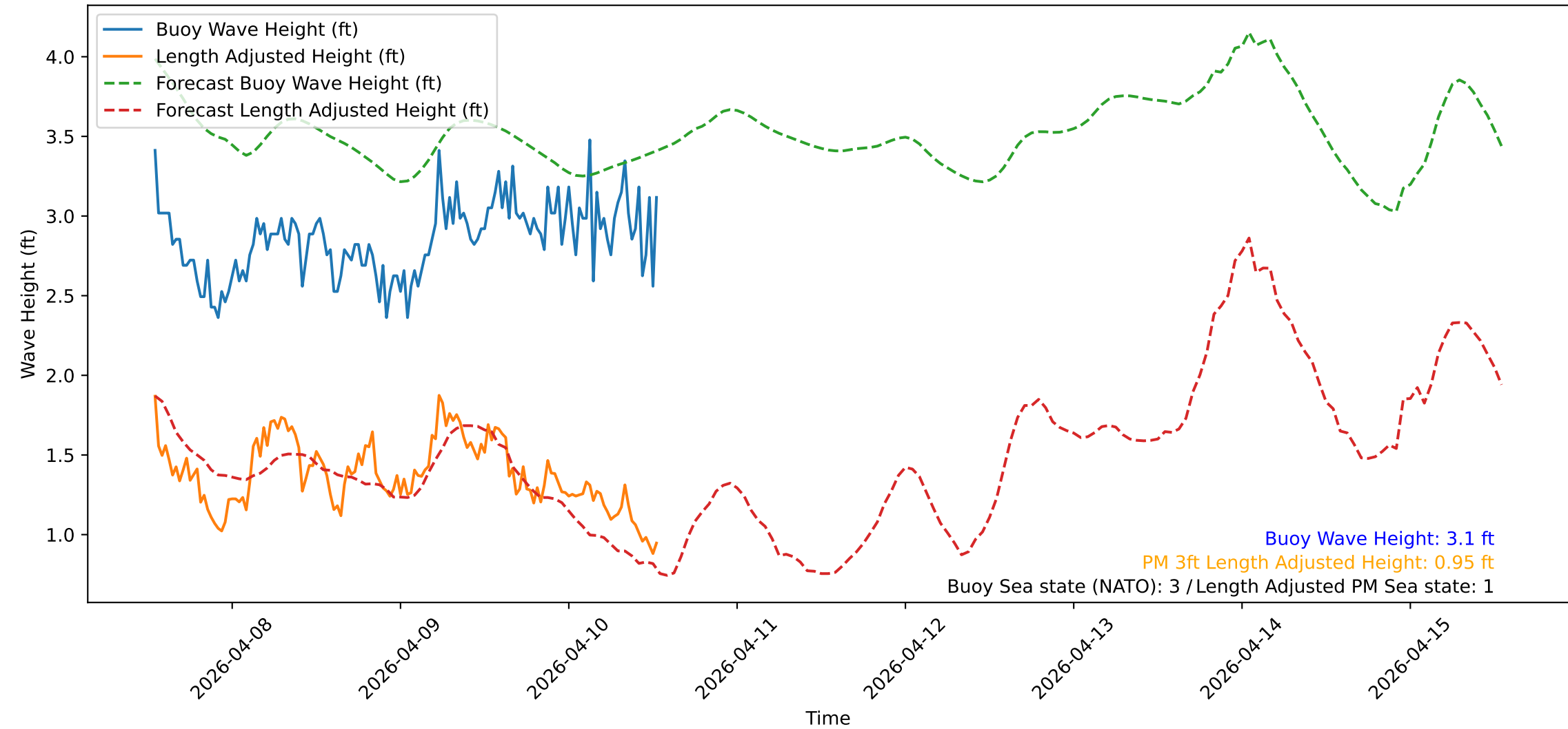
Wave Heights over Time for Green Beach at 2026-04-10 13:11:13
