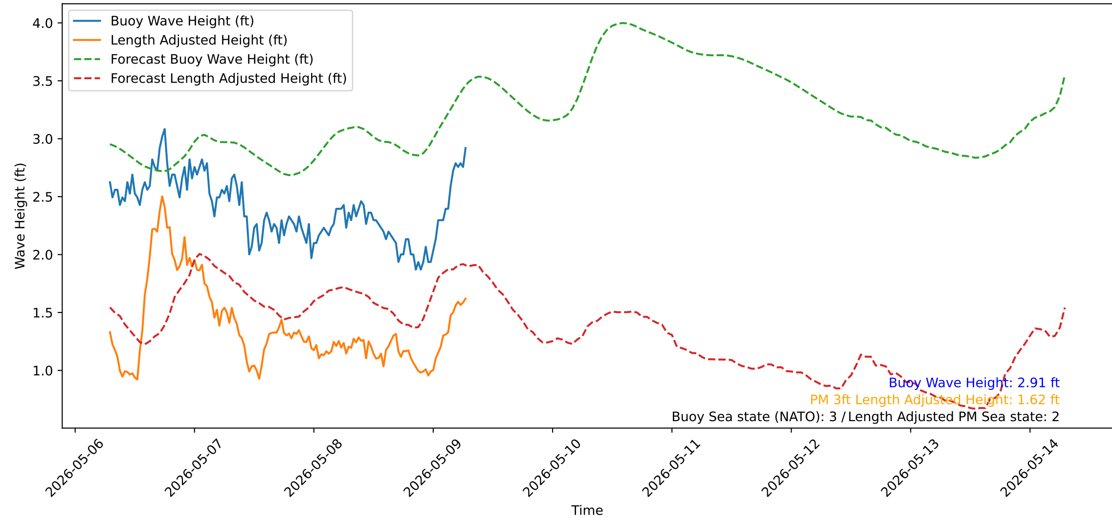
Wave Heights over Time for Oceanside Harbor at 2026-05-09 07:10:33
