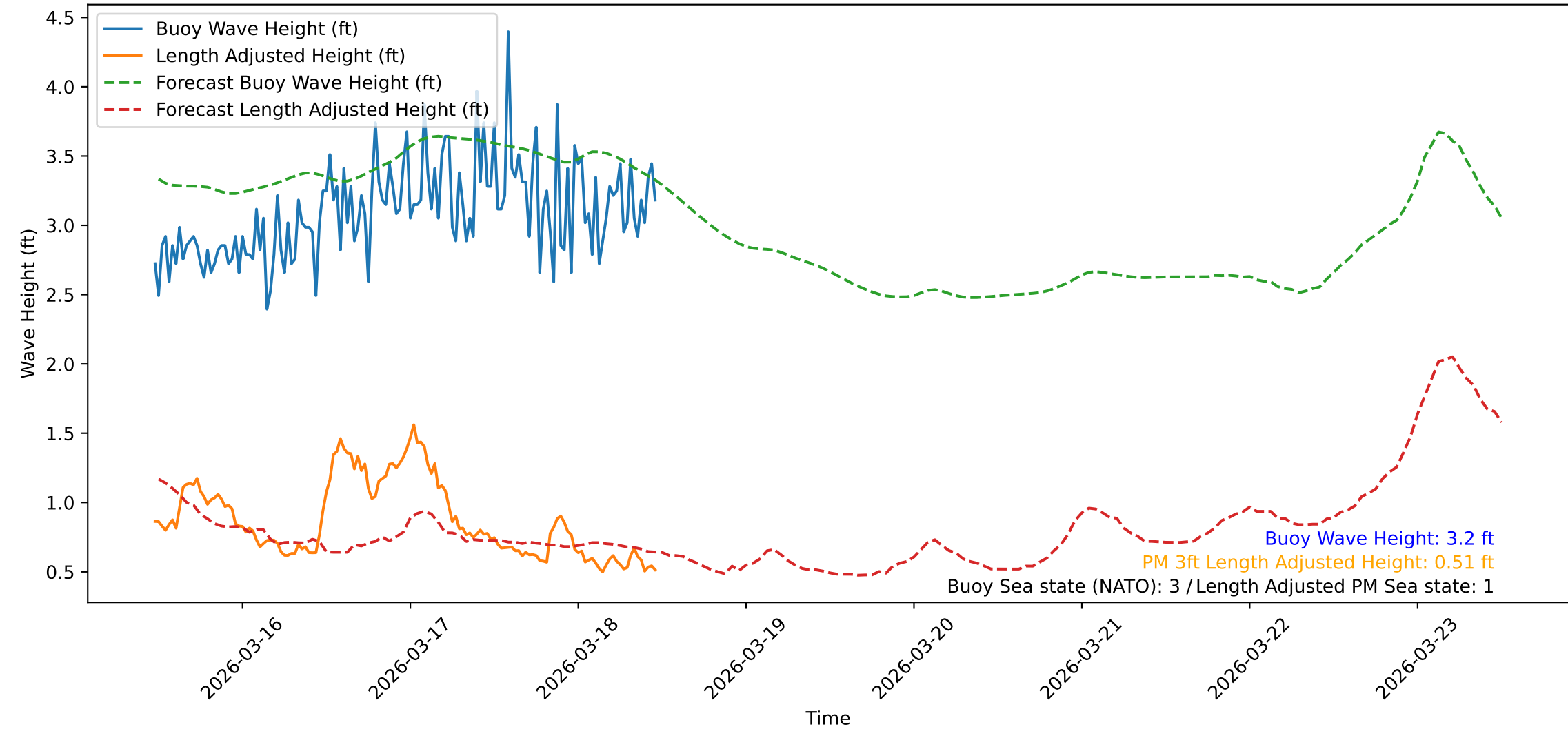
Wave Heights over Time for Oceanside Harbor at 2026-03-18 11:36:24
