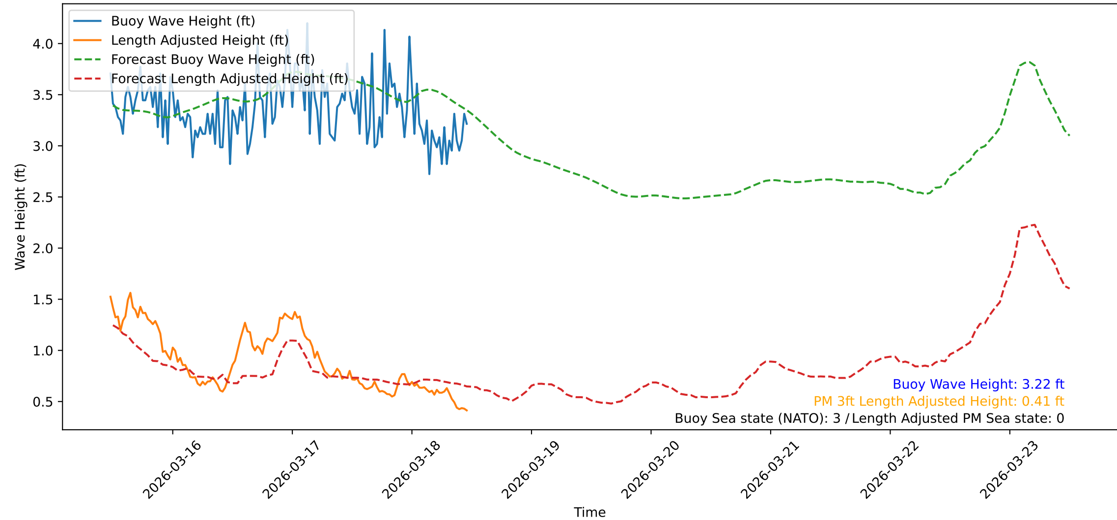
Wave Heights over Time for Green Beach at 2026-03-18 11:37:02
