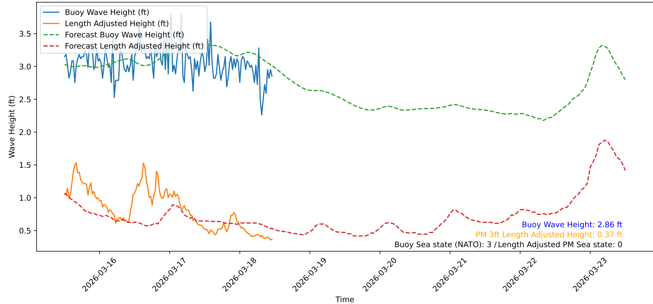
Wave Heights over Time for Red Beach at 2026-03-18 11:36:40
