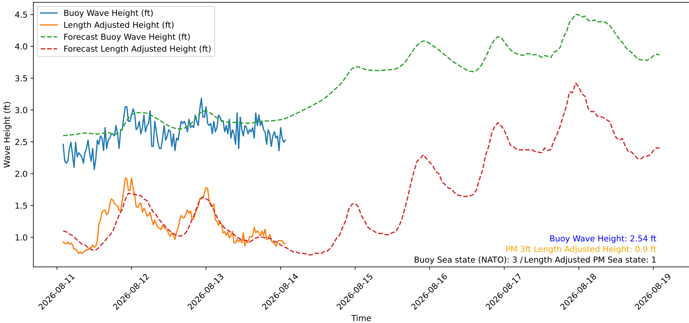
Wave Heights over Time for Oceanside Harbor at 2026-08-14 02:10:26
