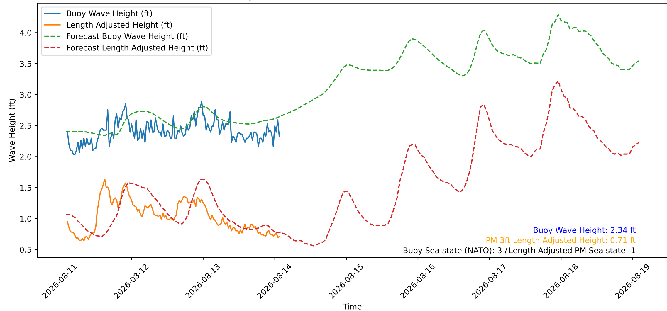
Wave Heights over Time for Red Beach at 2026-08-14 02:10:46
