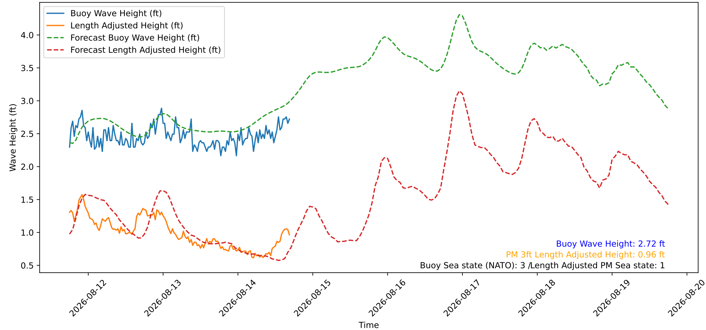
Wave Heights over Time for Red Beach at 2026-08-14 17:40:46
