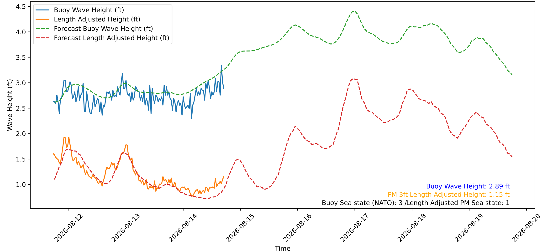
Wave Heights over Time for Oceanside Harbor at 2026-08-14 17:40:27
