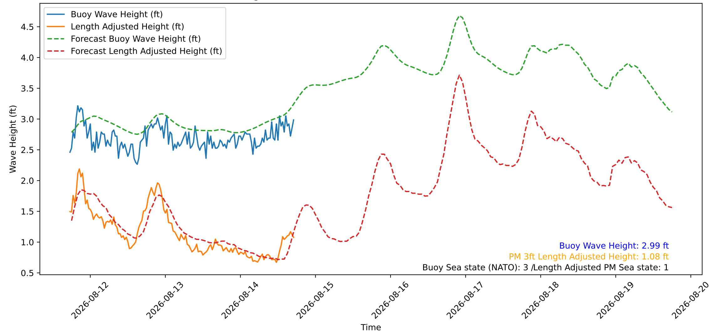
Wave Heights over Time for Green Beach at 2026-08-14 17:41:08
