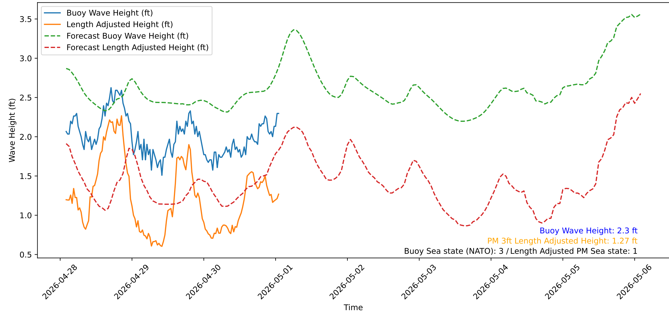
Wave Heights over Time for Red Beach at 2026-05-01 01:40:51
