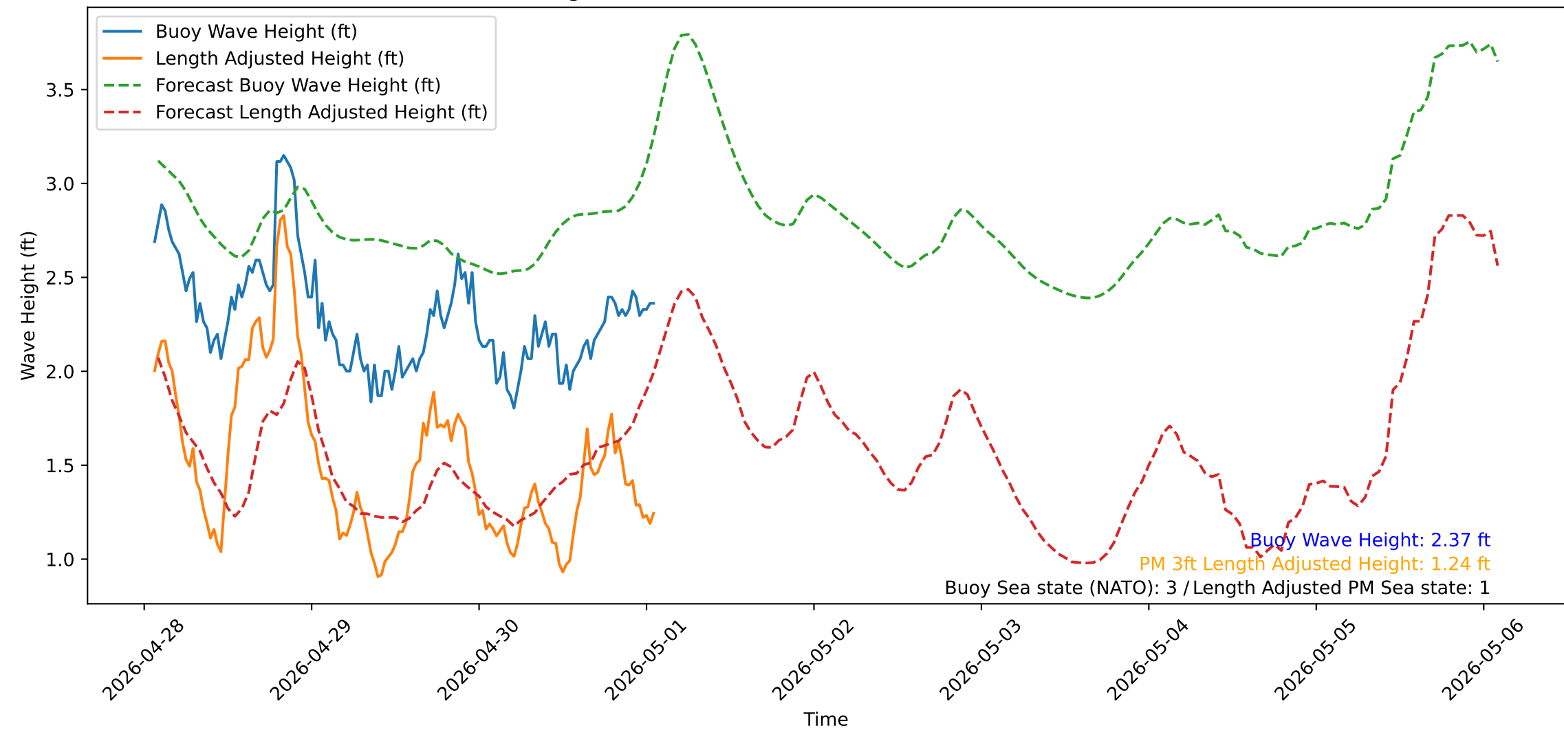
Wave Heights over Time for Green Beach at 2026-05-01 01:41:13
