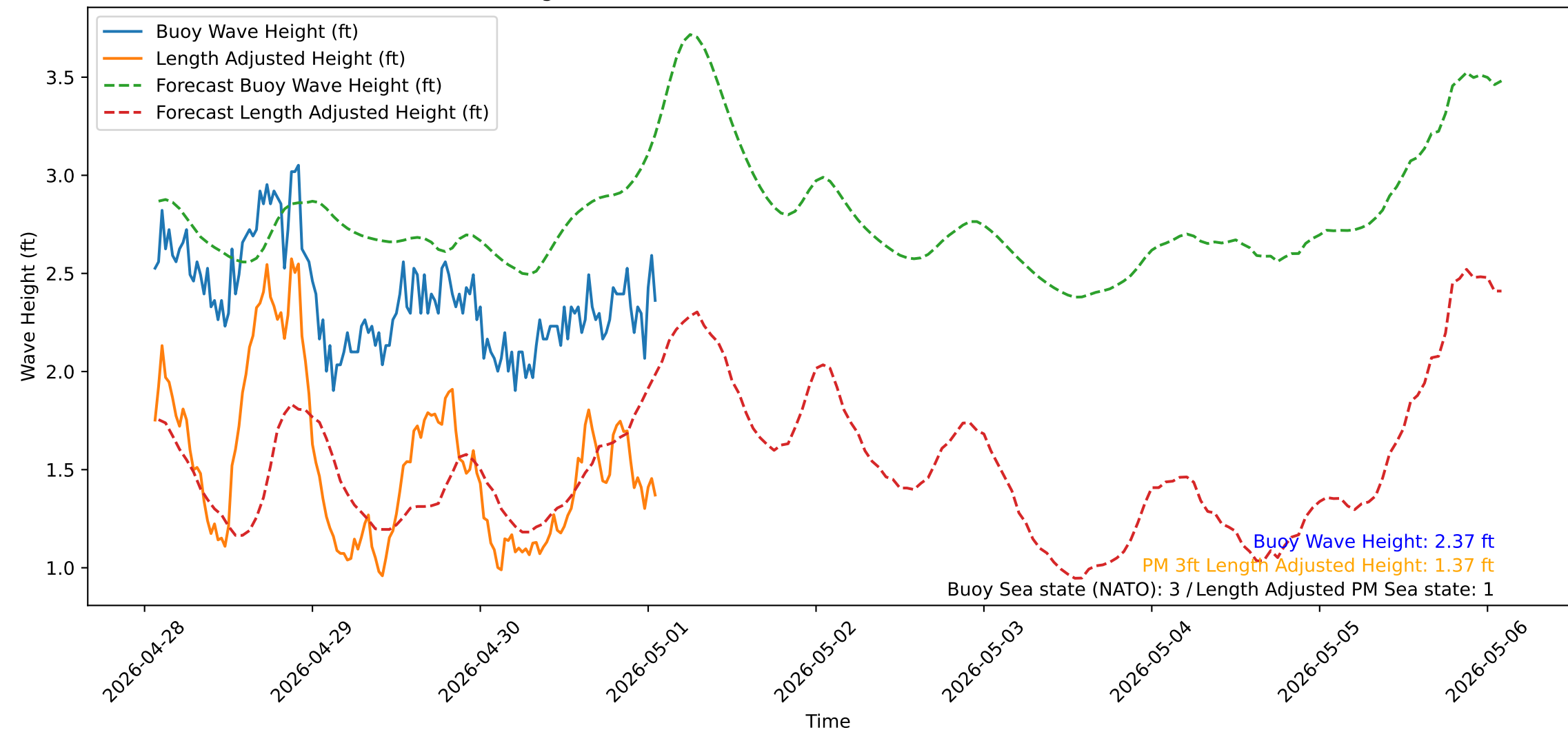
Wave Heights over Time for Oceanside Harbor at 2026-05-01 01:40:31
