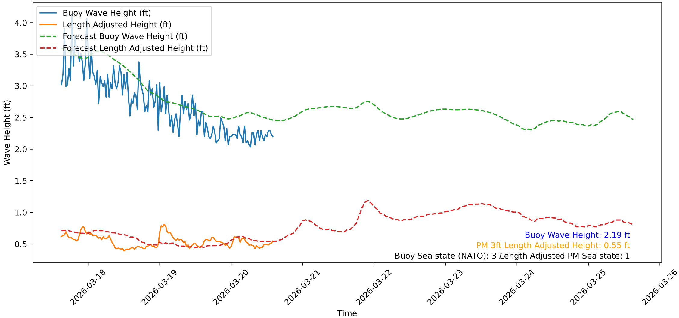
Wave Heights over Time for Green Beach at 2026-03-20 15:01:10
