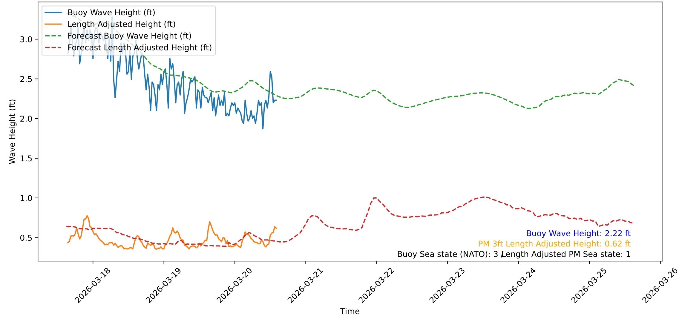
Wave Heights over Time for Red Beach at 2026-03-20 15:00:48
