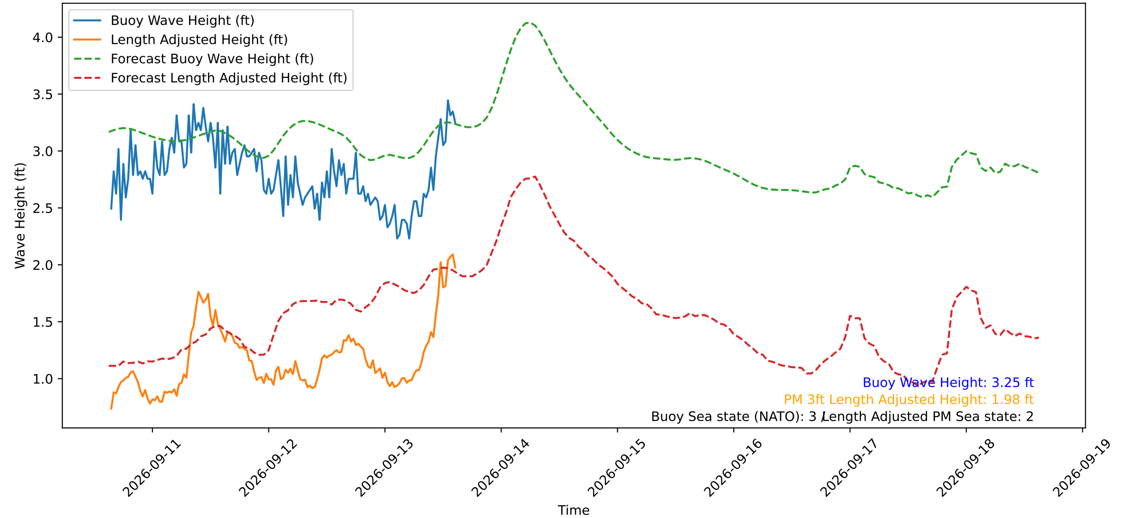
Wave Heights over Time for Red Beach at 2026-09-13 15:10:49
