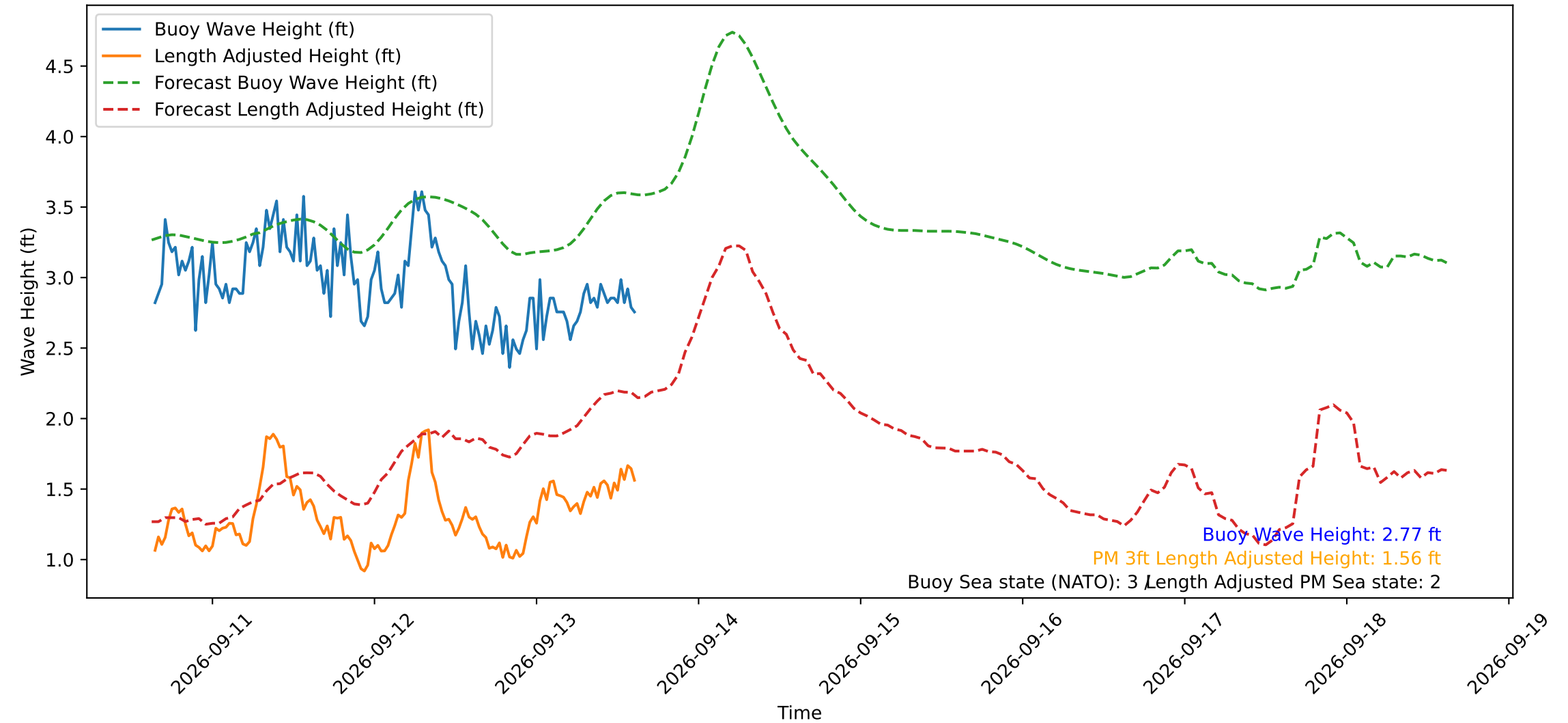
Wave Heights over Time for Green Beach at 2026-09-13 15:11:11
