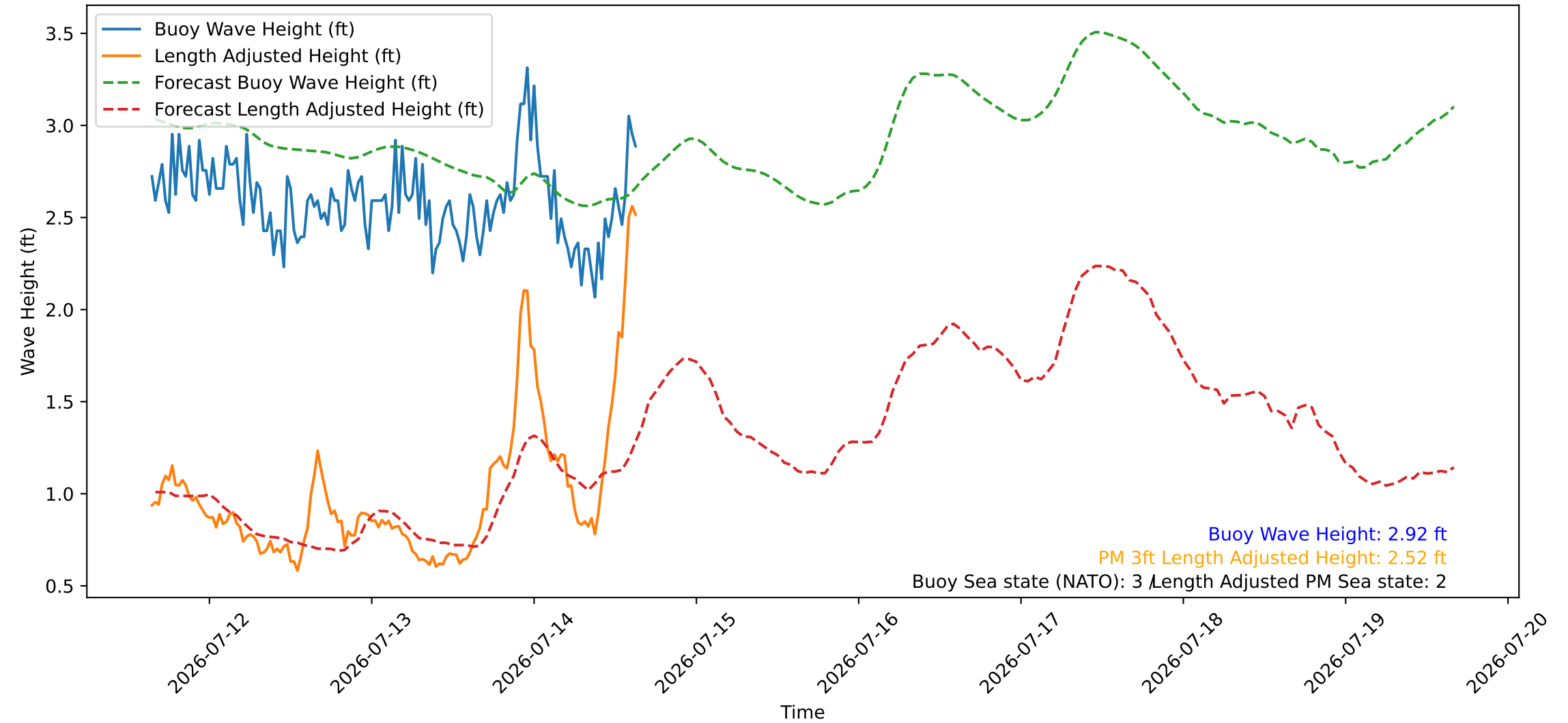
Wave Heights over Time for Green Beach at 2026-07-14 15:41:10
