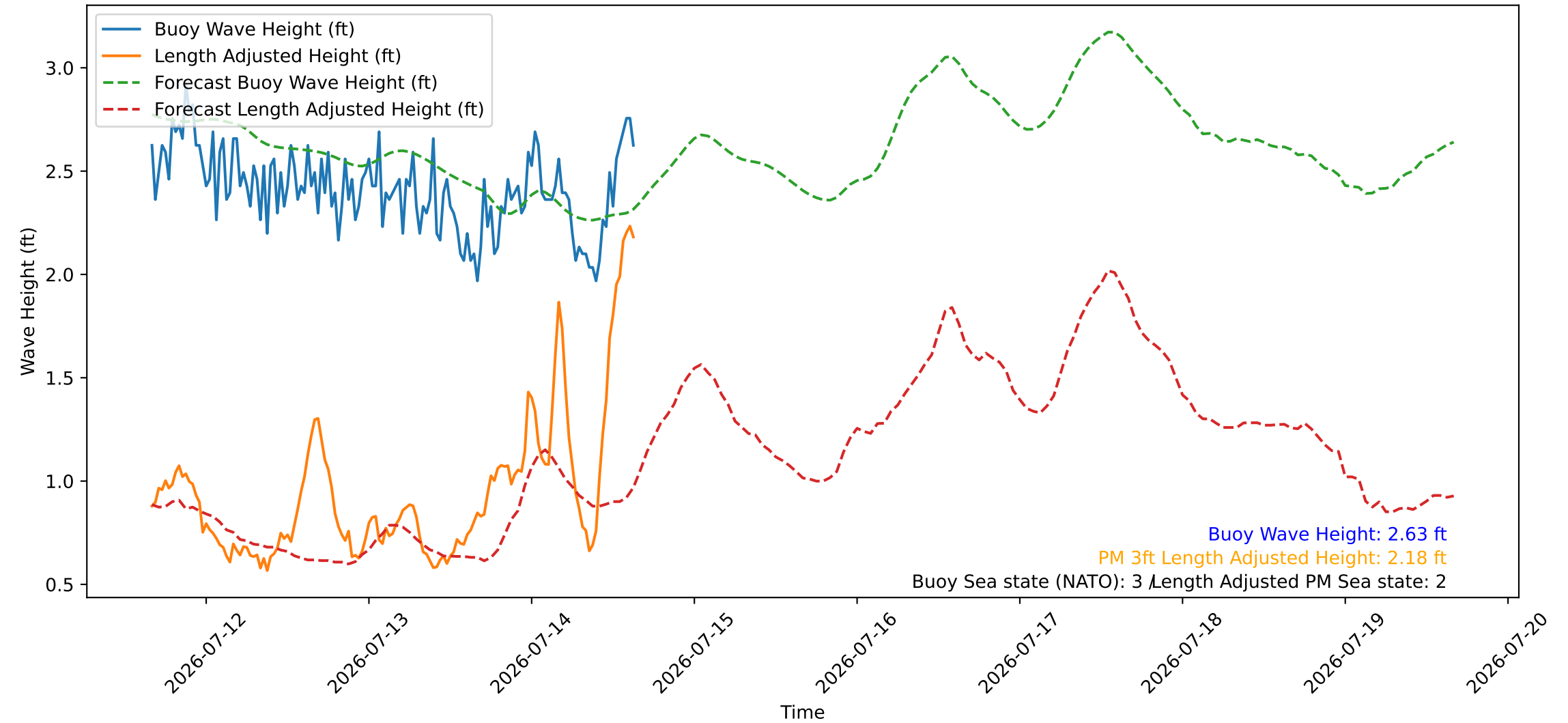
Wave Heights over Time for Red Beach at 2026-07-14 15:40:46
