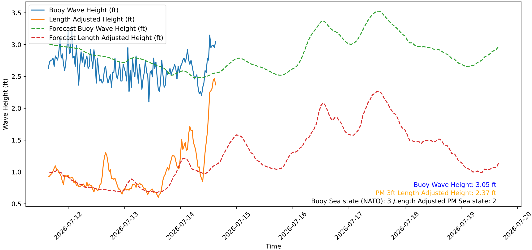
Wave Heights over Time for Oceanside Harbor at 2026-07-14 15:40:27
