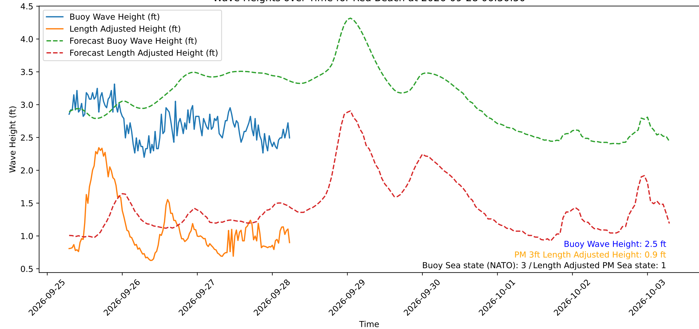
Wave Heights over Time for Red Beach at 2026-09-28 06:30:50
