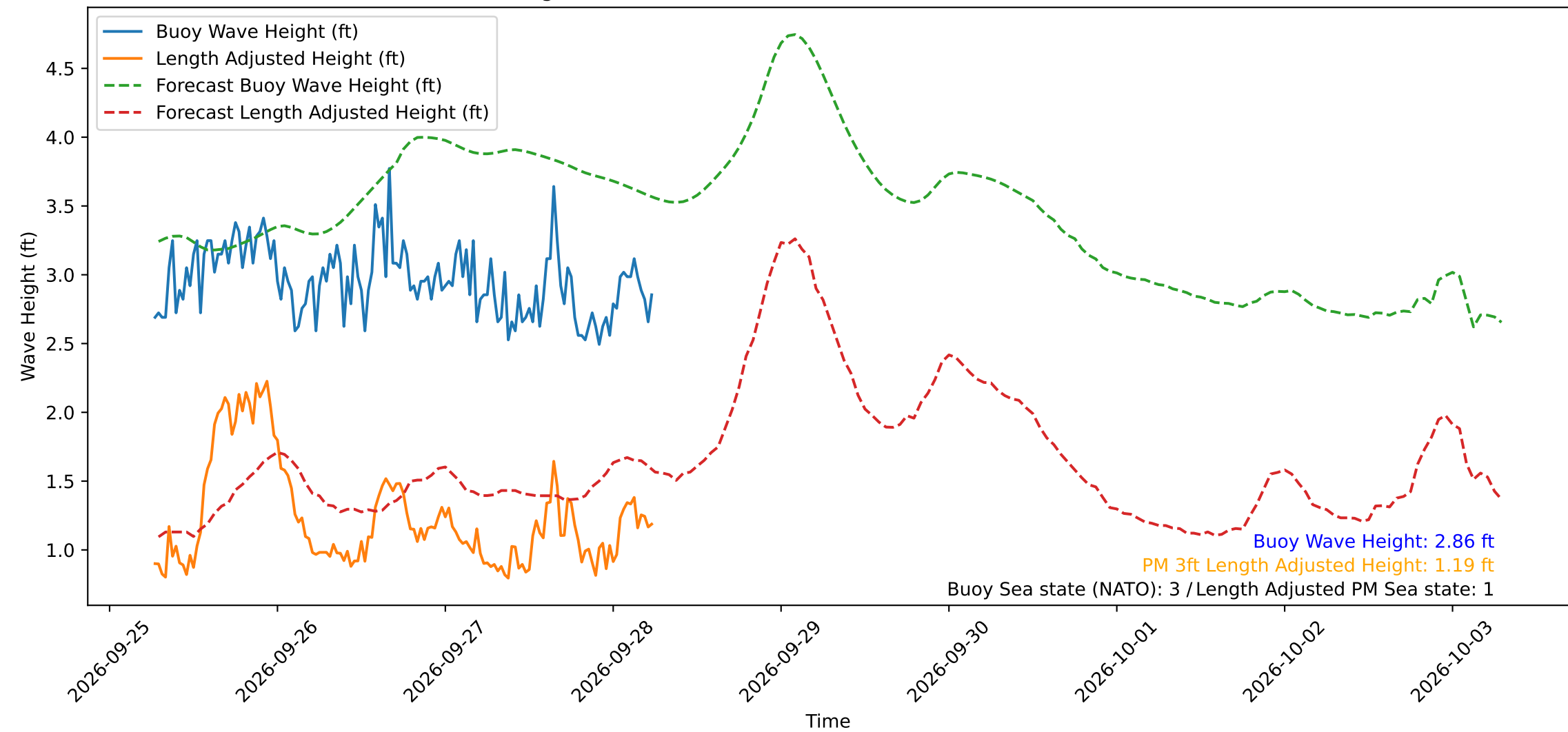
Wave Heights over Time for Oceanside Harbor at 2026-09-28 06:30:30
