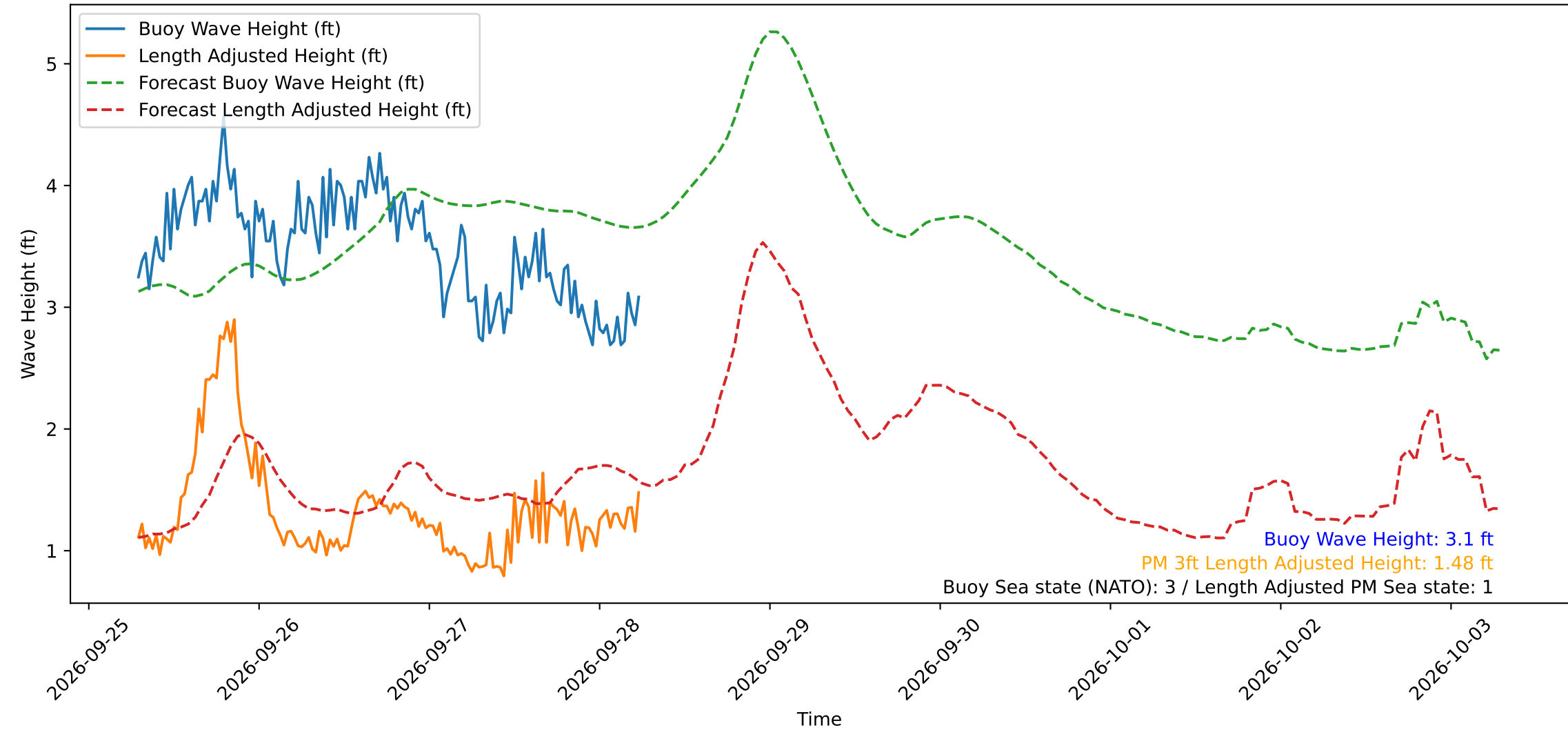
Wave Heights over Time for Green Beach at 2026-09-28 06:31:12
