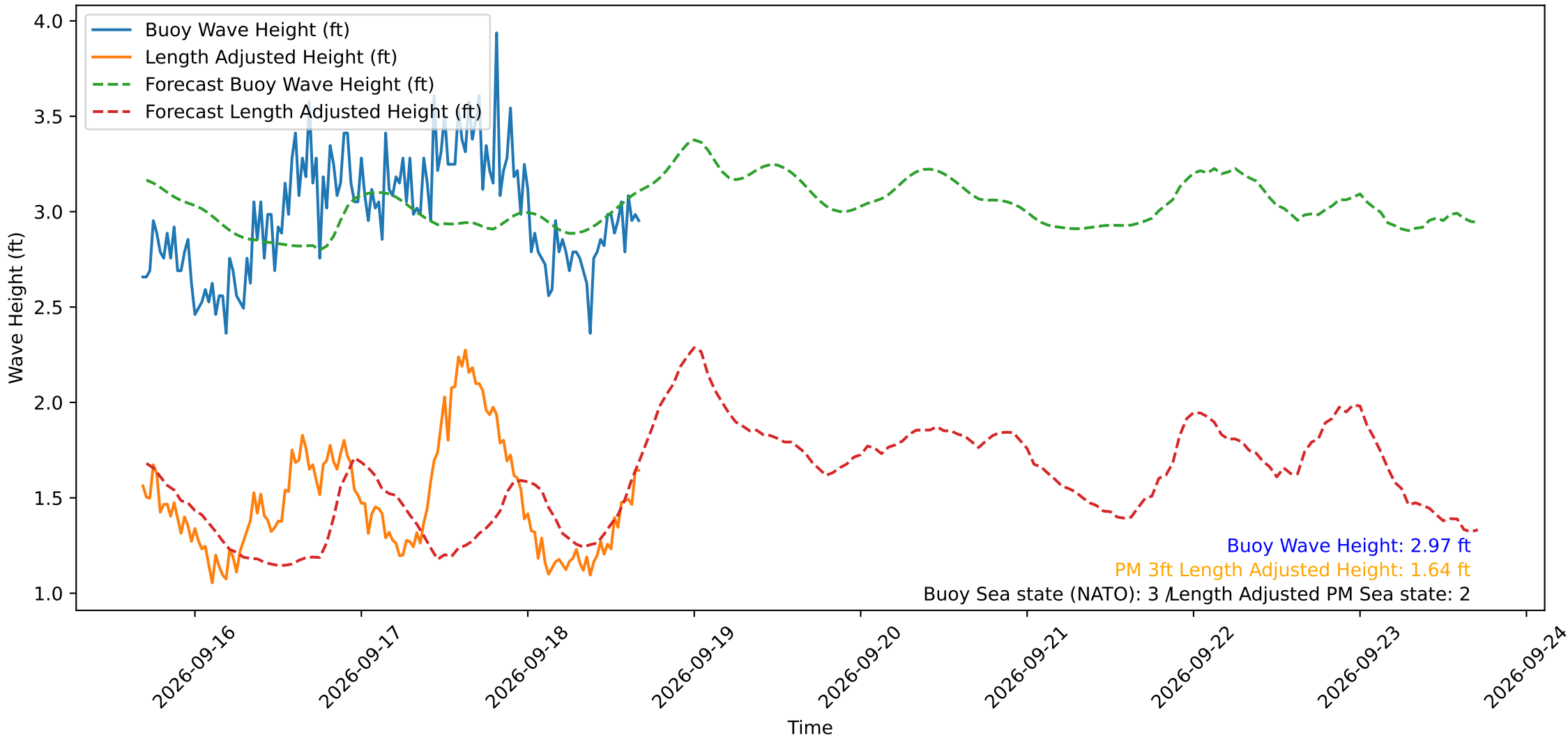
Wave Heights over Time for Oceanside Harbor at 2026-09-18 16:30:31
