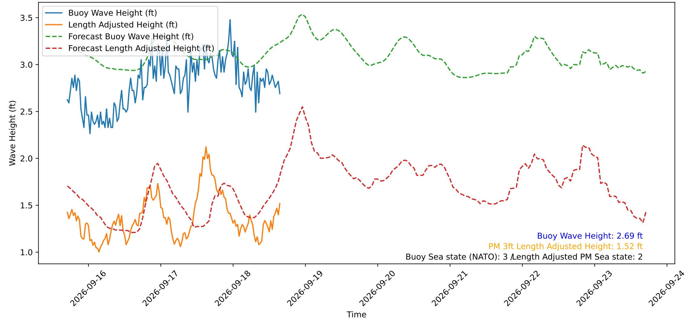
Wave Heights over Time for Green Beach at 2026-09-18 16:31:16
