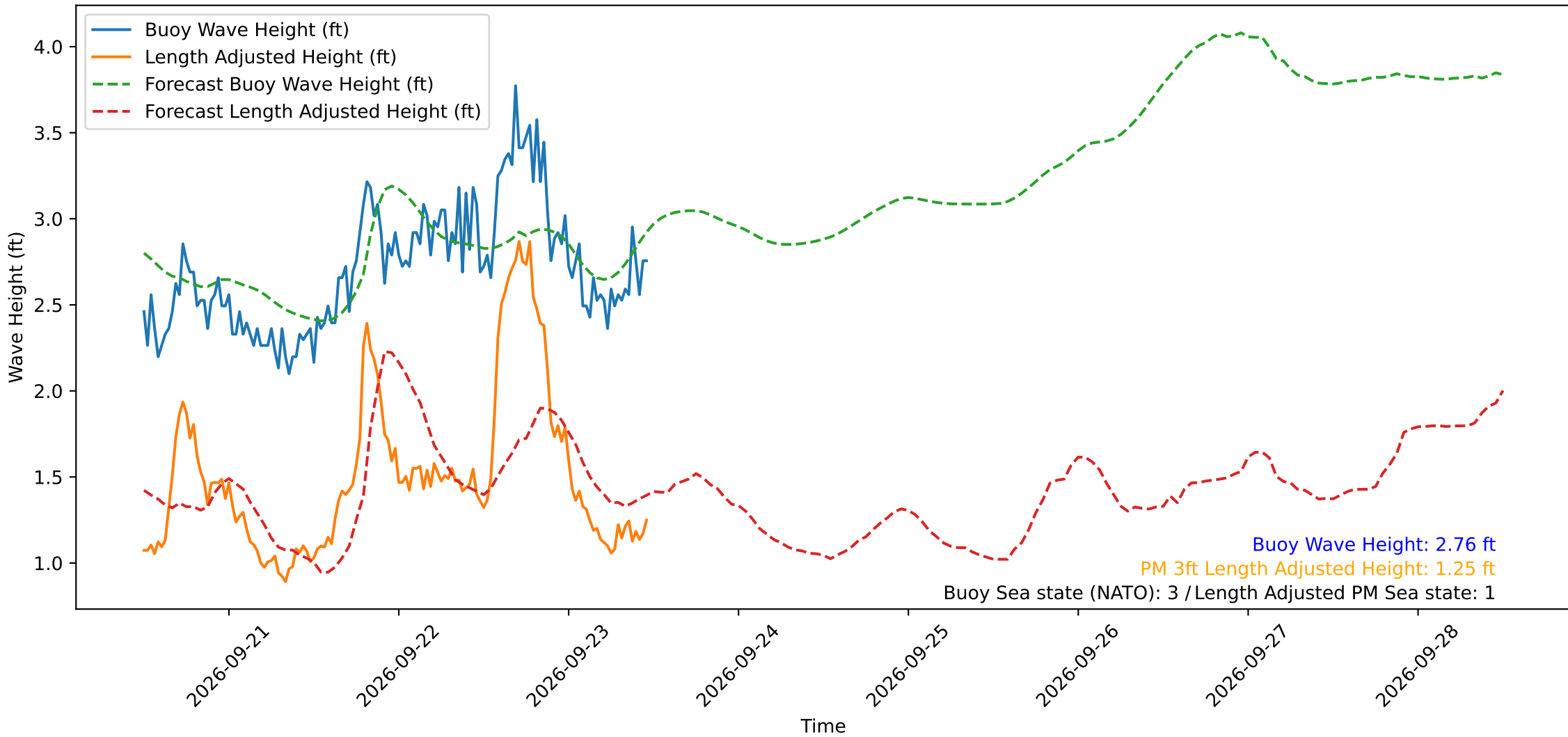
Wave Heights over Time for Oceanside Harbor at 2026-09-23 11:50:29
