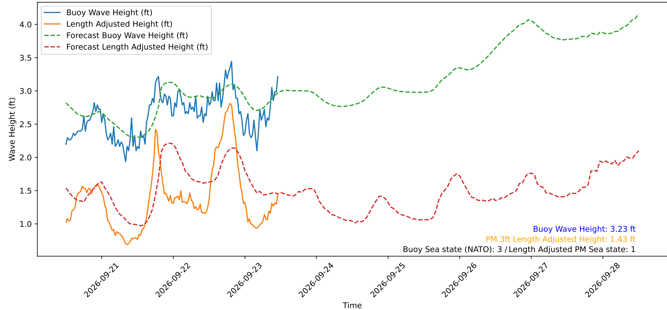
Wave Heights over Time for Green Beach at 2026-09-23 11:51:14
