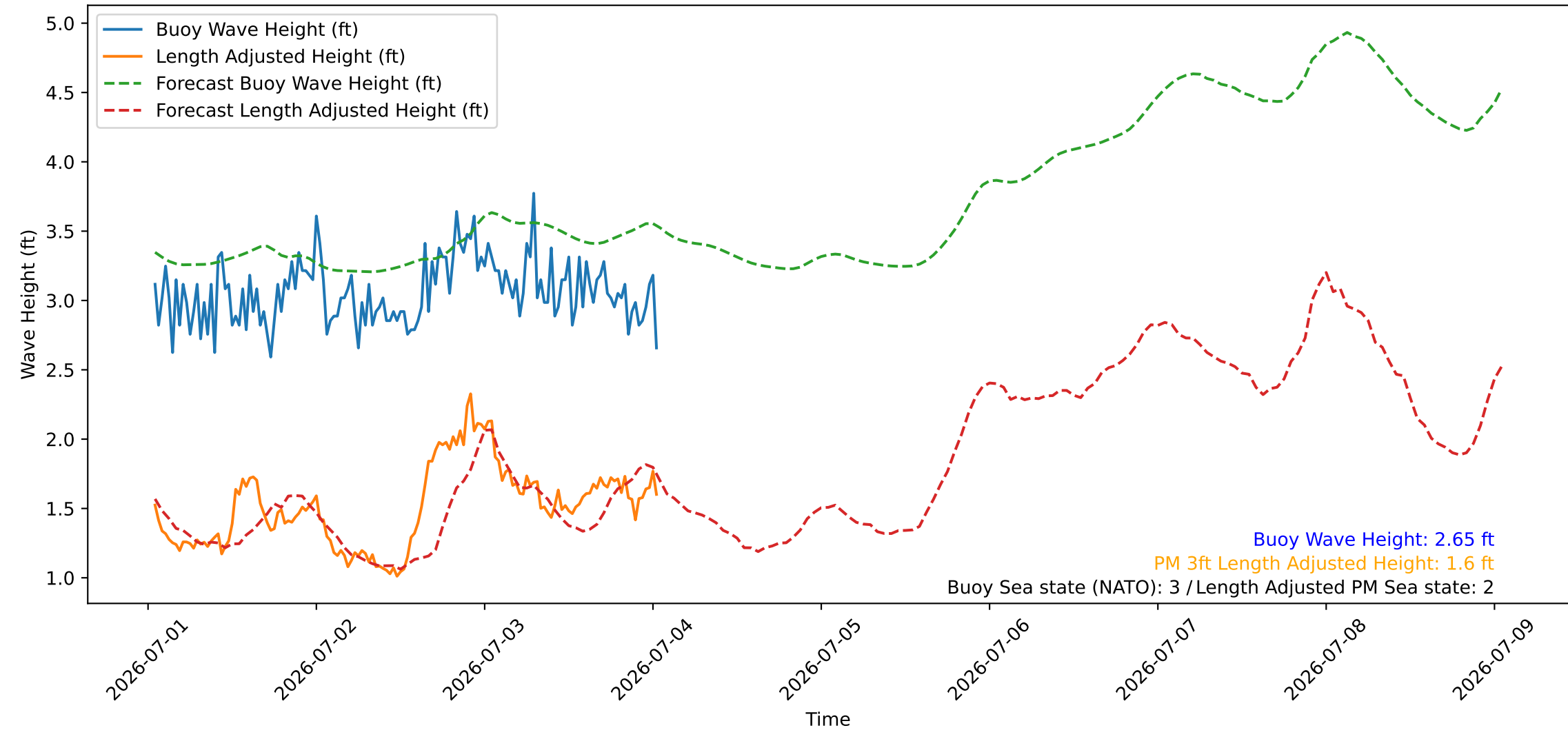
Wave Heights over Time for Oceanside Harbor at 2026-07-04 01:10:27
