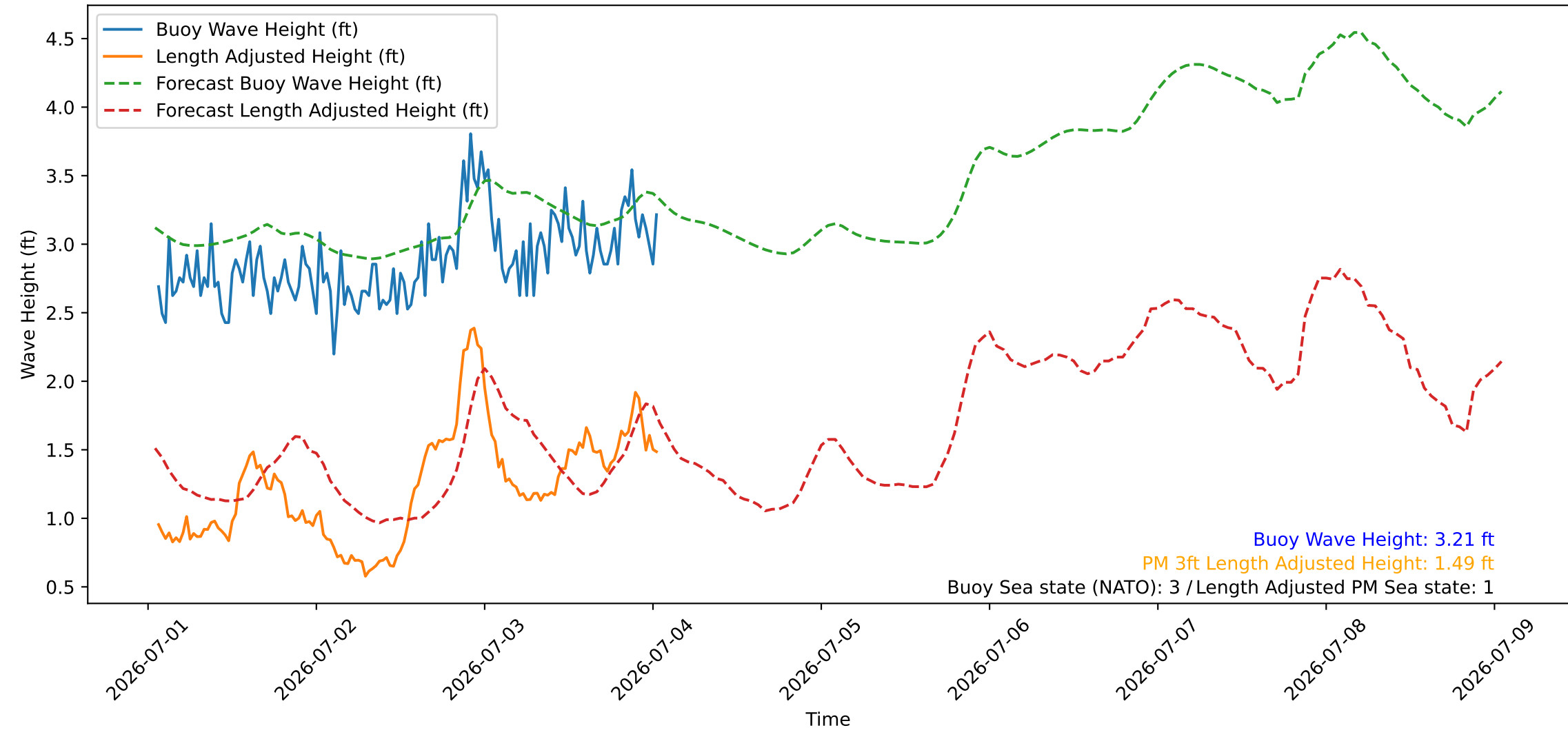
Wave Heights over Time for Red Beach at 2026-07-04 01:10:46
