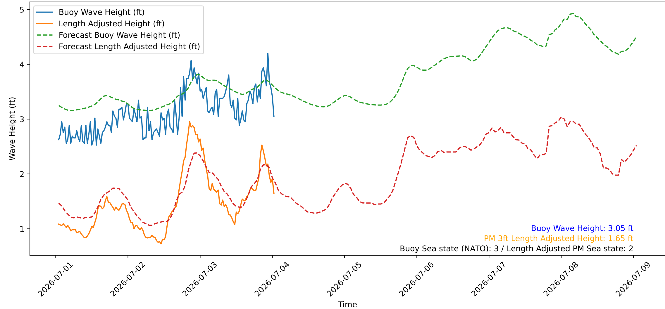
Wave Heights over Time for Green Beach at 2026-07-04 01:11:08
