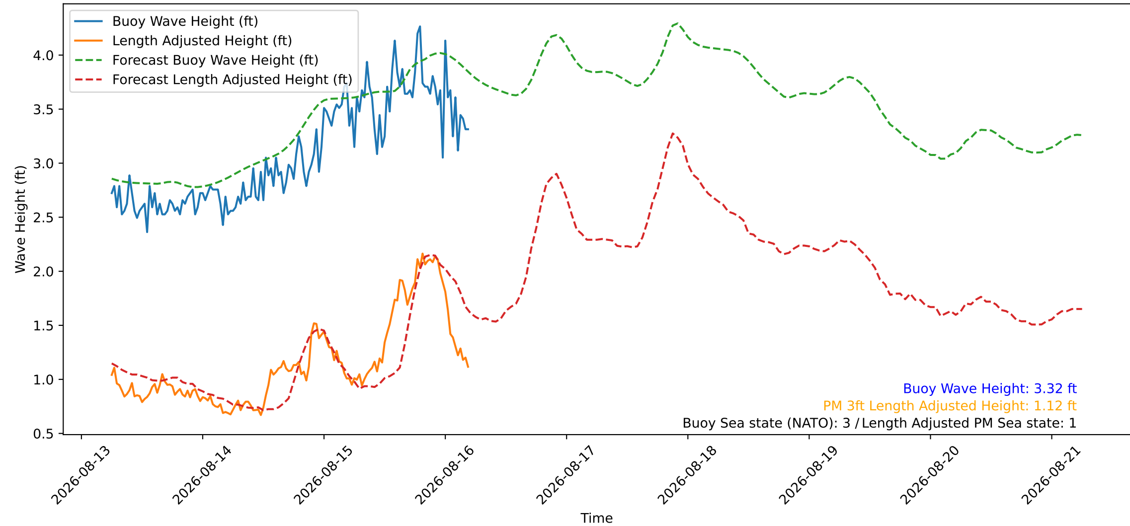
Wave Heights over Time for Green Beach at 2026-08-16 05:31:08
