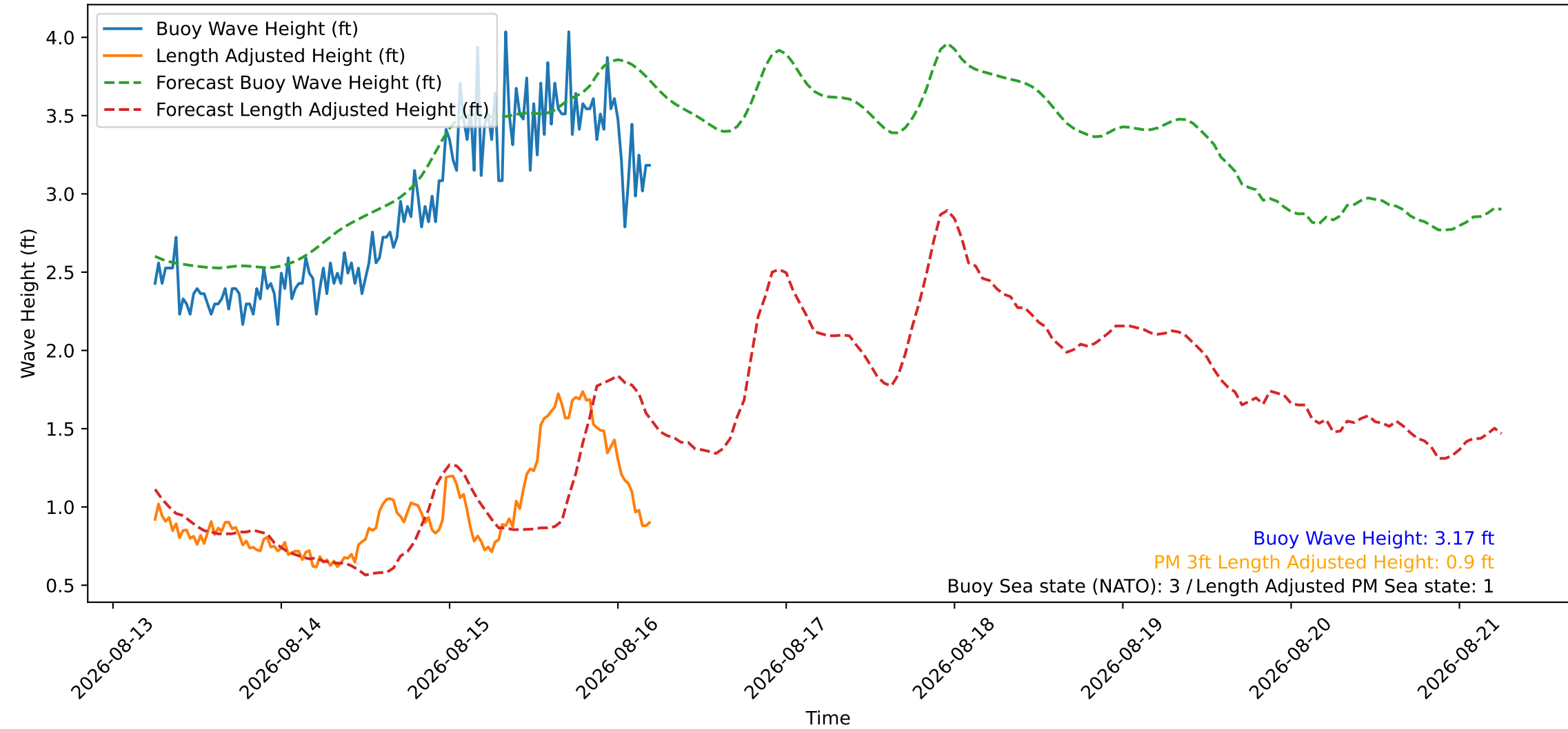
Wave Heights over Time for Red Beach at 2026-08-16 05:30:45
