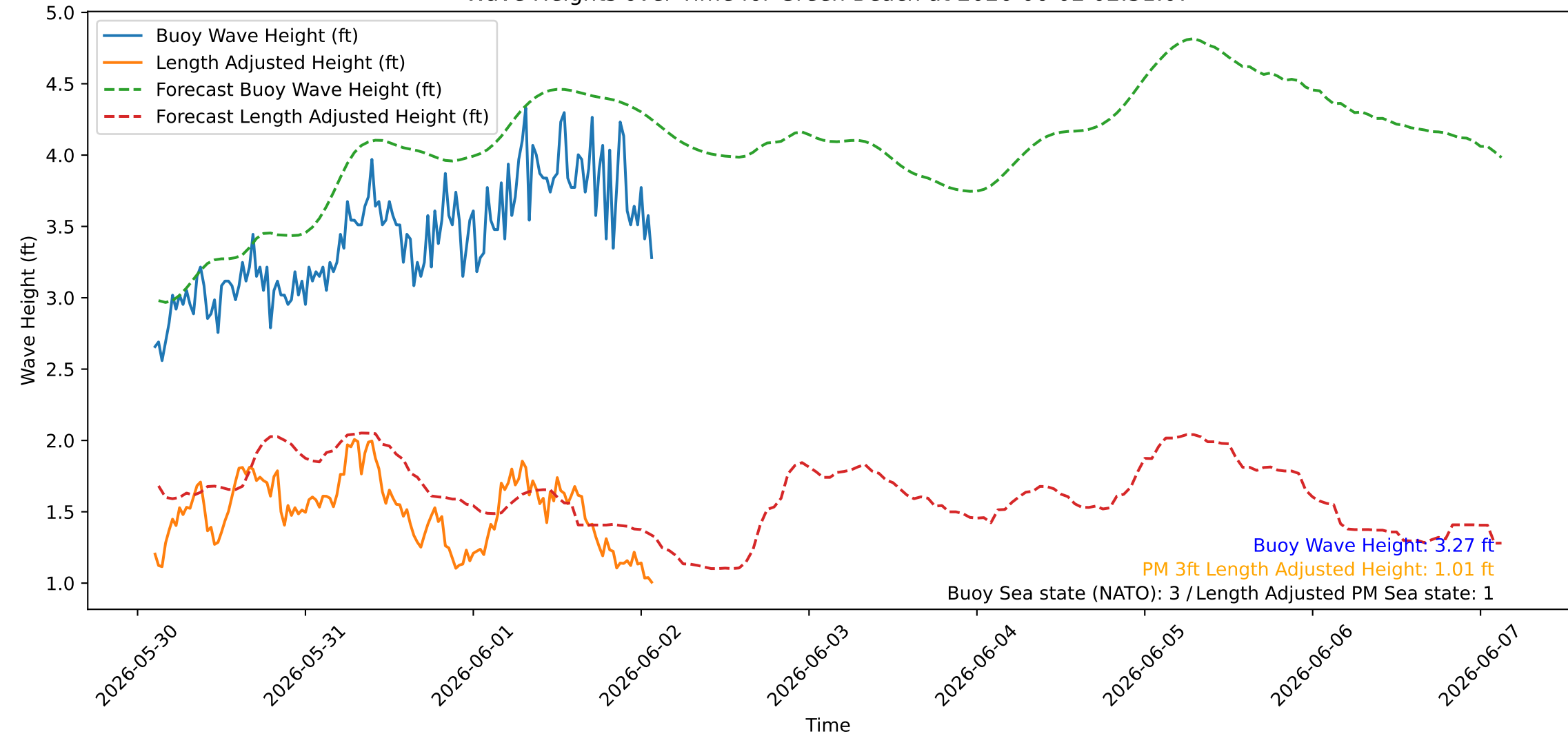
Wave Heights over Time for Green Beach at 2026-06-02 02:31:07
