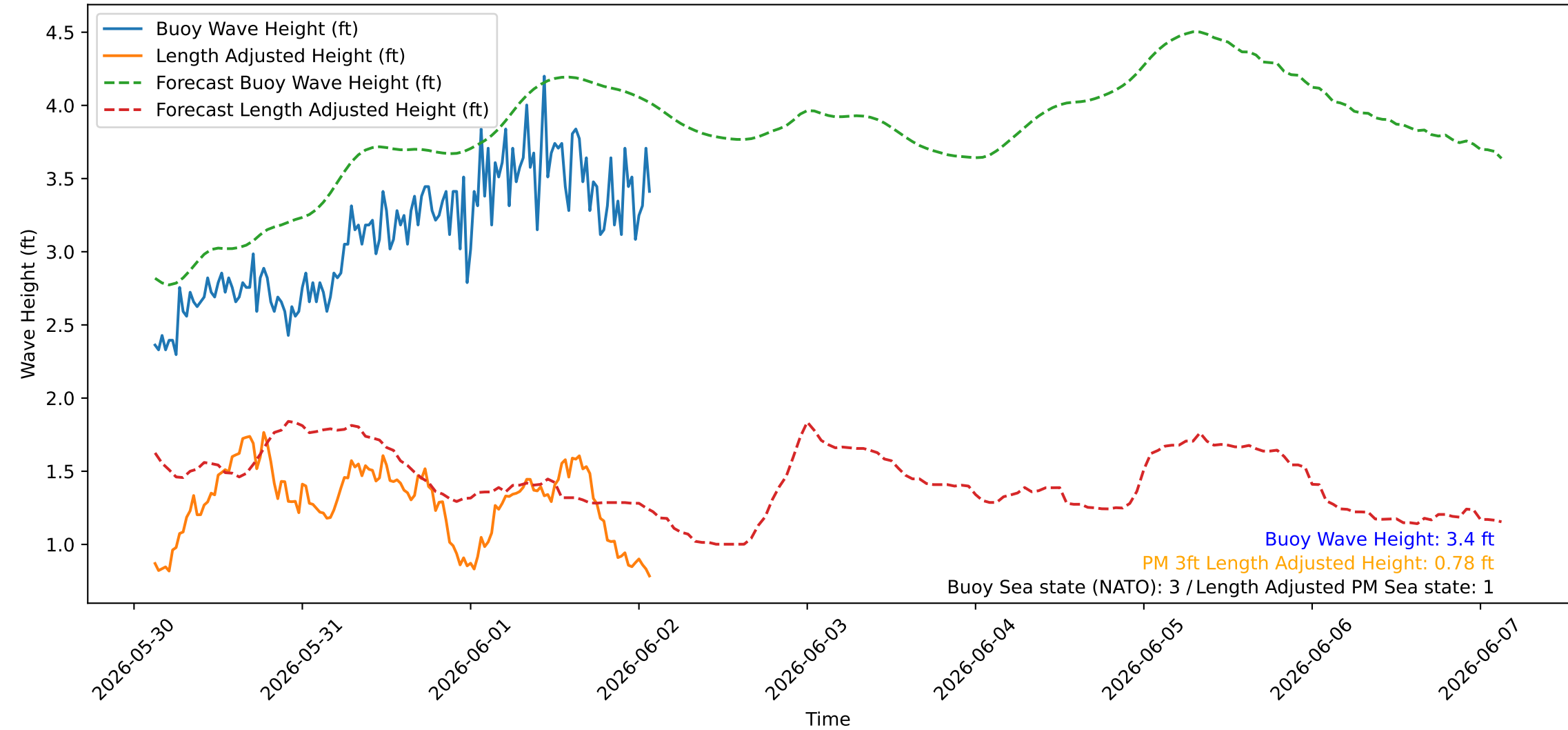
Wave Heights over Time for Red Beach at 2026-06-02 02:30:45
