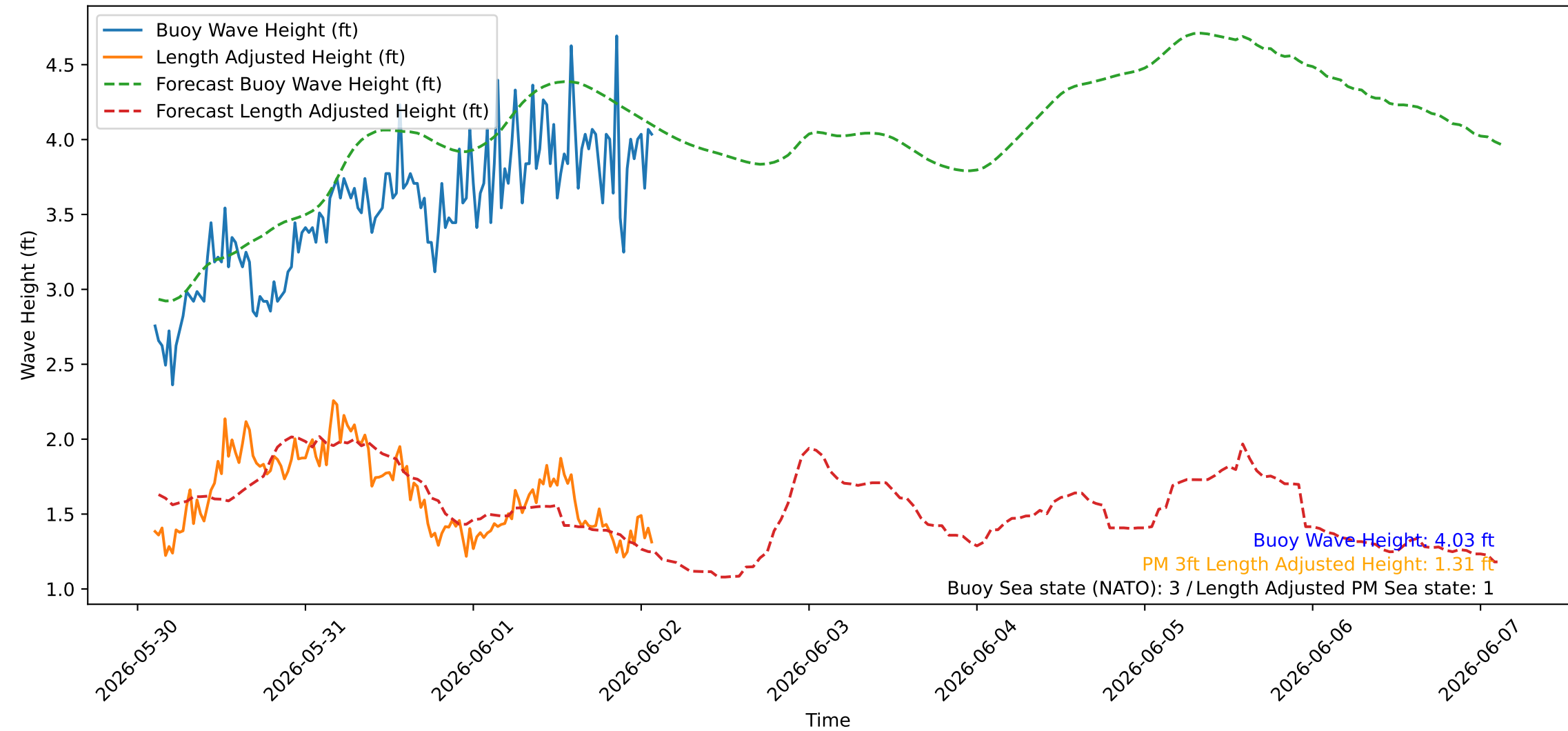
Wave Heights over Time for Oceanside Harbor at 2026-06-02 02:30:26
