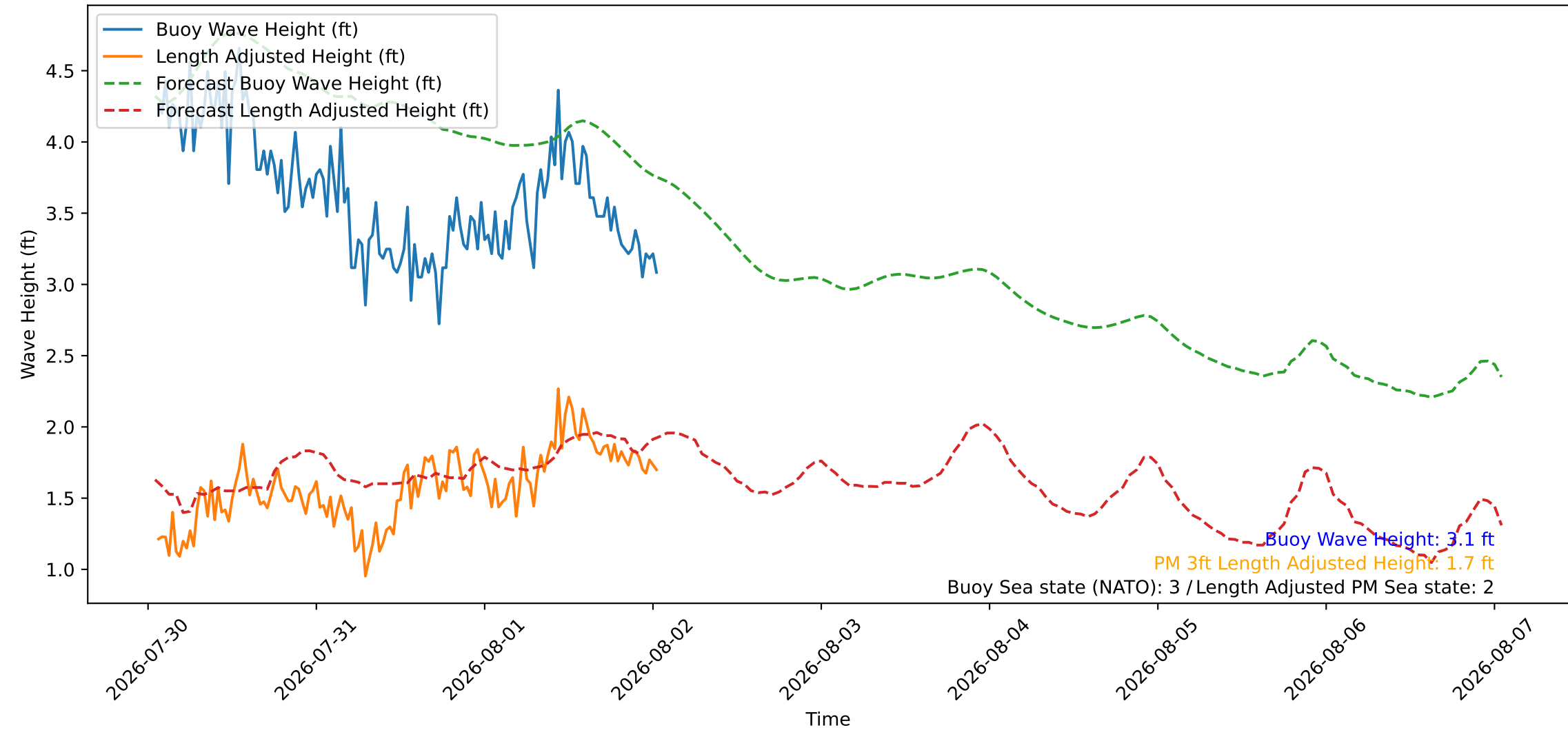
Wave Heights over Time for Oceanside Harbor at 2026-08-02 01:20:26
