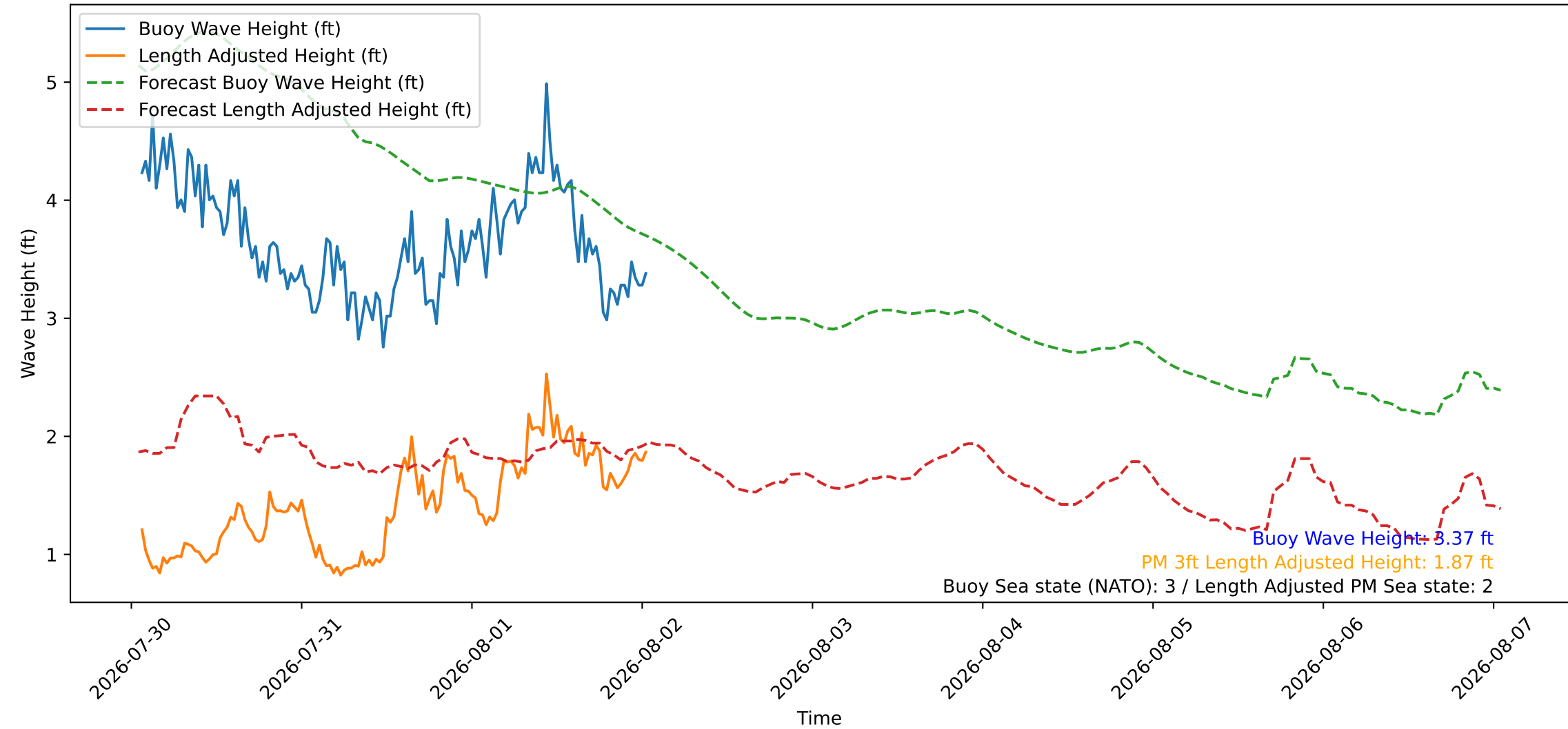
Wave Heights over Time for Green Beach at 2026-08-02 01:21:10
