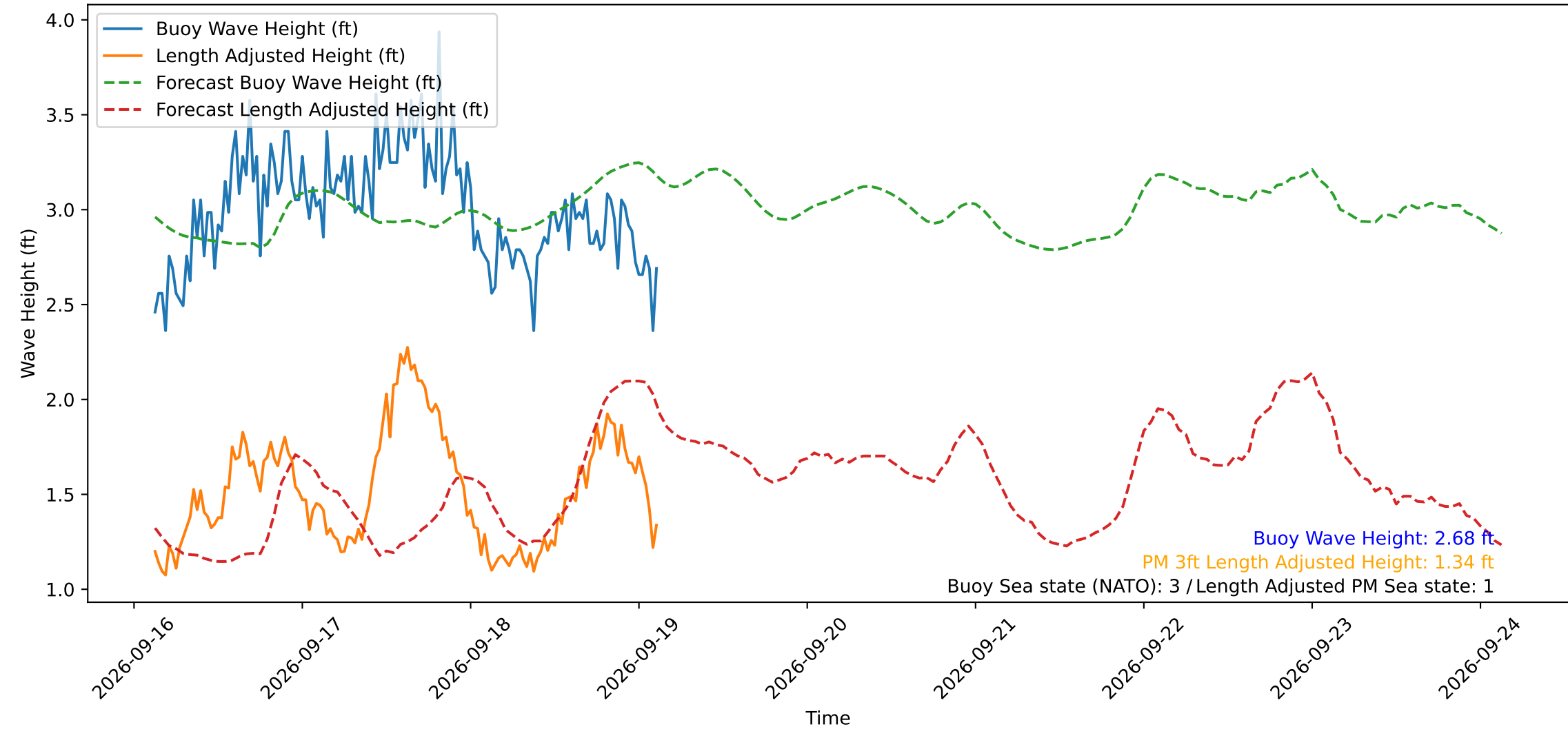
Wave Heights over Time for Oceanside Harbor at 2026-09-19 03:10:30
