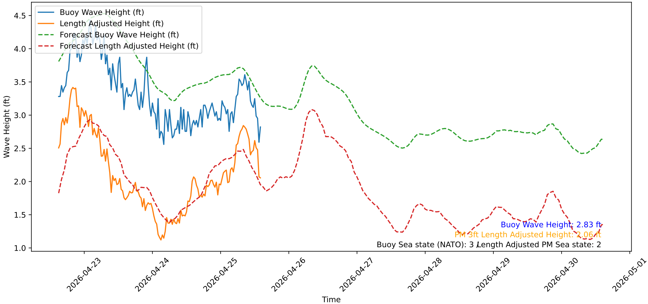
Wave Heights over Time for Oceanside Harbor at 2026-04-25 15:10:31
