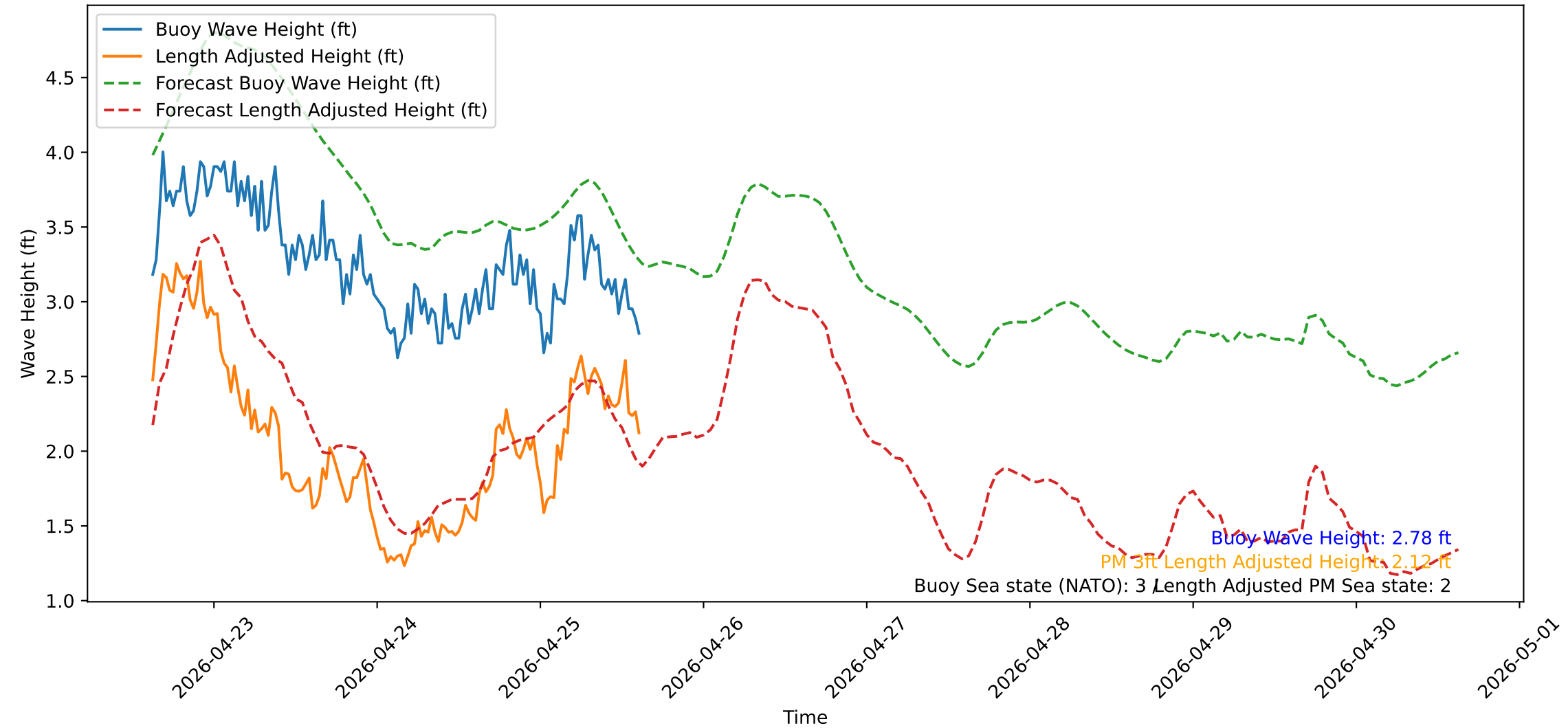
Wave Heights over Time for Green Beach at 2026-04-25 15:11:12
