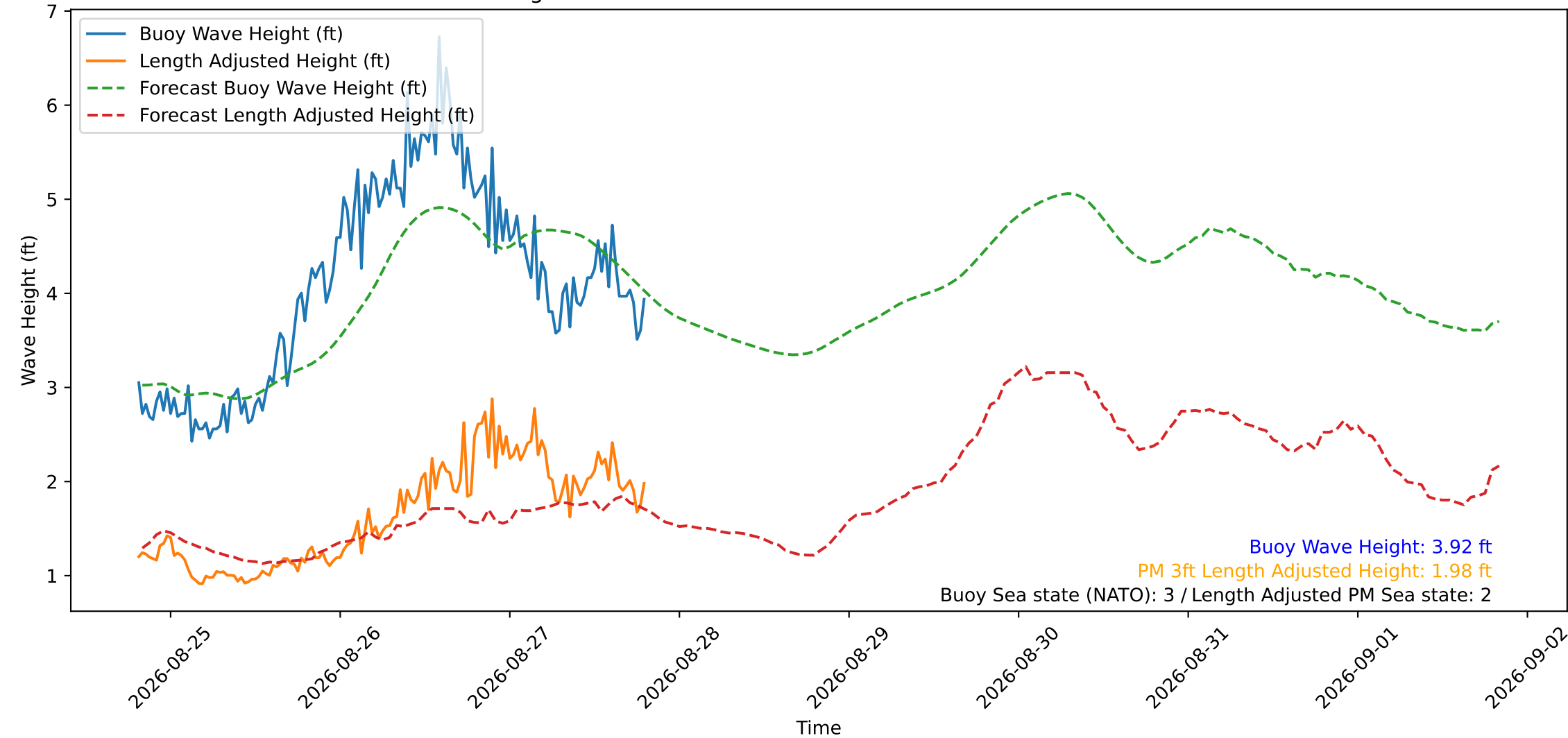
Wave Heights over Time for Oceanside Harbor at 2026-08-27 19:40:29
