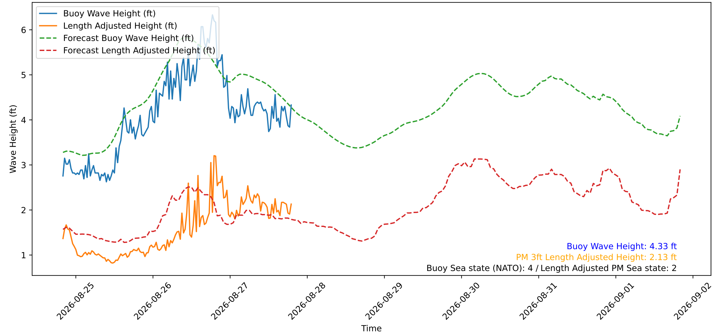
Wave Heights over Time for Green Beach at 2026-08-27 19:41:11
