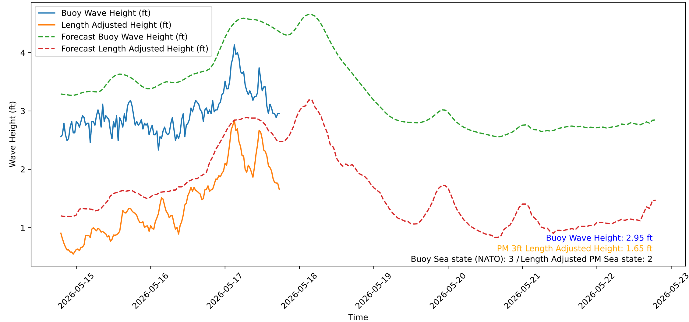
Wave Heights over Time for Red Beach at 2026-05-17 18:30:50
