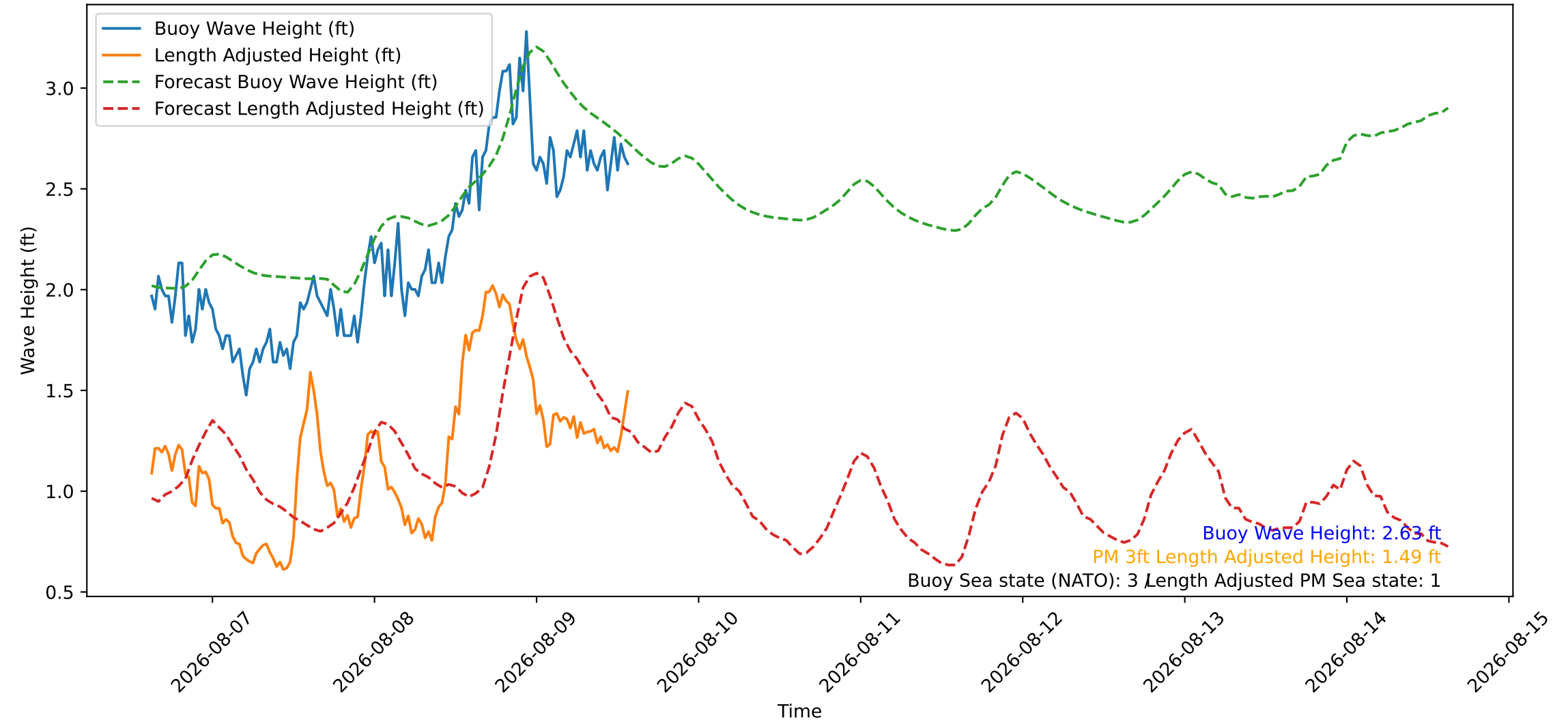
Wave Heights over Time for Red Beach at 2026-08-09 14:40:46
