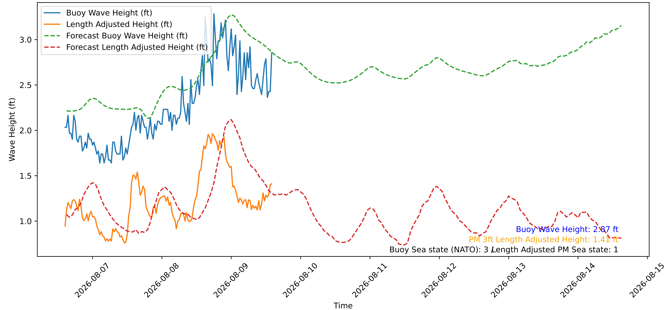
Wave Heights over Time for Oceanside Harbor at 2026-08-09 14:40:27
