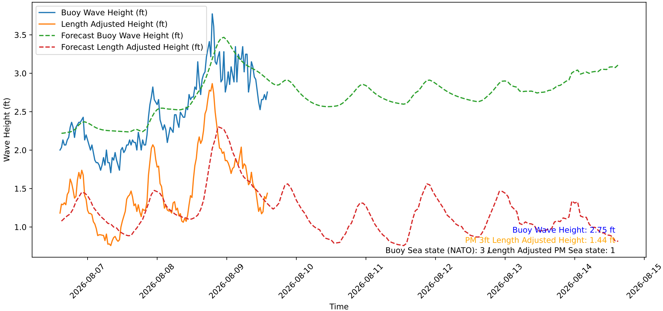
Wave Heights over Time for Green Beach at 2026-08-09 14:41:09
