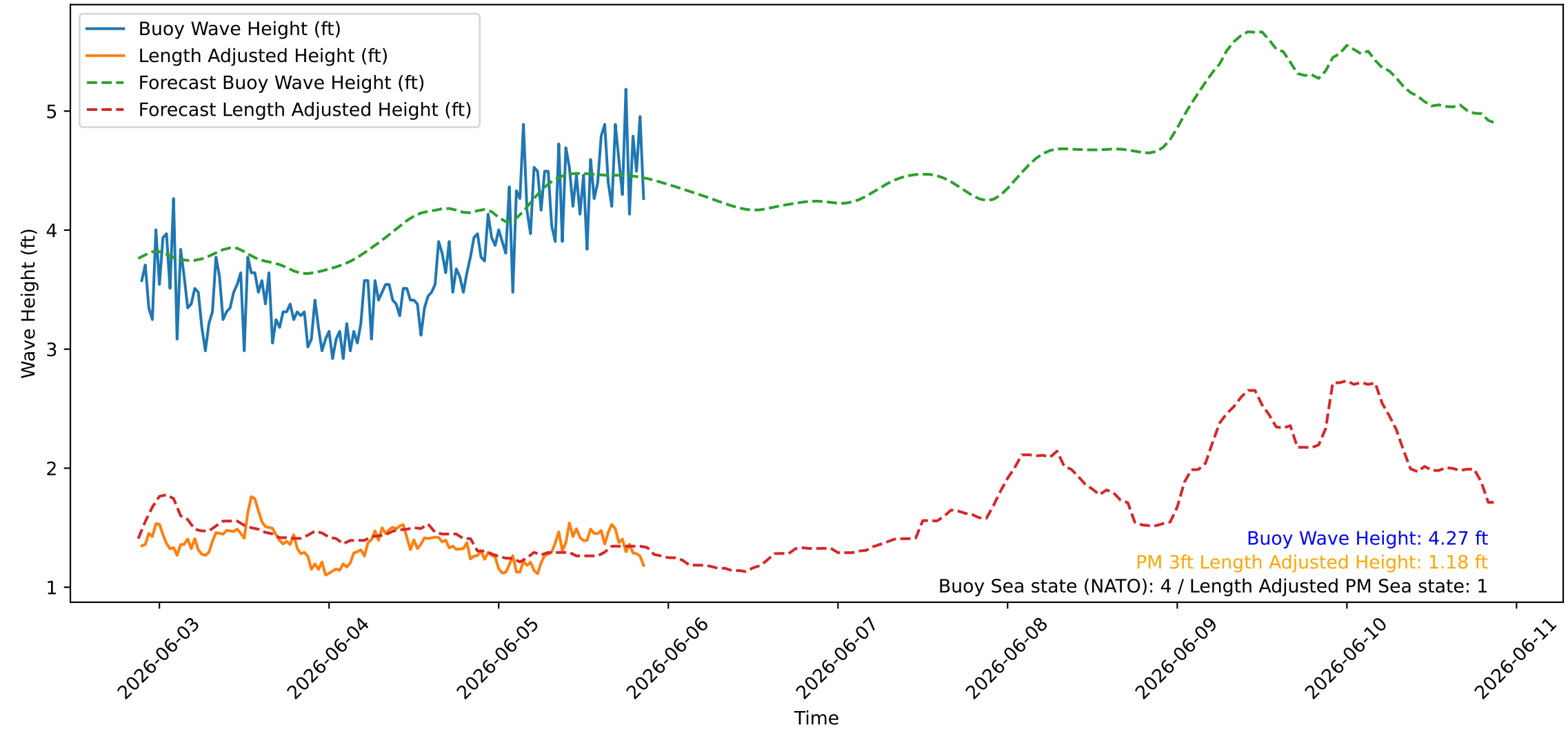
Wave Heights over Time for Oceanside Harbor at 2026-06-05 21:20:25
