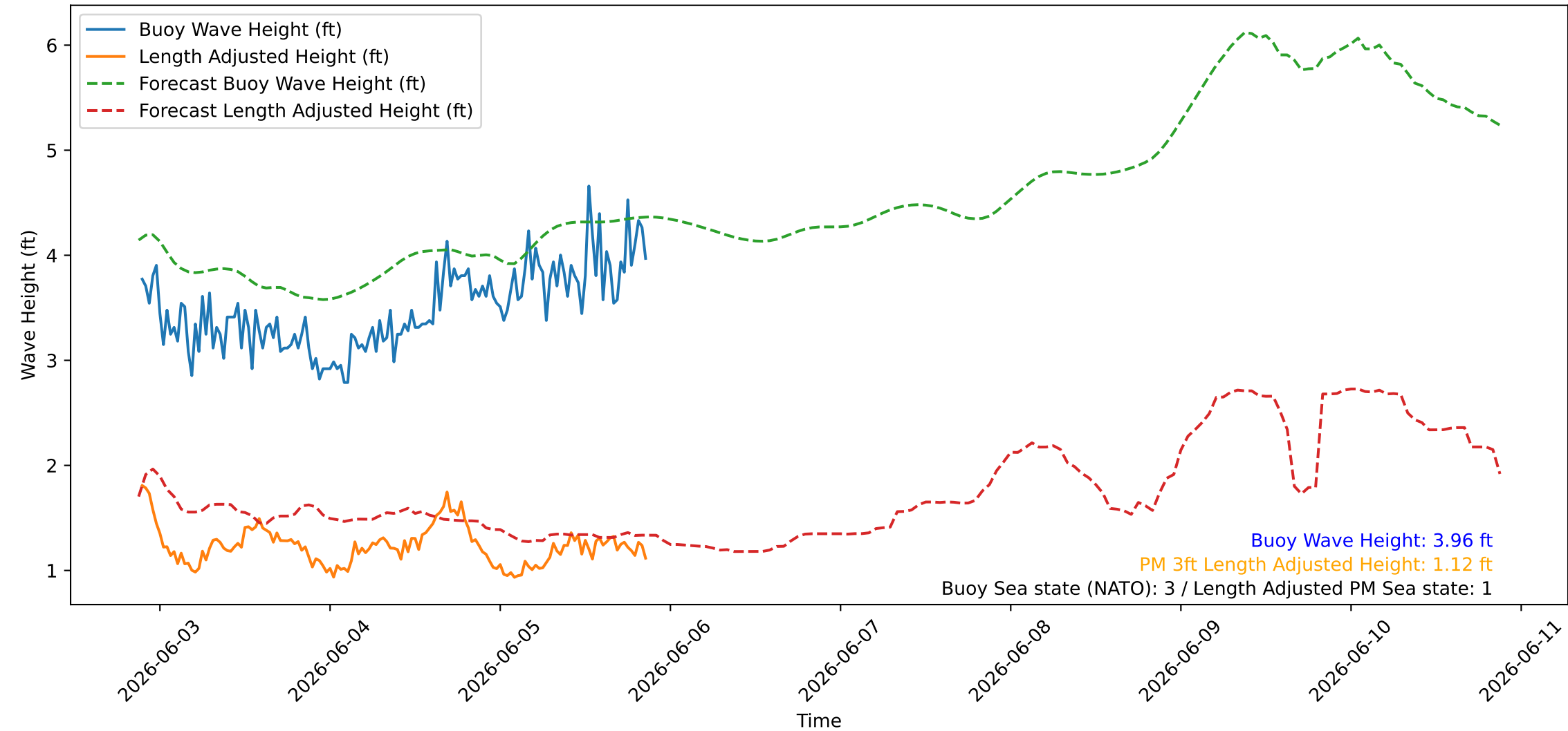
Wave Heights over Time for Green Beach at 2026-06-05 21:21:08
