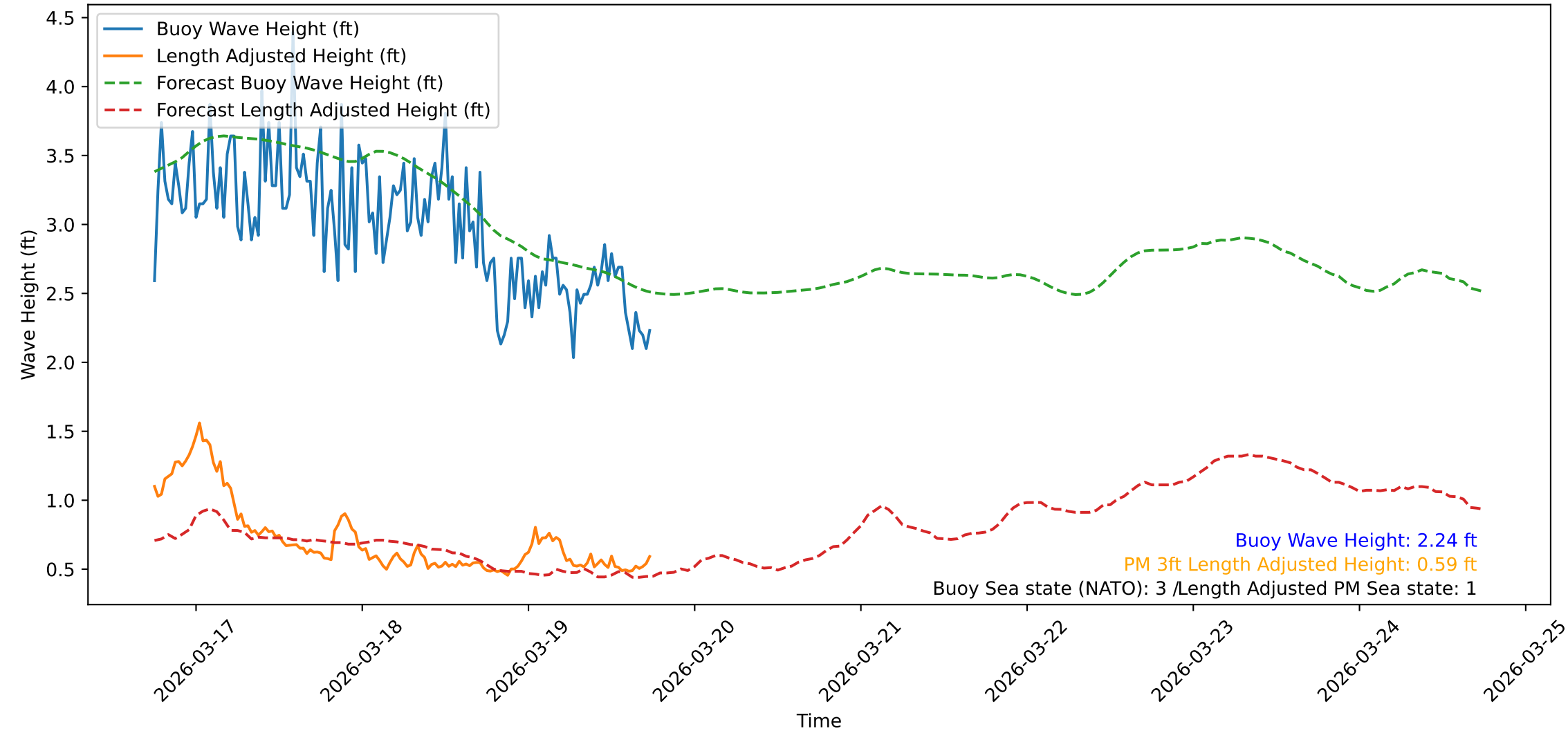
Wave Heights over Time for Oceanside Harbor at 2026-03-19 18:10:31
