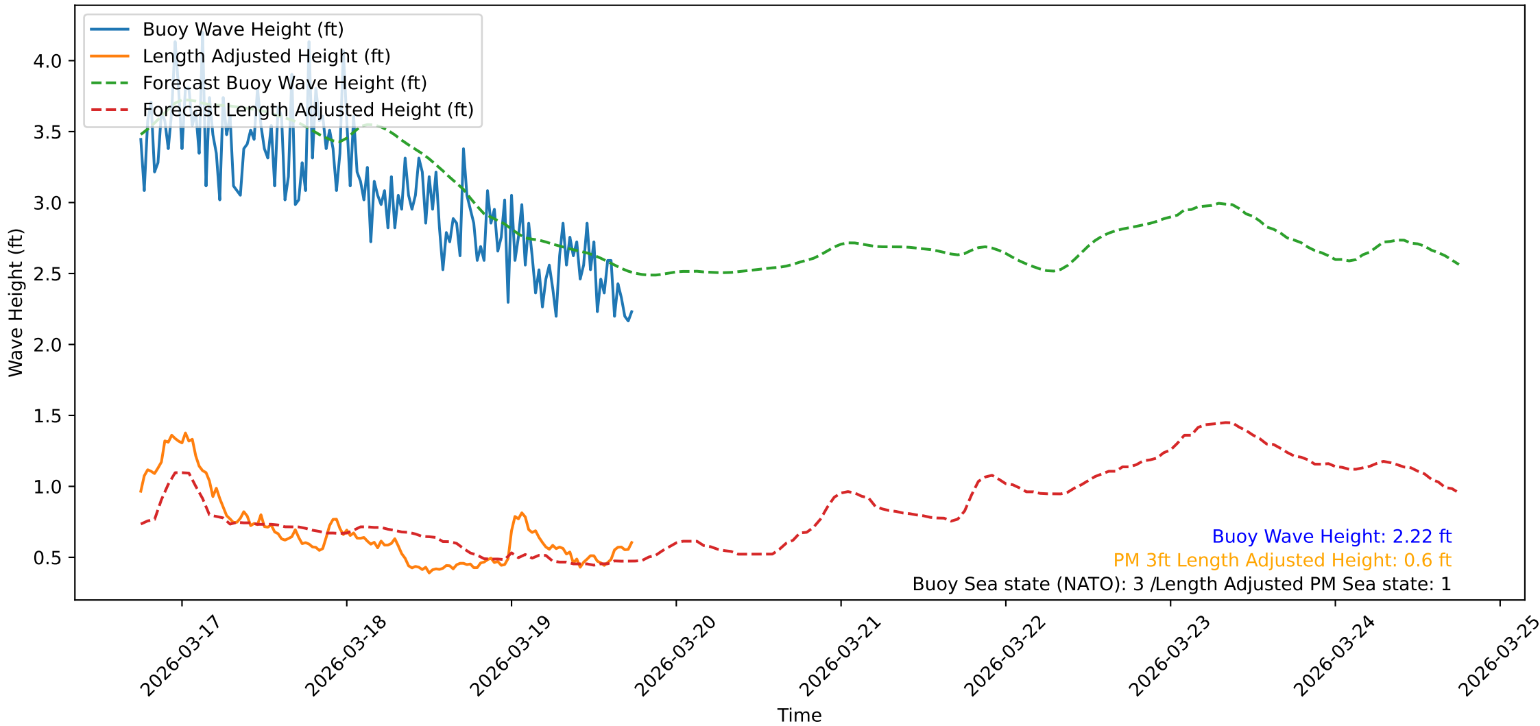
Wave Heights over Time for Green Beach at 2026-03-19 18:11:10
