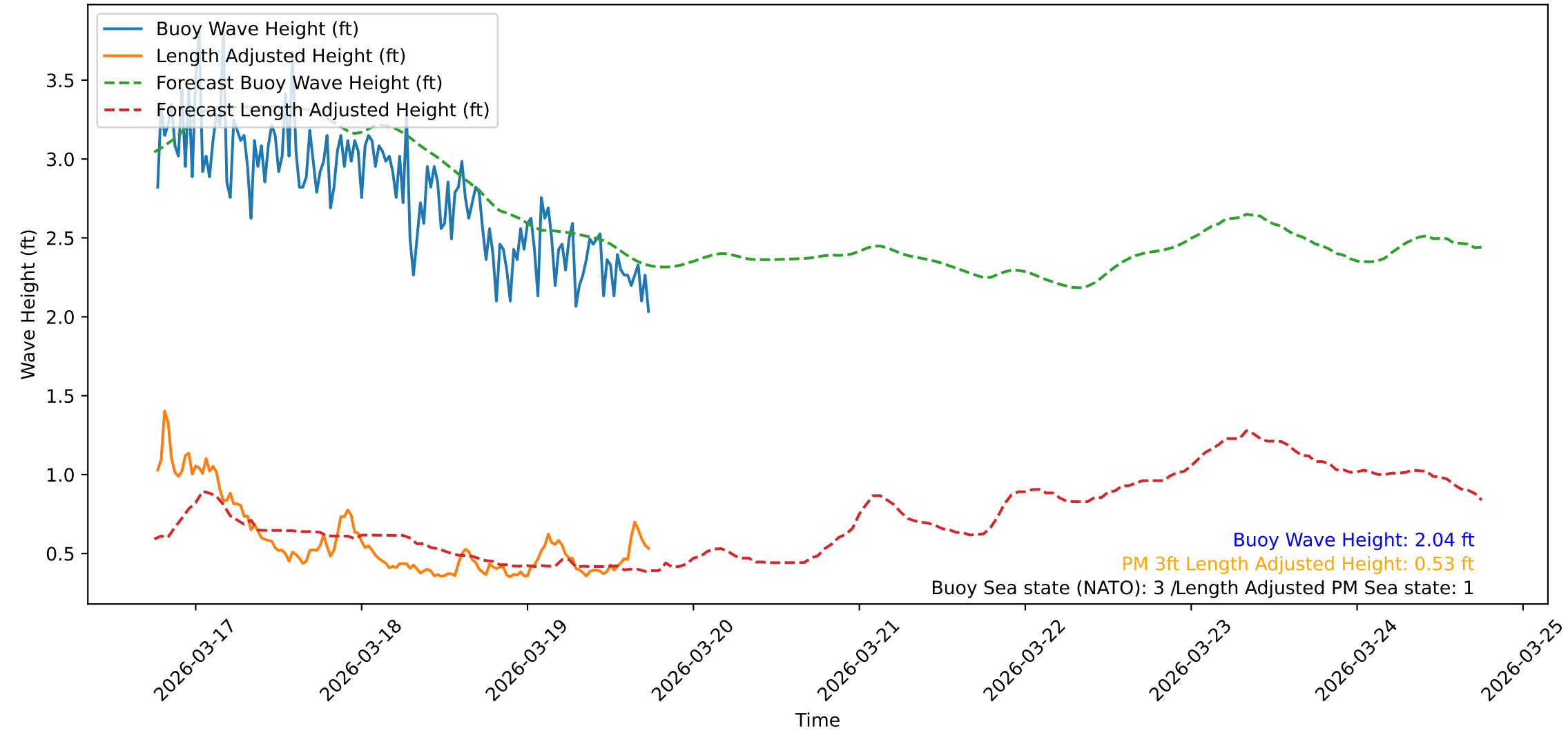
Wave Heights over Time for Red Beach at 2026-03-19 18:10:47
