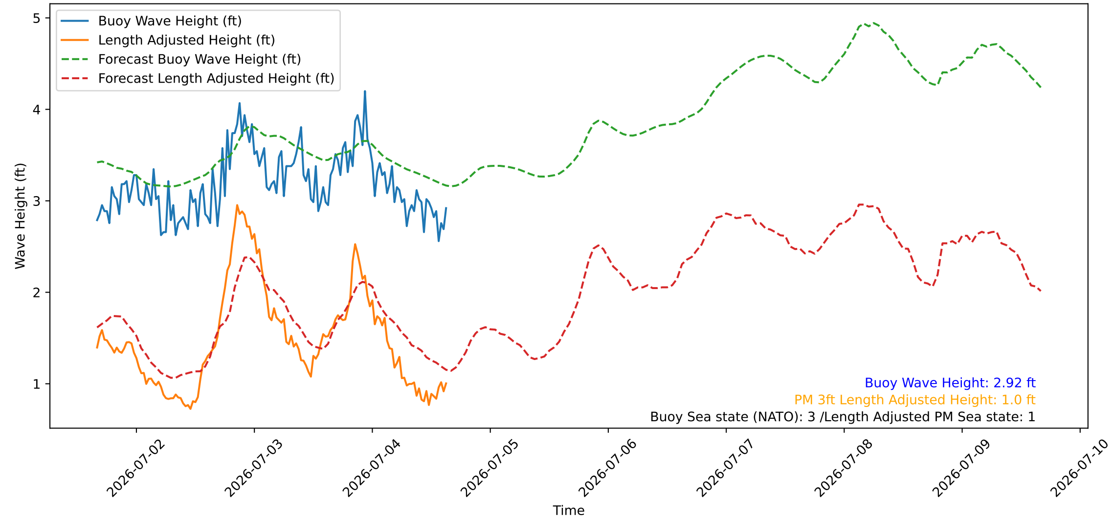
Wave Heights over Time for Green Beach at 2026-07-04 15:51:09
