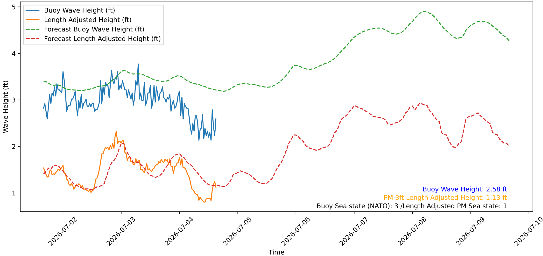
Wave Heights over Time for Oceanside Harbor at 2026-07-04 15:50:26
