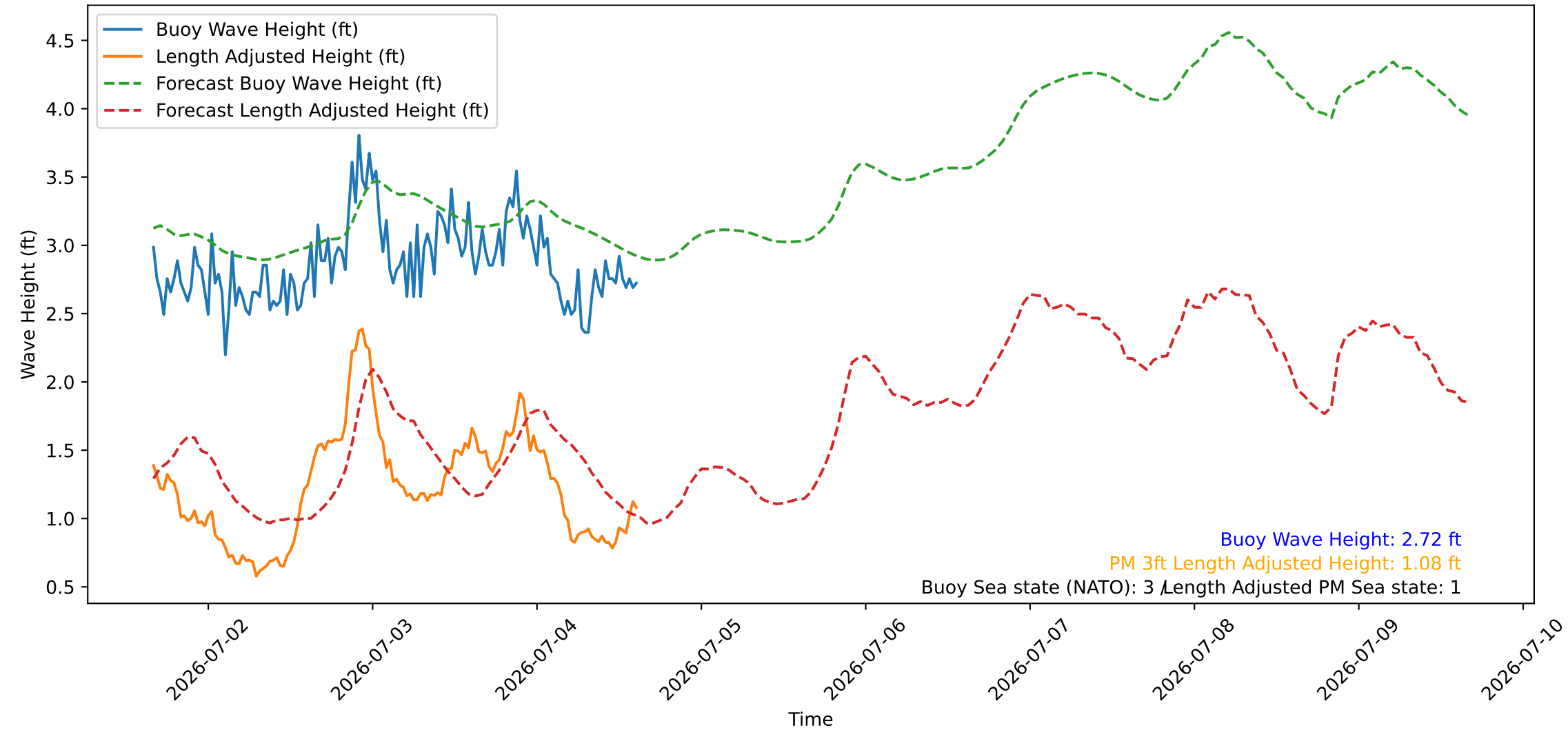
Wave Heights over Time for Red Beach at 2026-07-04 15:50:47
