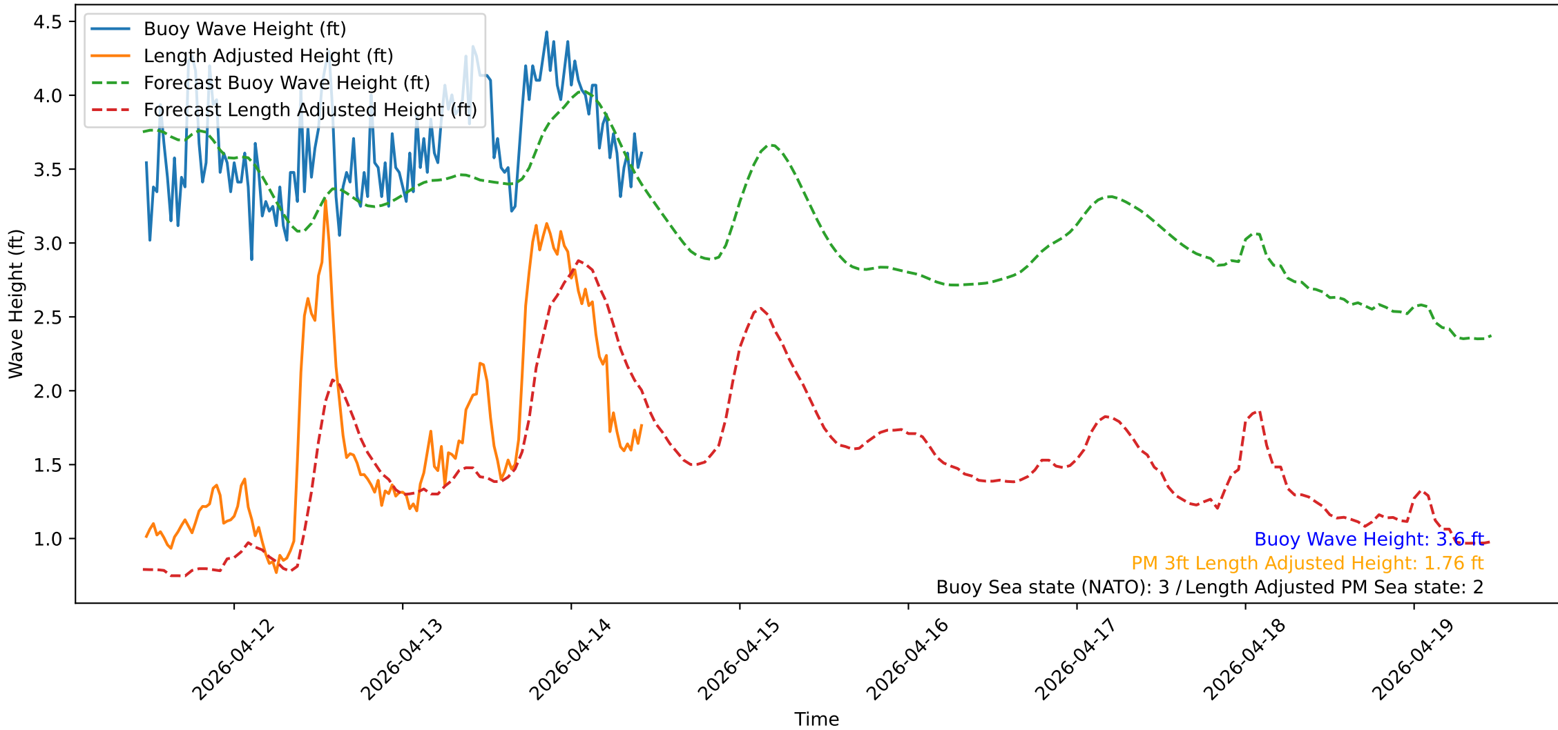
Wave Heights over Time for Red Beach at 2026-04-14 11:00:50
