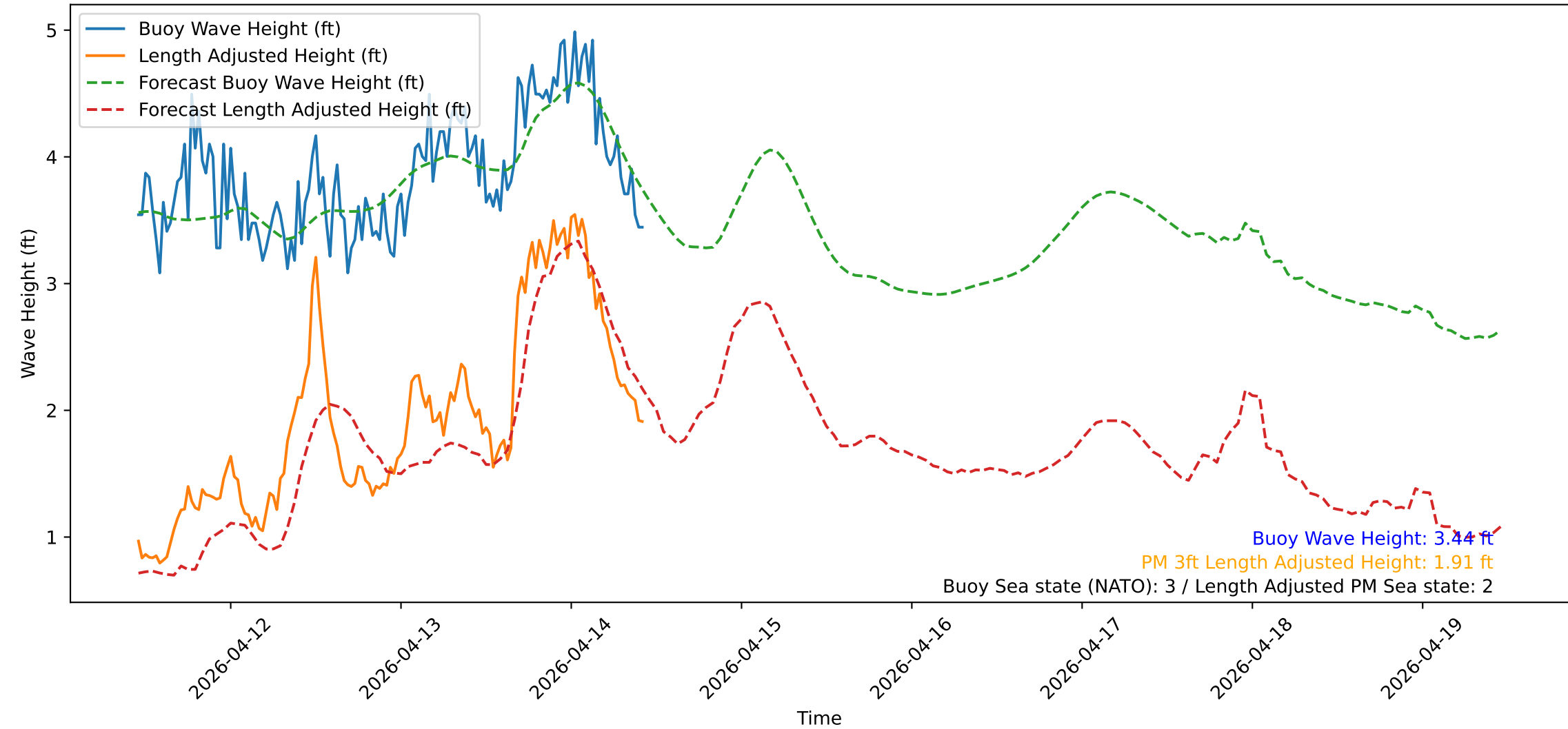
Wave Heights over Time for Green Beach at 2026-04-14 11:01:12
