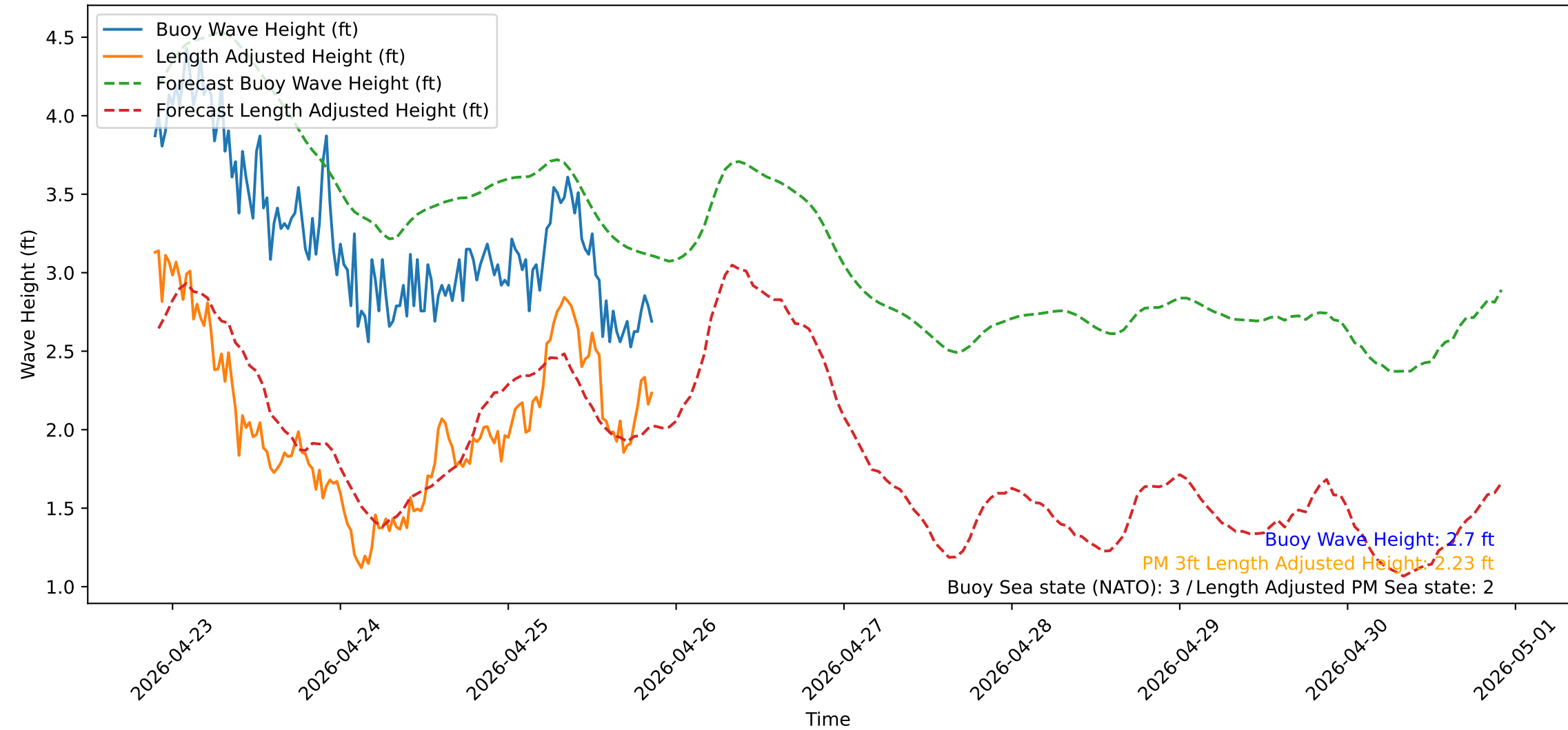
Wave Heights over Time for Oceanside Harbor at 2026-04-25 21:40:31
