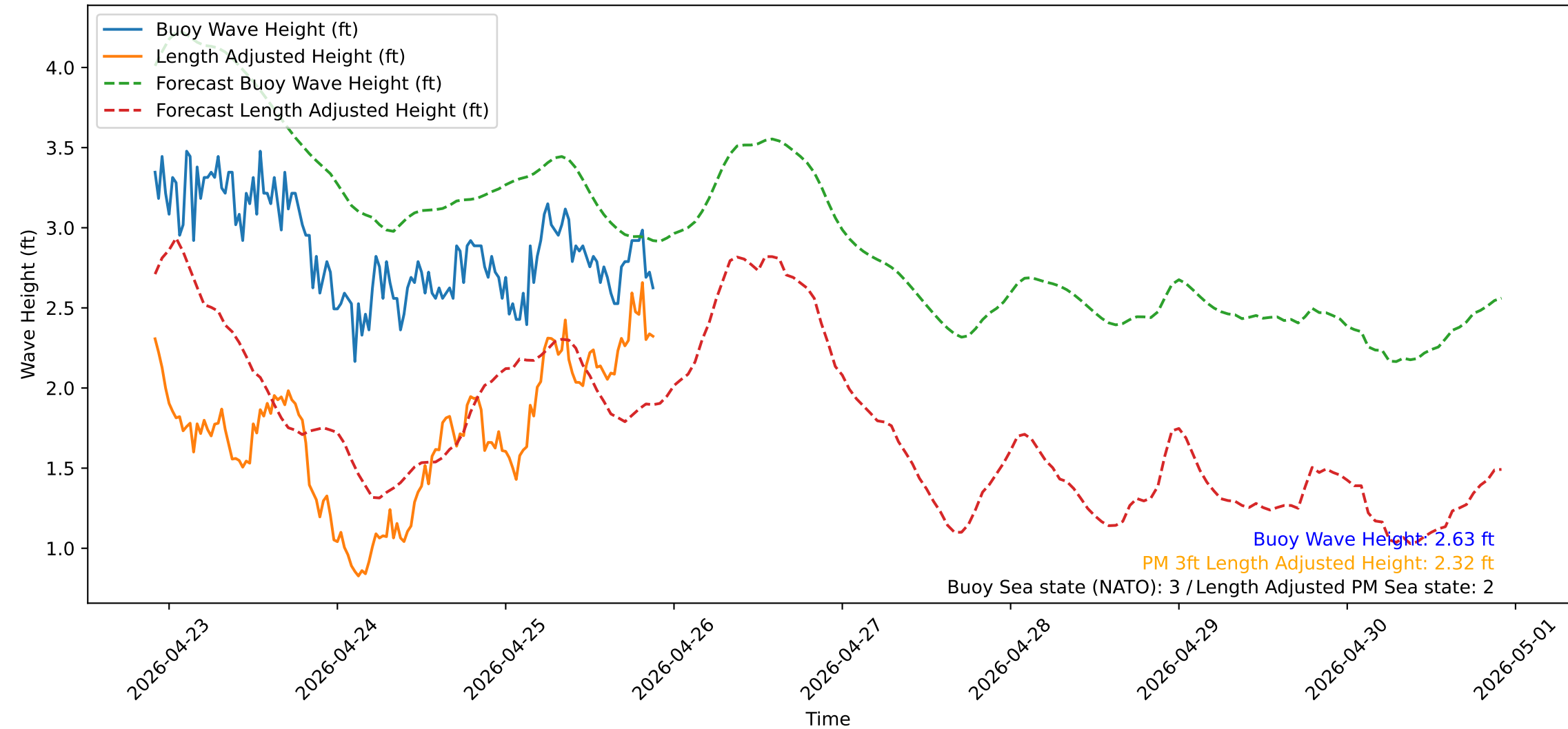
Wave Heights over Time for Red Beach at 2026-04-25 21:40:50
