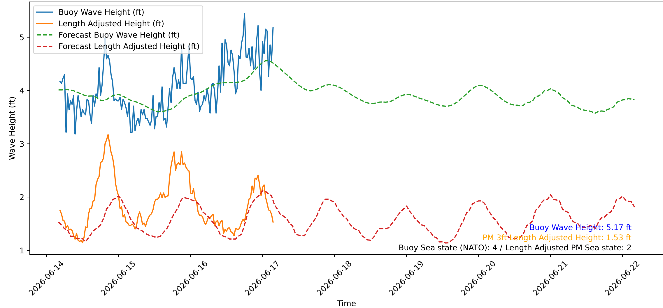
Wave Heights over Time for Oceanside Harbor at 2026-06-17 04:20:26
