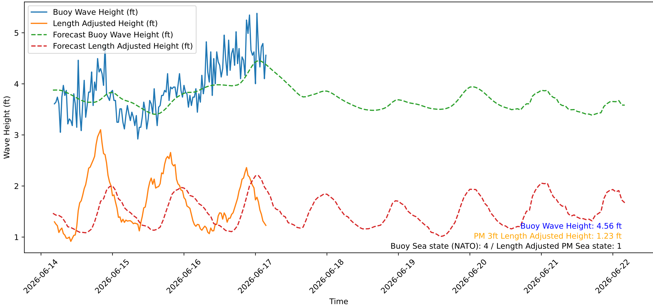
Wave Heights over Time for Red Beach at 2026-06-17 04:20:47
