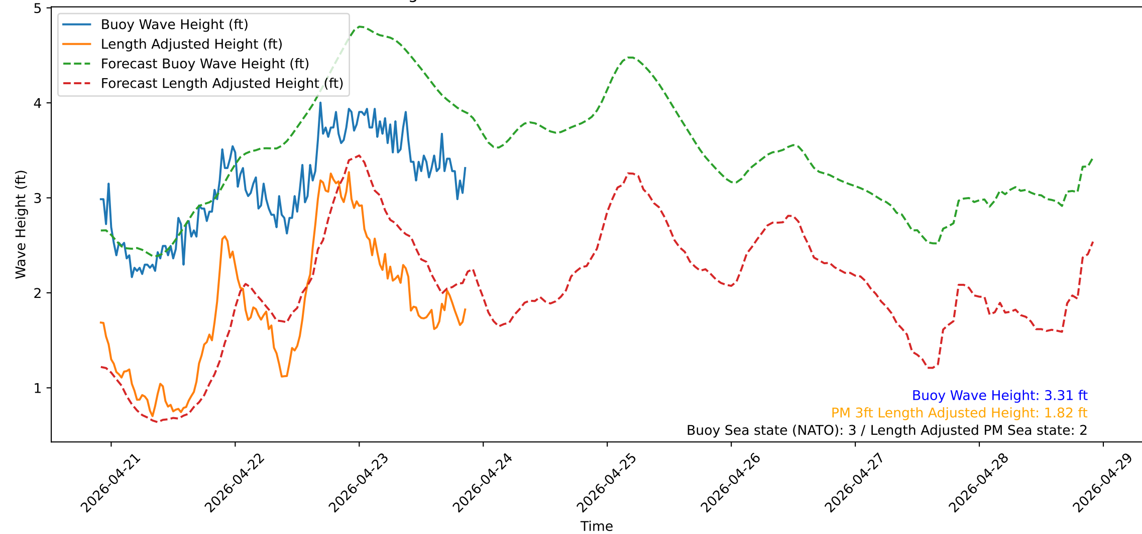
Wave Heights over Time for Green Beach at 2026-04-23 21:51:14
