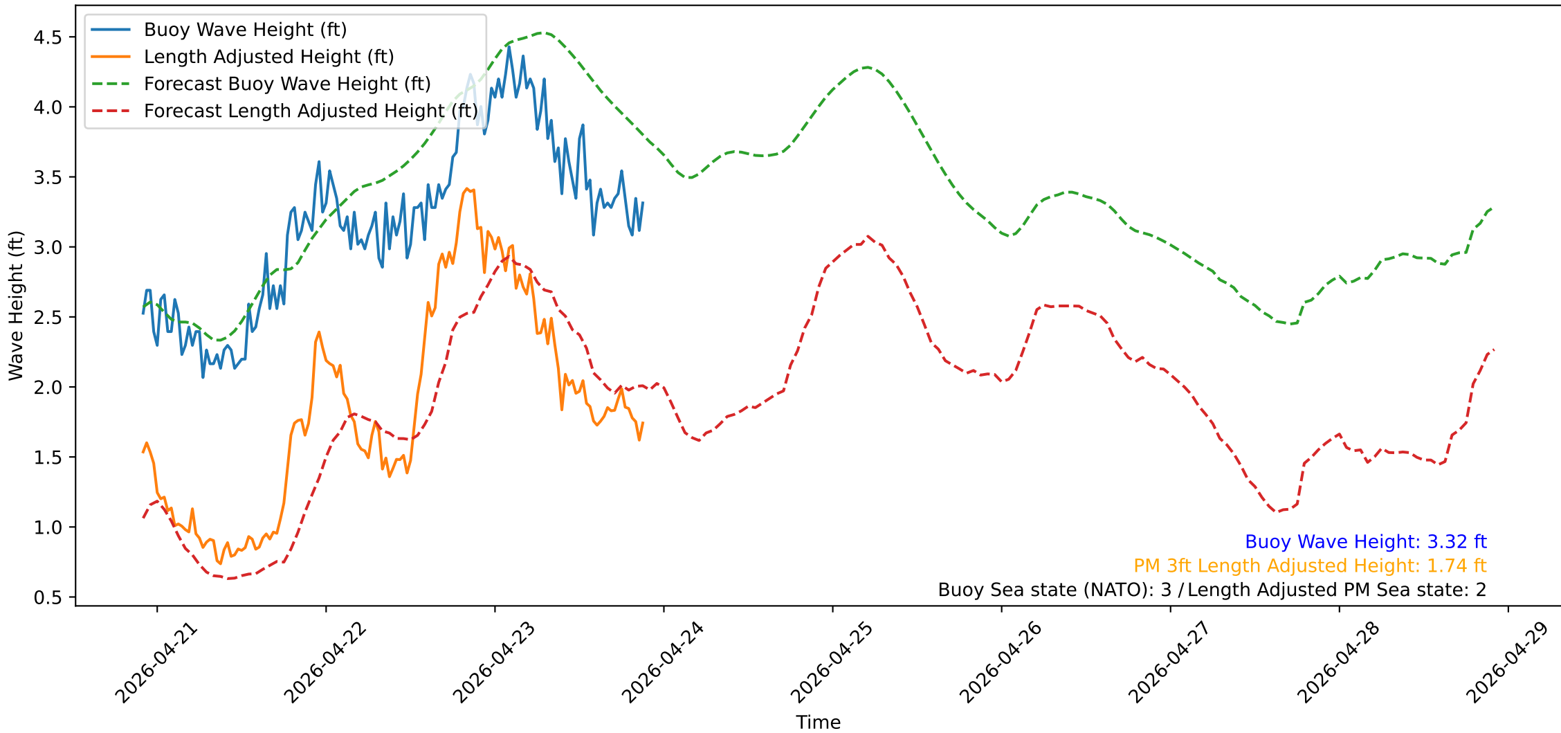
Wave Heights over Time for Oceanside Harbor at 2026-04-23 21:50:31
