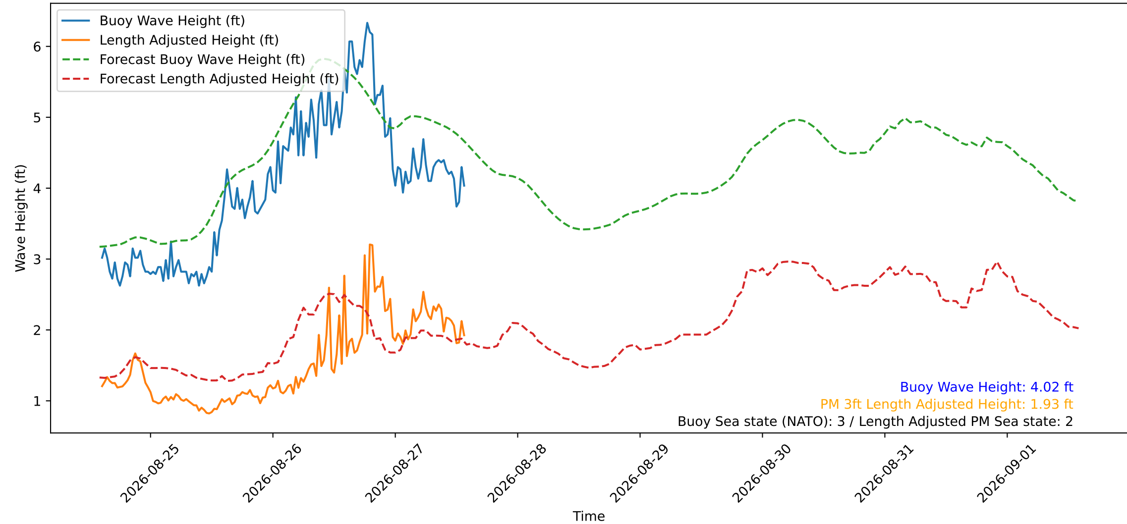
Wave Heights over Time for Green Beach at 2026-08-27 14:21:14
