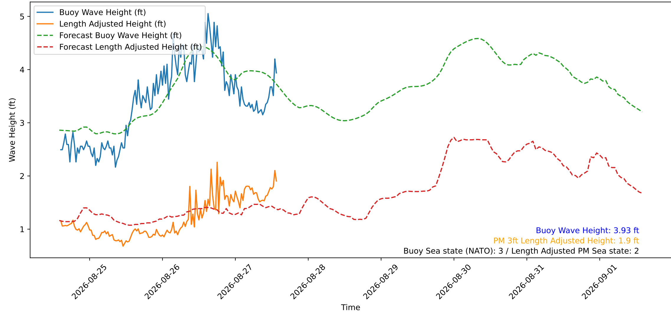
Wave Heights over Time for Red Beach at 2026-08-27 14:20:50
