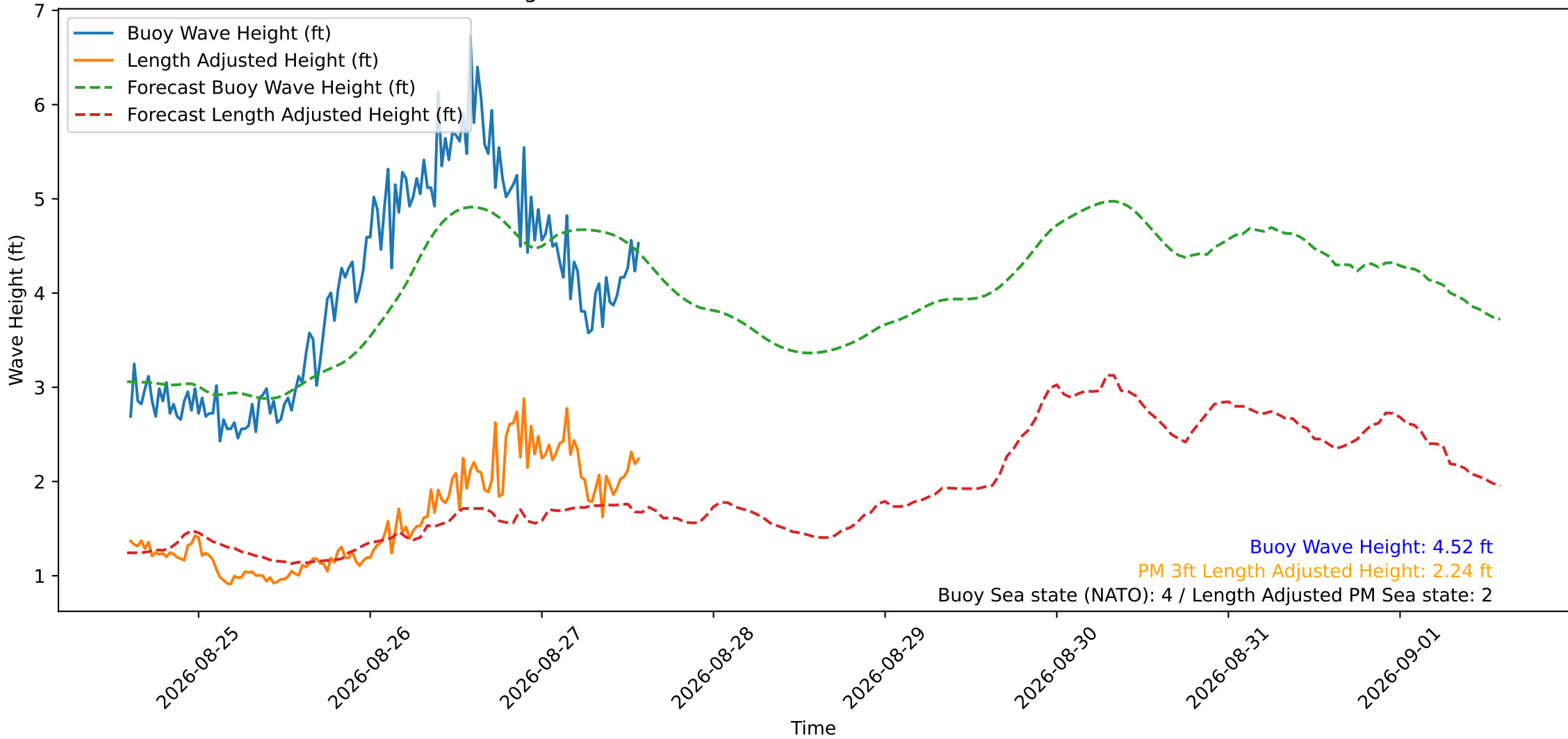
Wave Heights over Time for Oceanside Harbor at 2026-08-27 14:20:29
