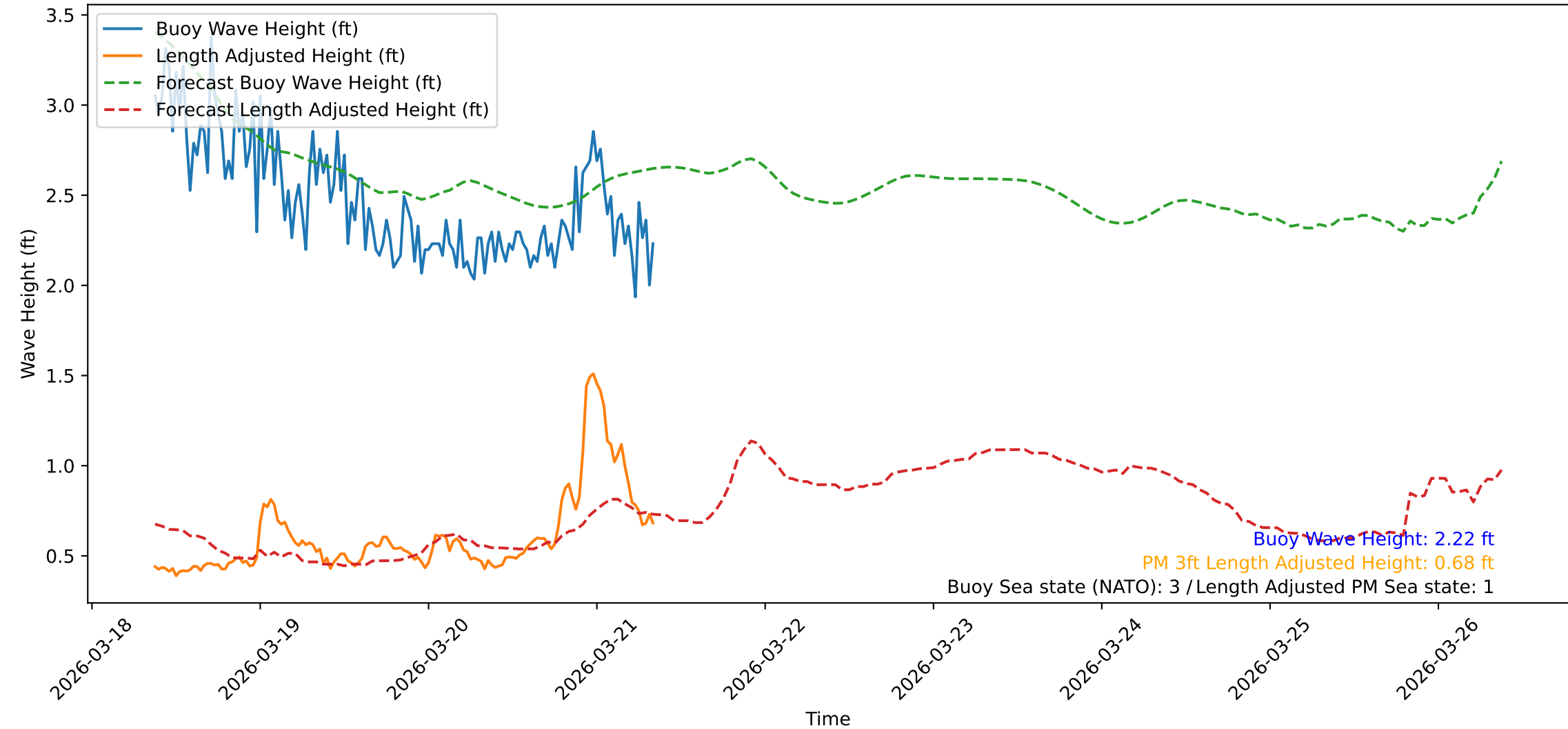
Wave Heights over Time for Green Beach at 2026-03-21 08:51:10
