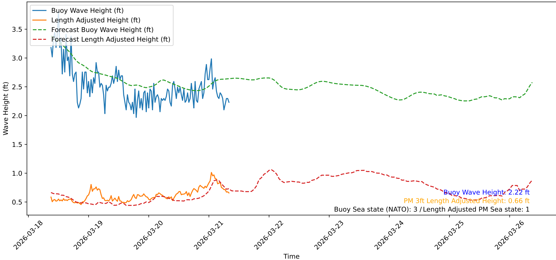
Wave Heights over Time for Oceanside Harbor at 2026-03-21 08:50:31
