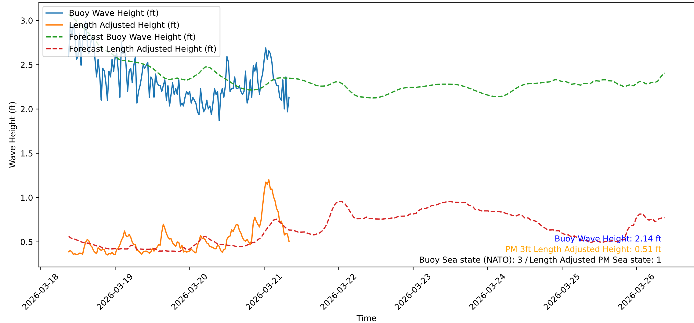
Wave Heights over Time for Red Beach at 2026-03-21 08:50:48
