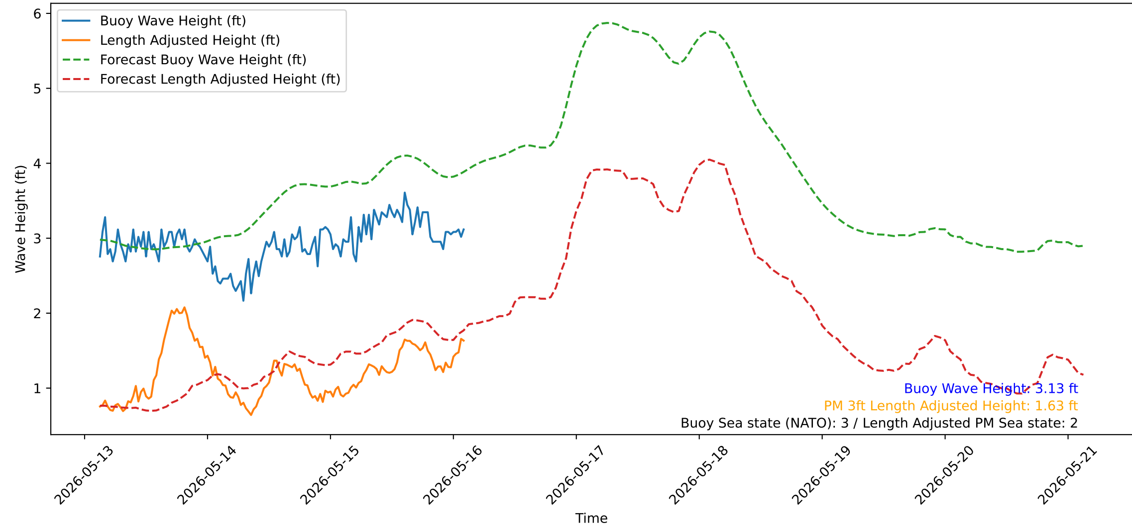
Wave Heights over Time for Oceanside Harbor at 2026-05-16 03:00:31
