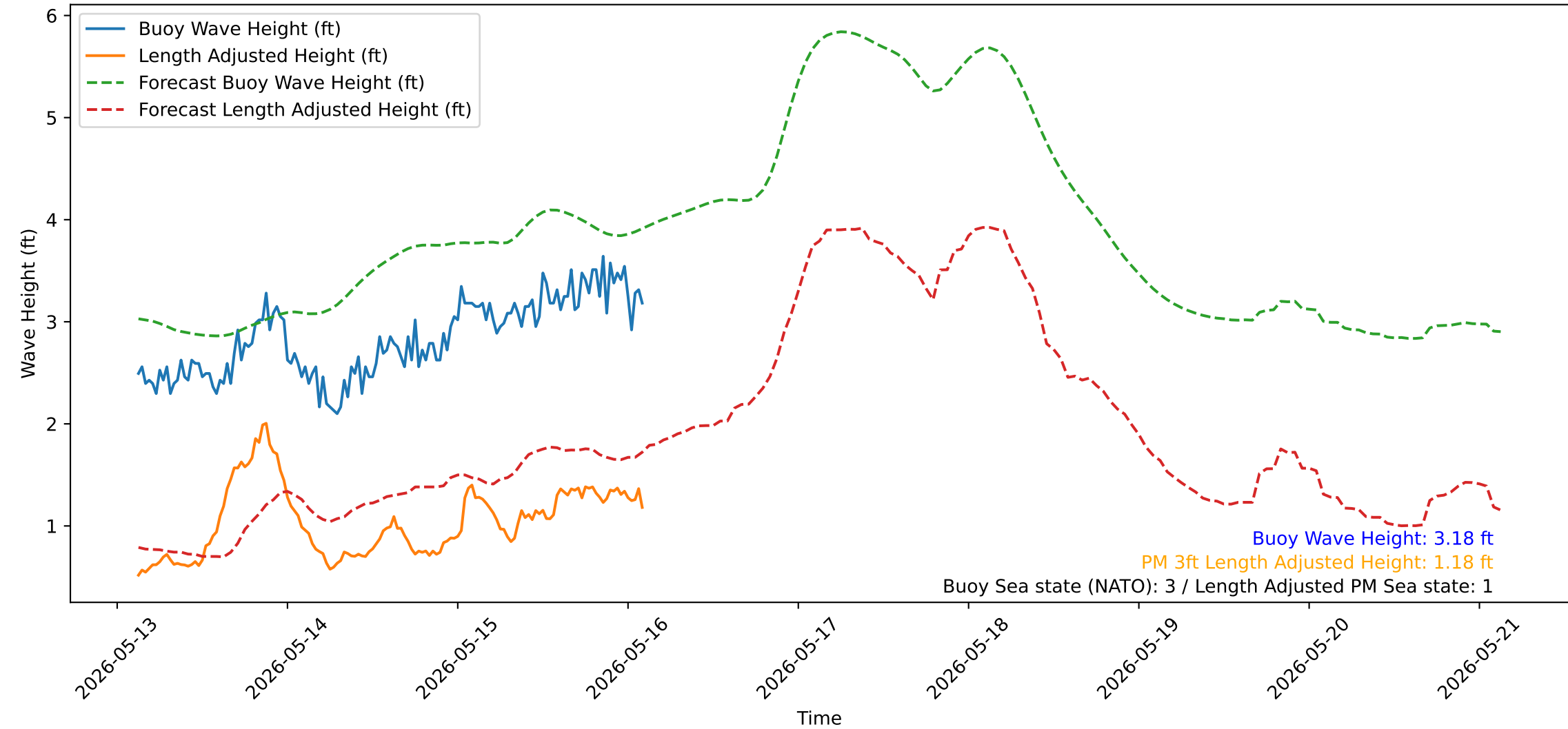
Wave Heights over Time for Green Beach at 2026-05-16 03:01:14
