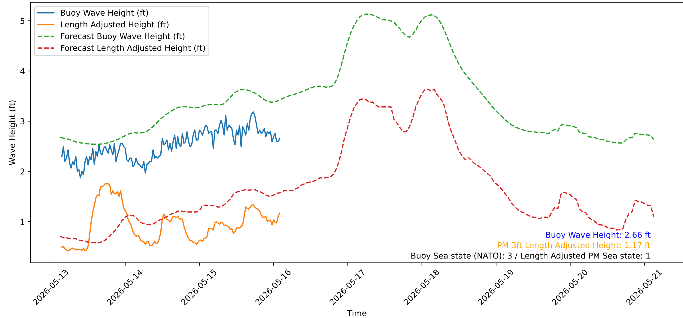
Wave Heights over Time for Red Beach at 2026-05-16 03:00:51
