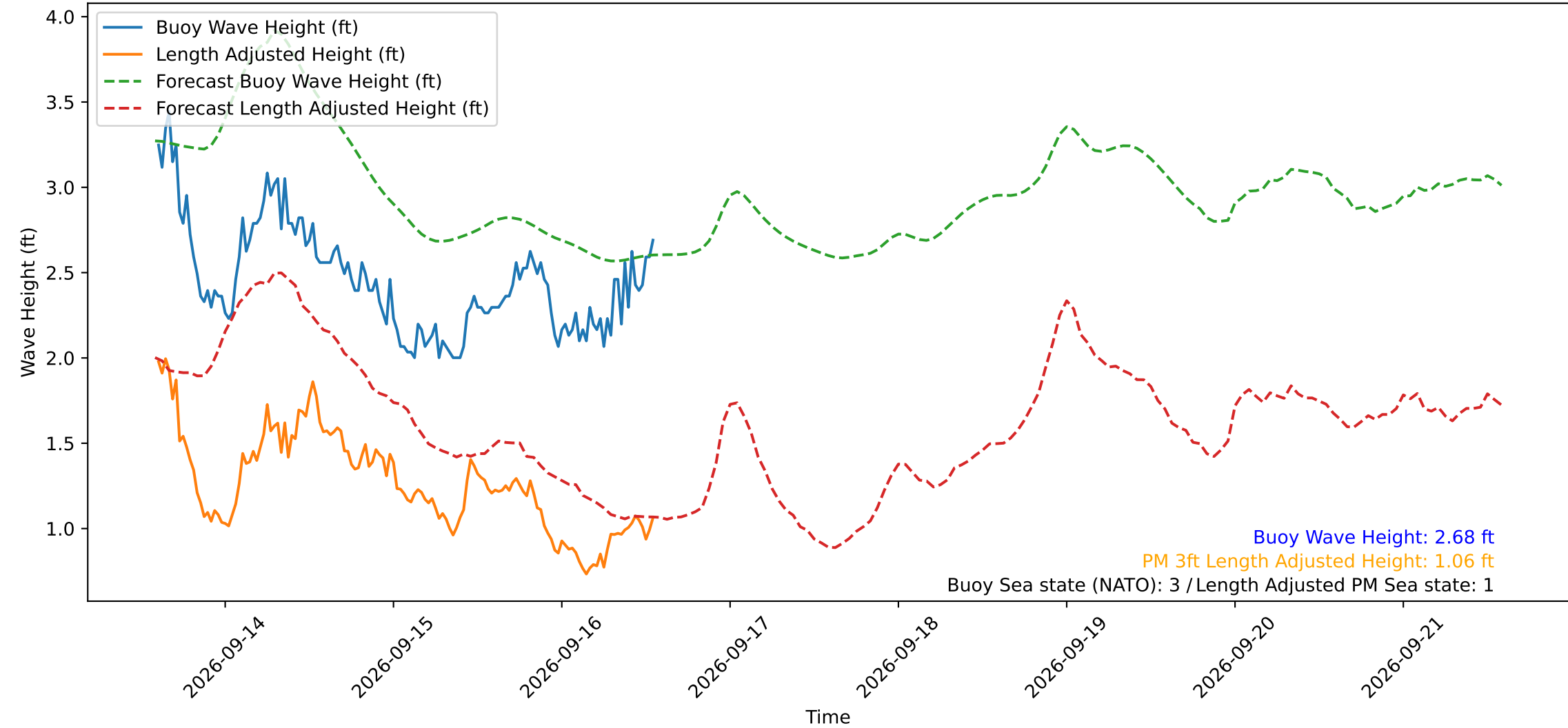
Wave Heights over Time for Red Beach at 2026-09-16 14:00:49
