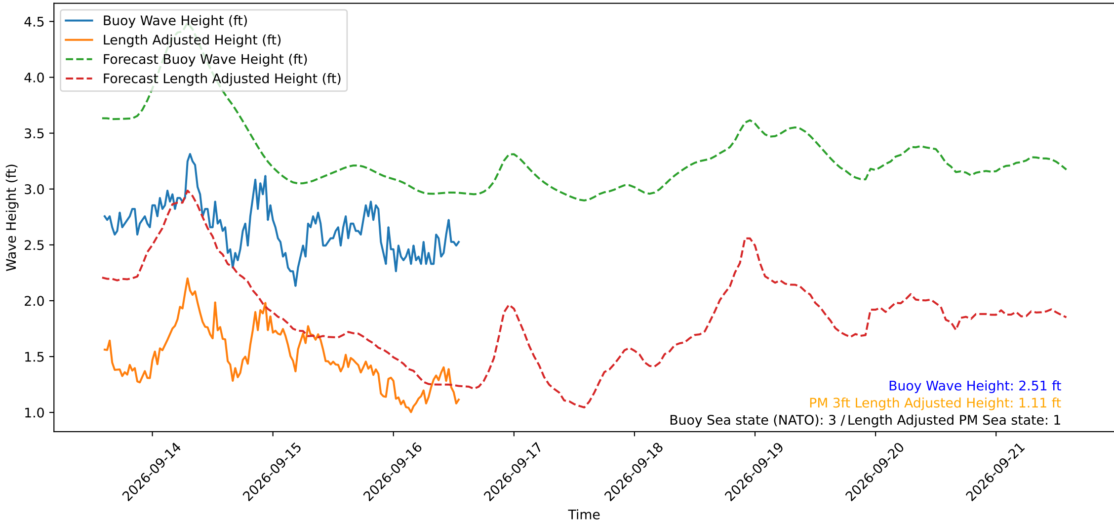
Wave Heights over Time for Green Beach at 2026-09-16 14:01:11
