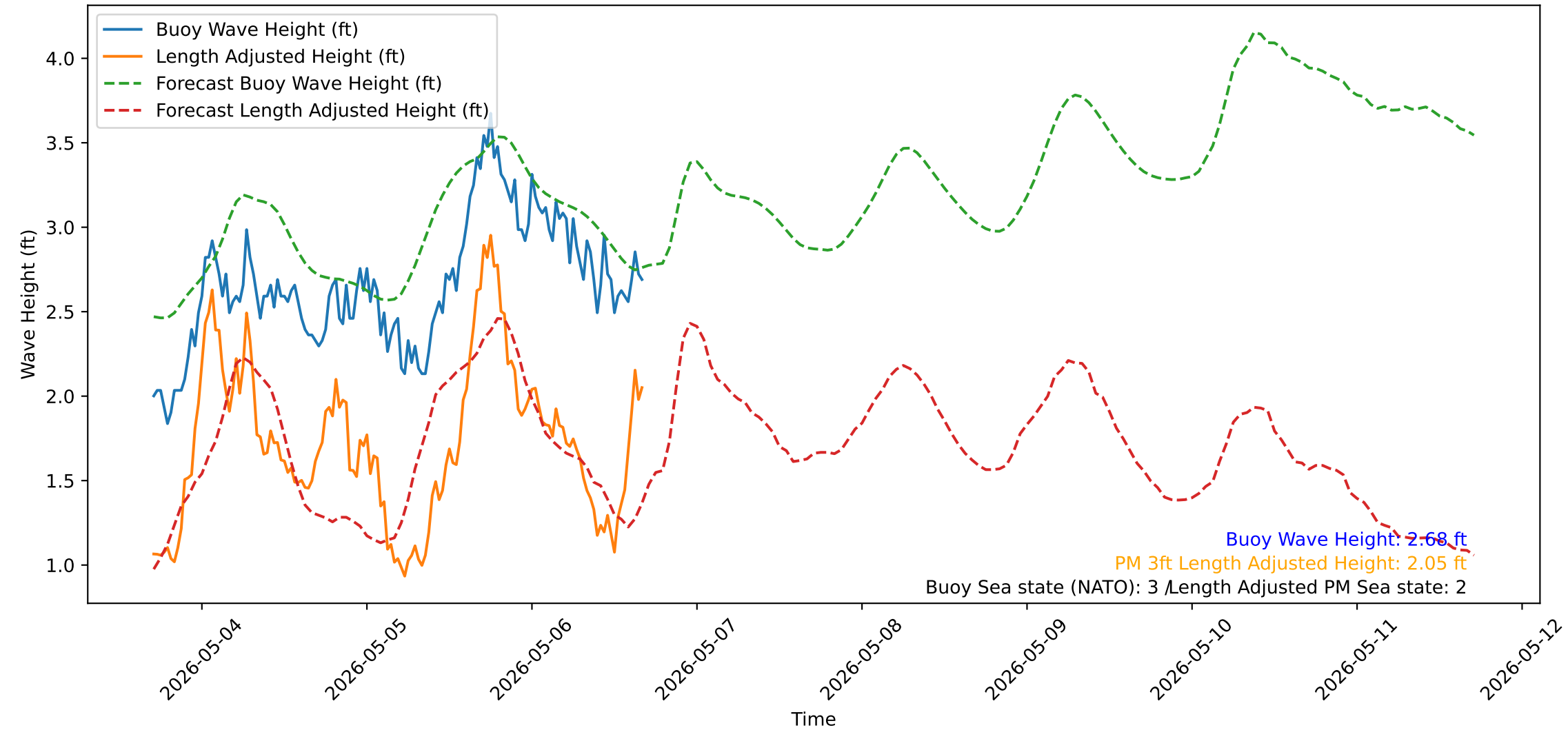
Wave Heights over Time for Green Beach at 2026-05-06 16:51:15
