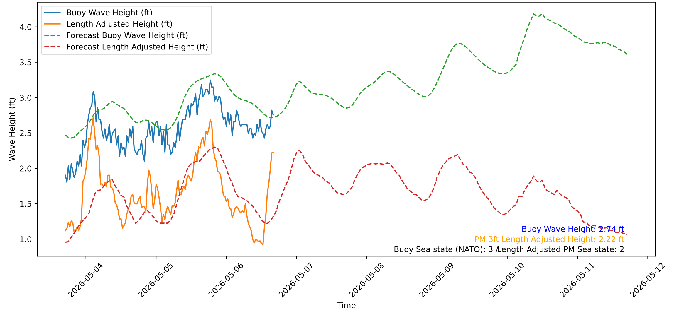
Wave Heights over Time for Oceanside Harbor at 2026-05-06 16:50:31
