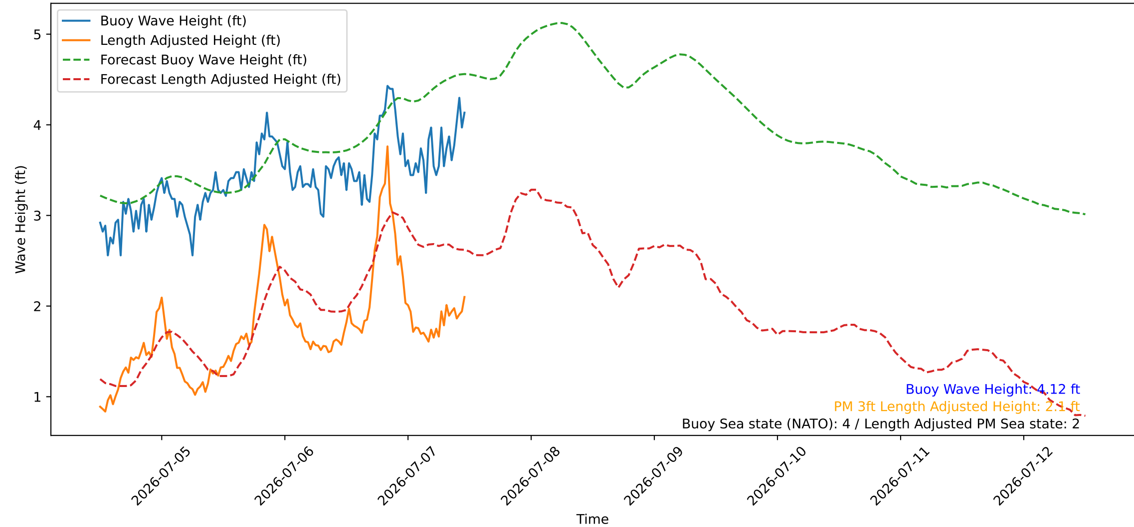
Wave Heights over Time for Green Beach at 2026-07-07 12:01:08
