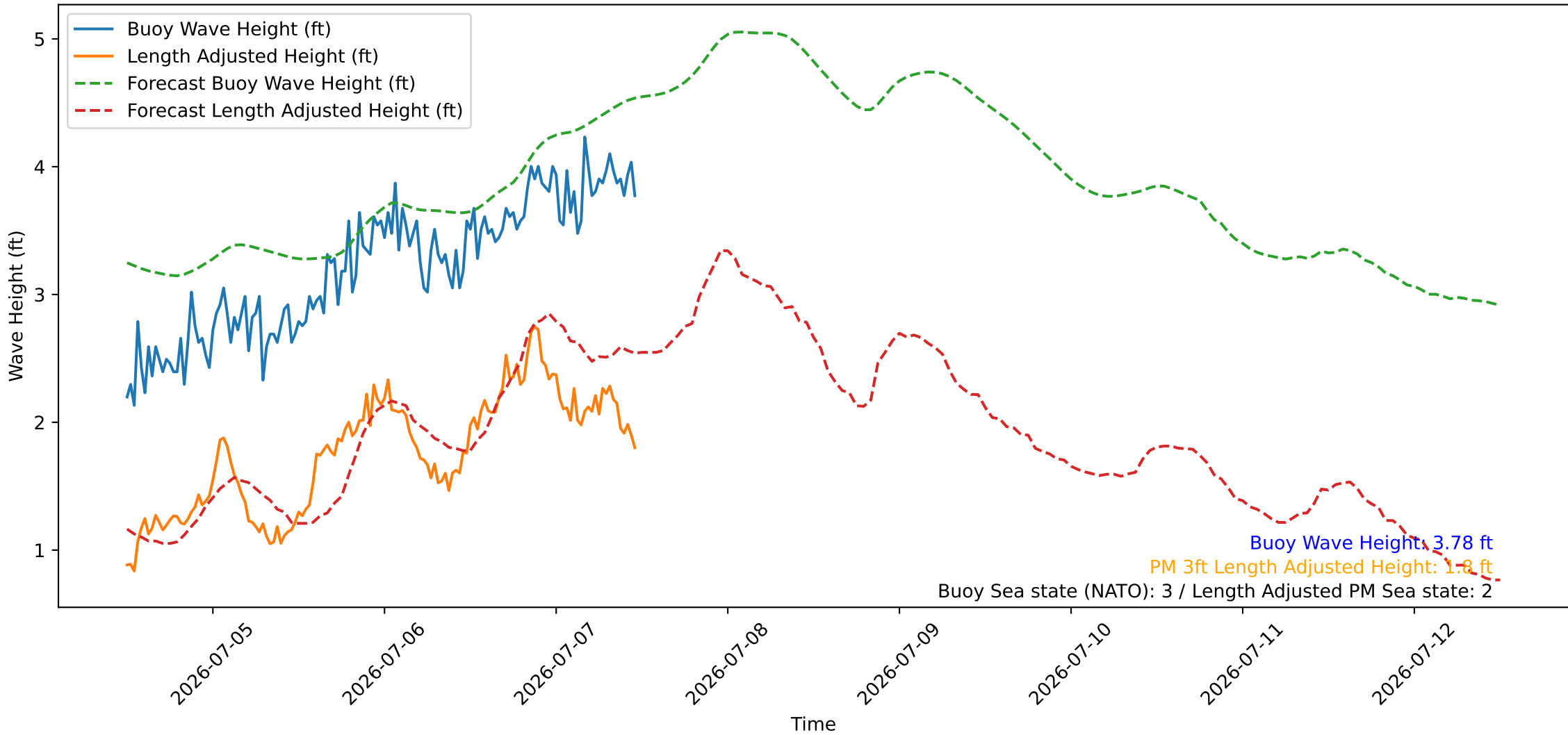
Wave Heights over Time for Oceanside Harbor at 2026-07-07 12:00:26
