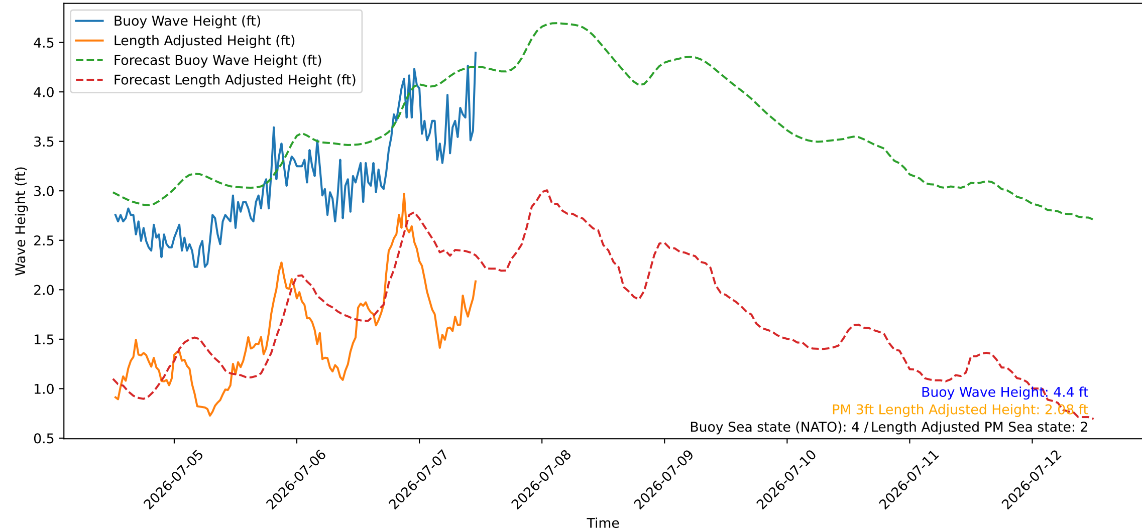
Wave Heights over Time for Red Beach at 2026-07-07 12:00:45
