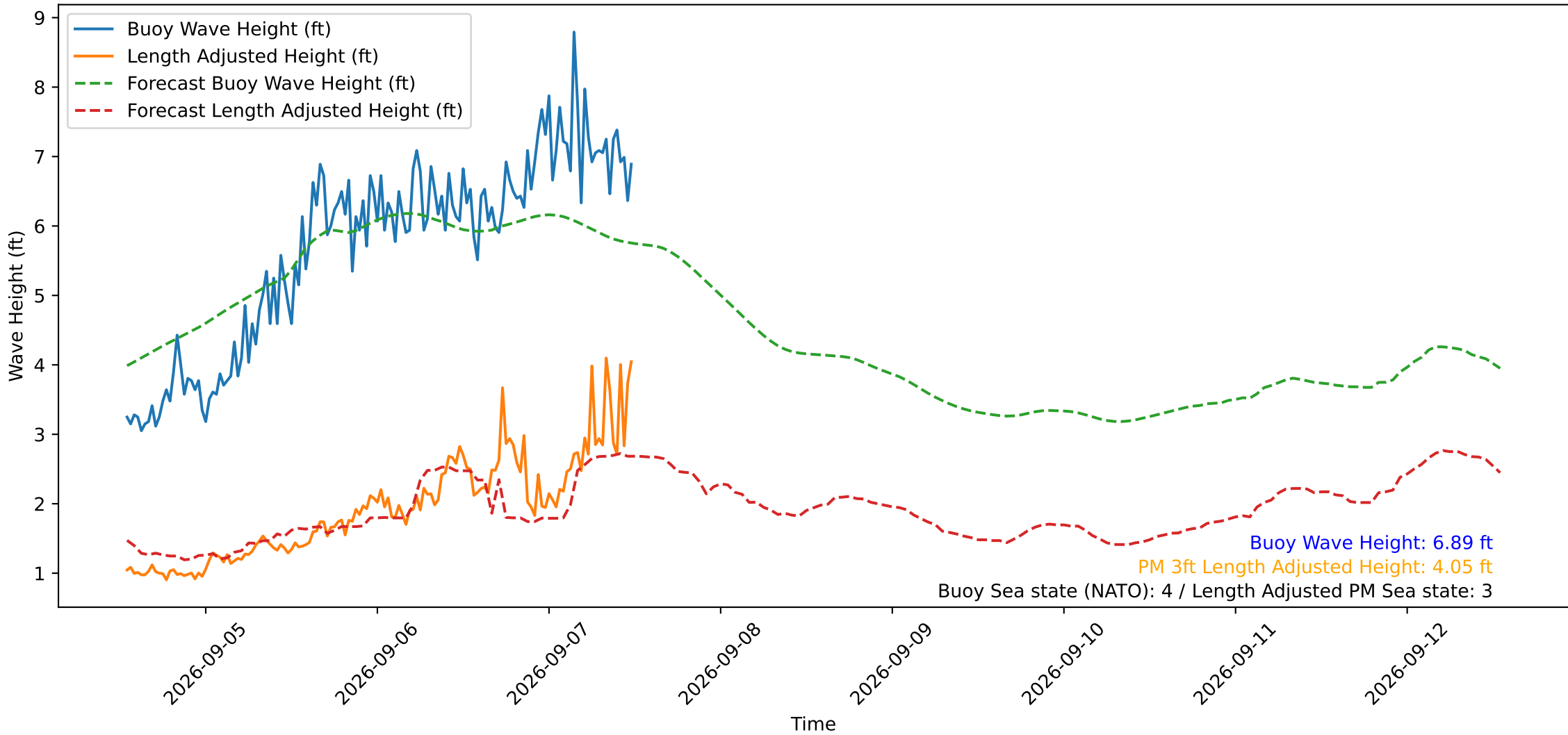
Wave Heights over Time for Green Beach at 2026-09-07 12:31:12
