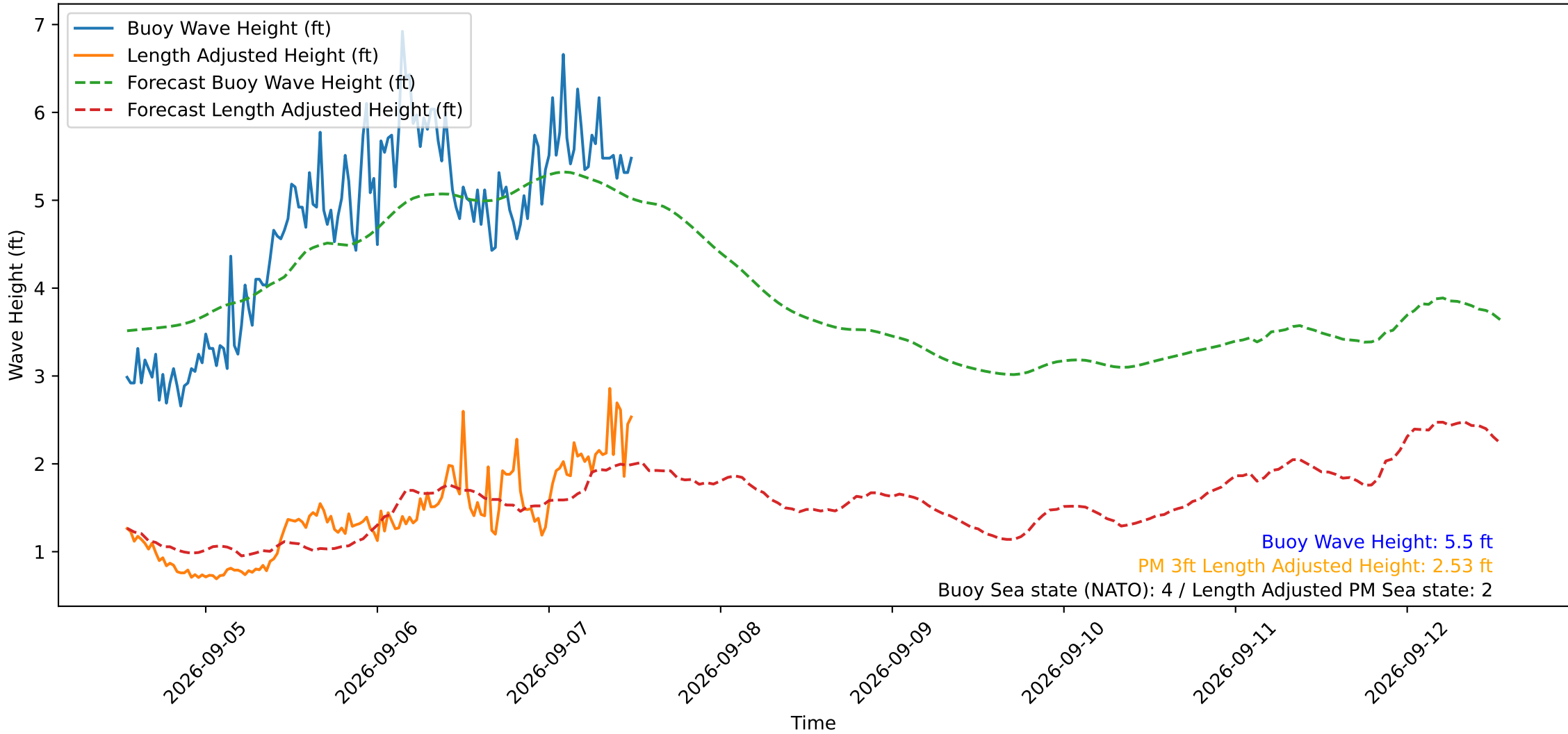
Wave Heights over Time for Red Beach at 2026-09-07 12:30:49
