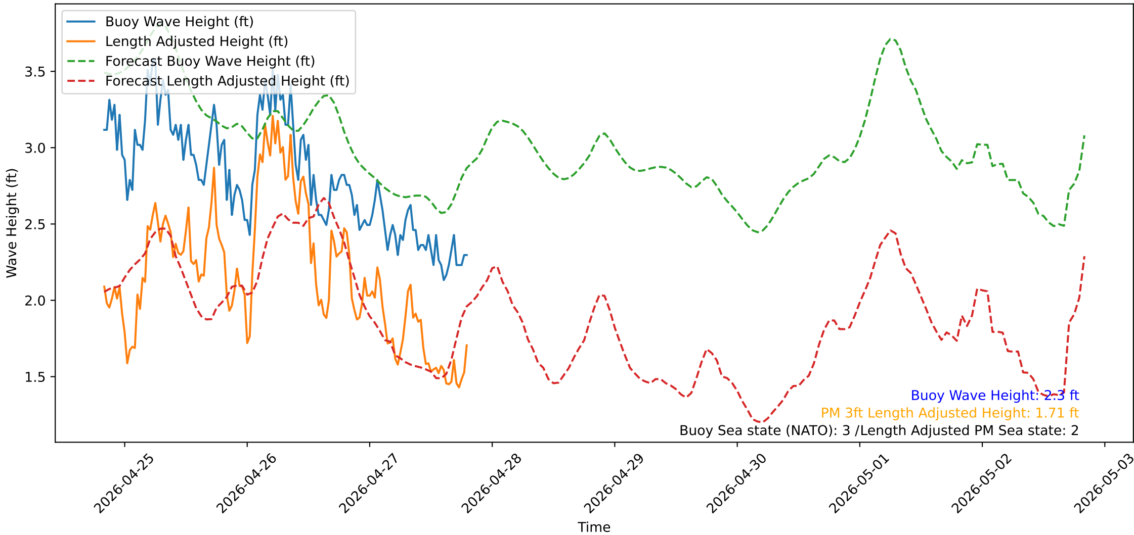
Wave Heights over Time for Green Beach at 2026-04-27 20:01:12
