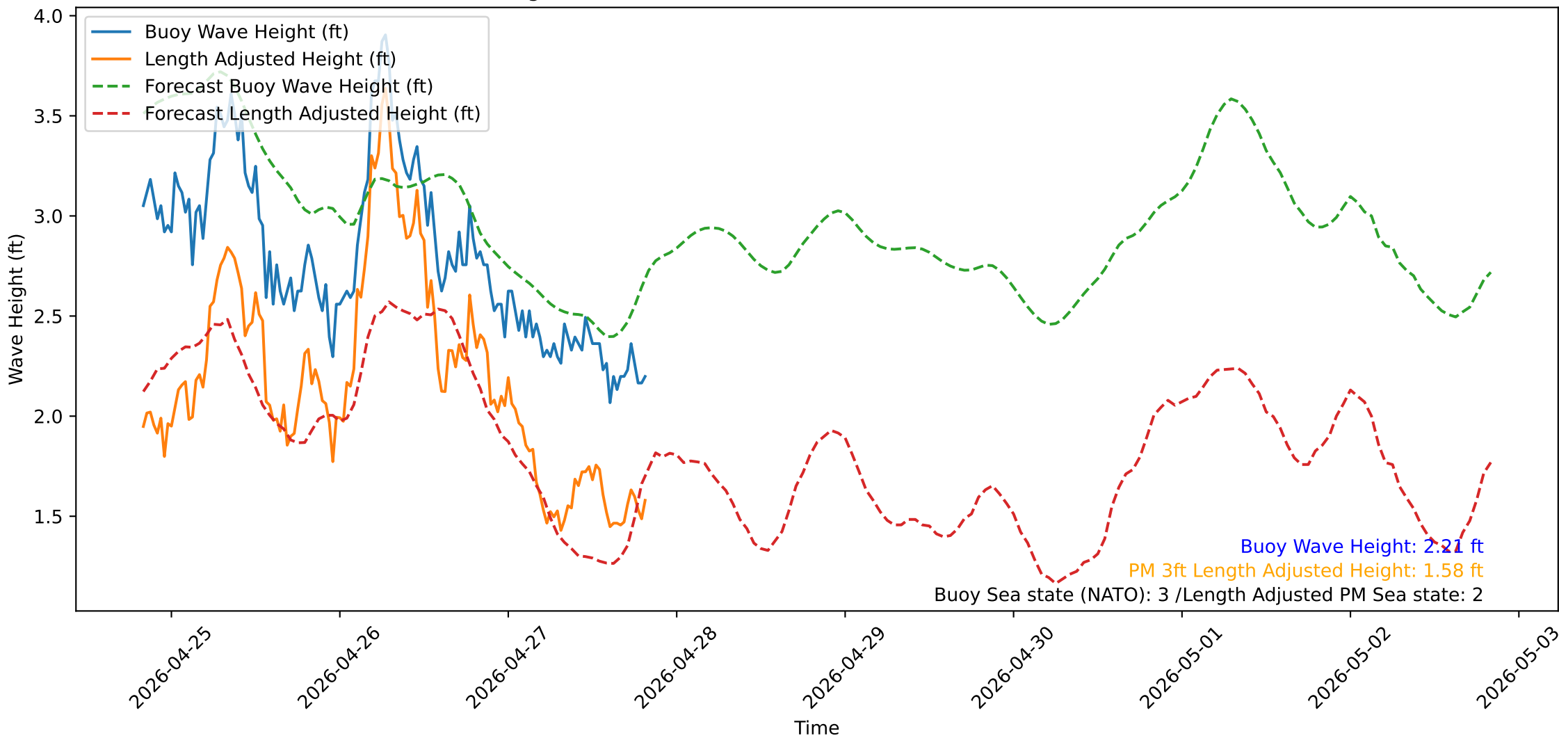
Wave Heights over Time for Oceanside Harbor at 2026-04-27 20:00:31
