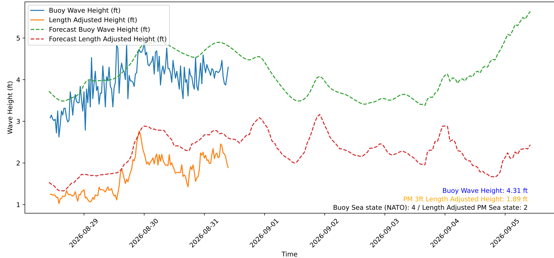
Wave Heights over Time for Green Beach at 2026-08-31 10:21:14
