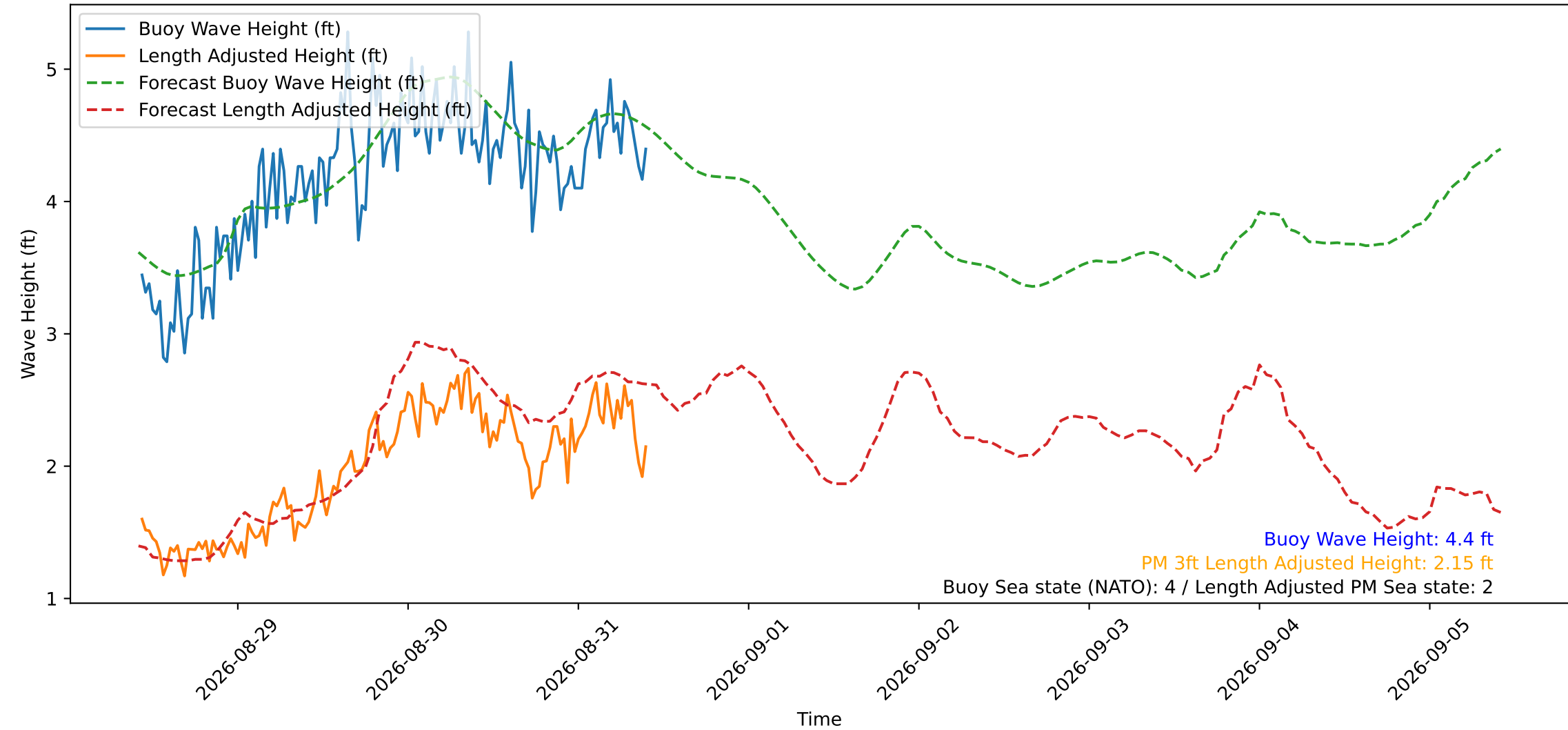
Wave Heights over Time for Oceanside Harbor at 2026-08-31 10:20:29
