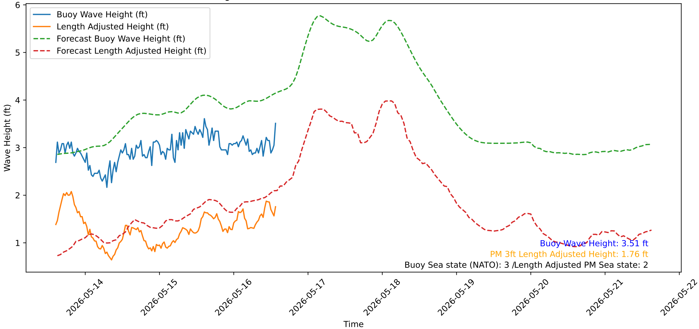
Wave Heights over Time for Oceanside Harbor at 2026-05-16 14:40:31
