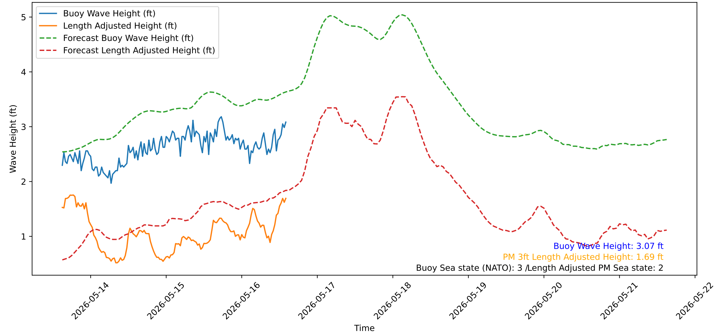
Wave Heights over Time for Red Beach at 2026-05-16 14:40:50
