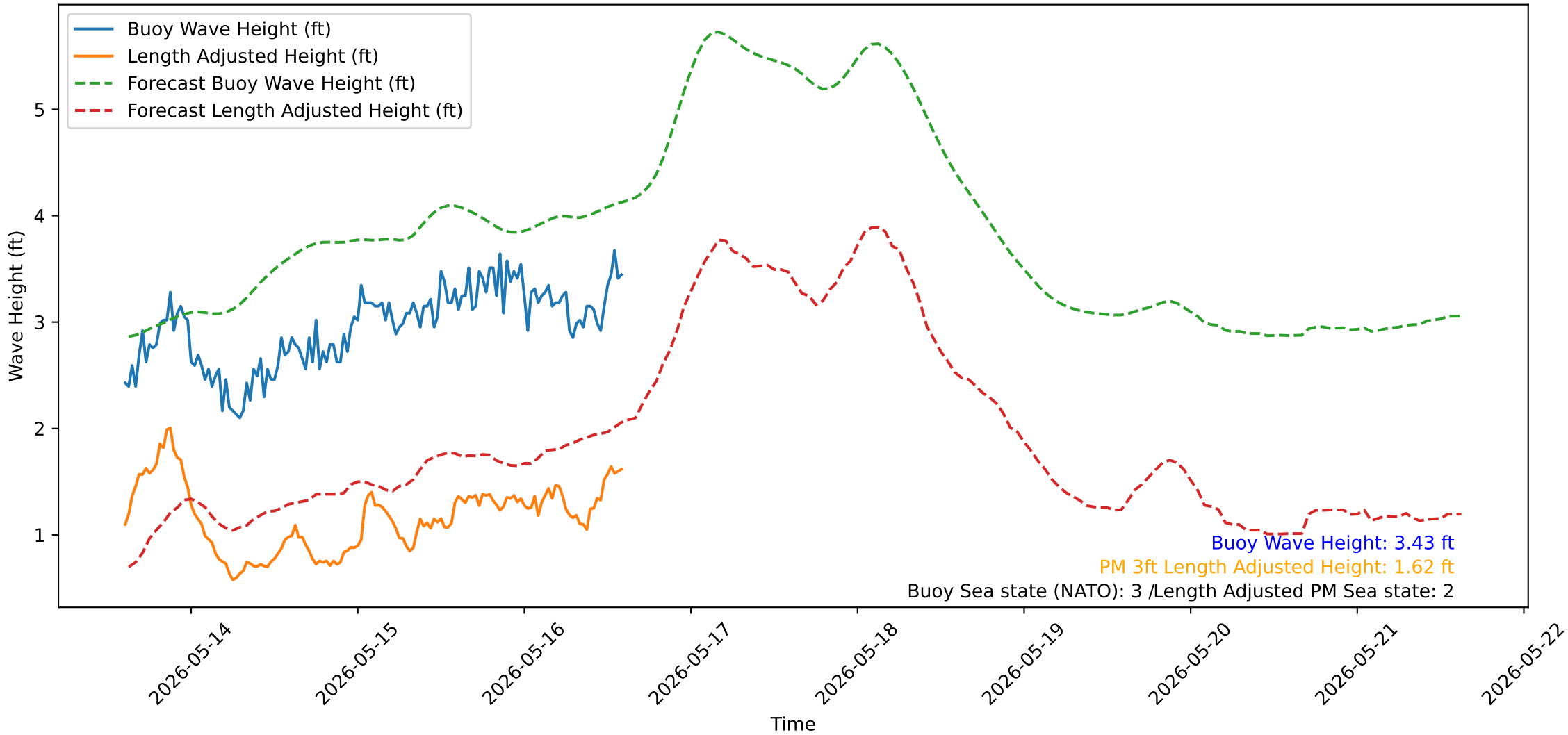
Wave Heights over Time for Green Beach at 2026-05-16 14:41:13
