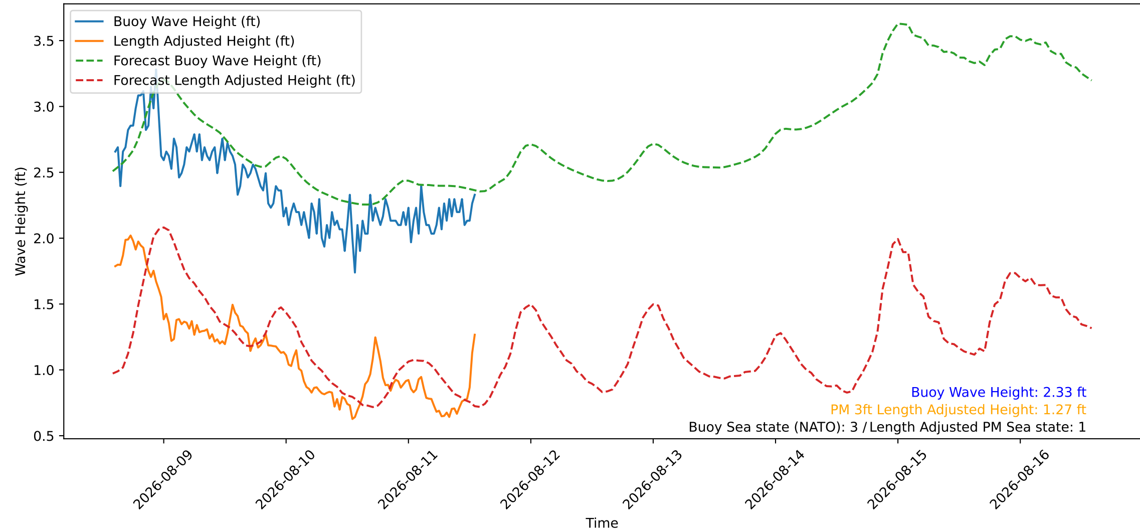
Wave Heights over Time for Red Beach at 2026-08-11 14:00:46
