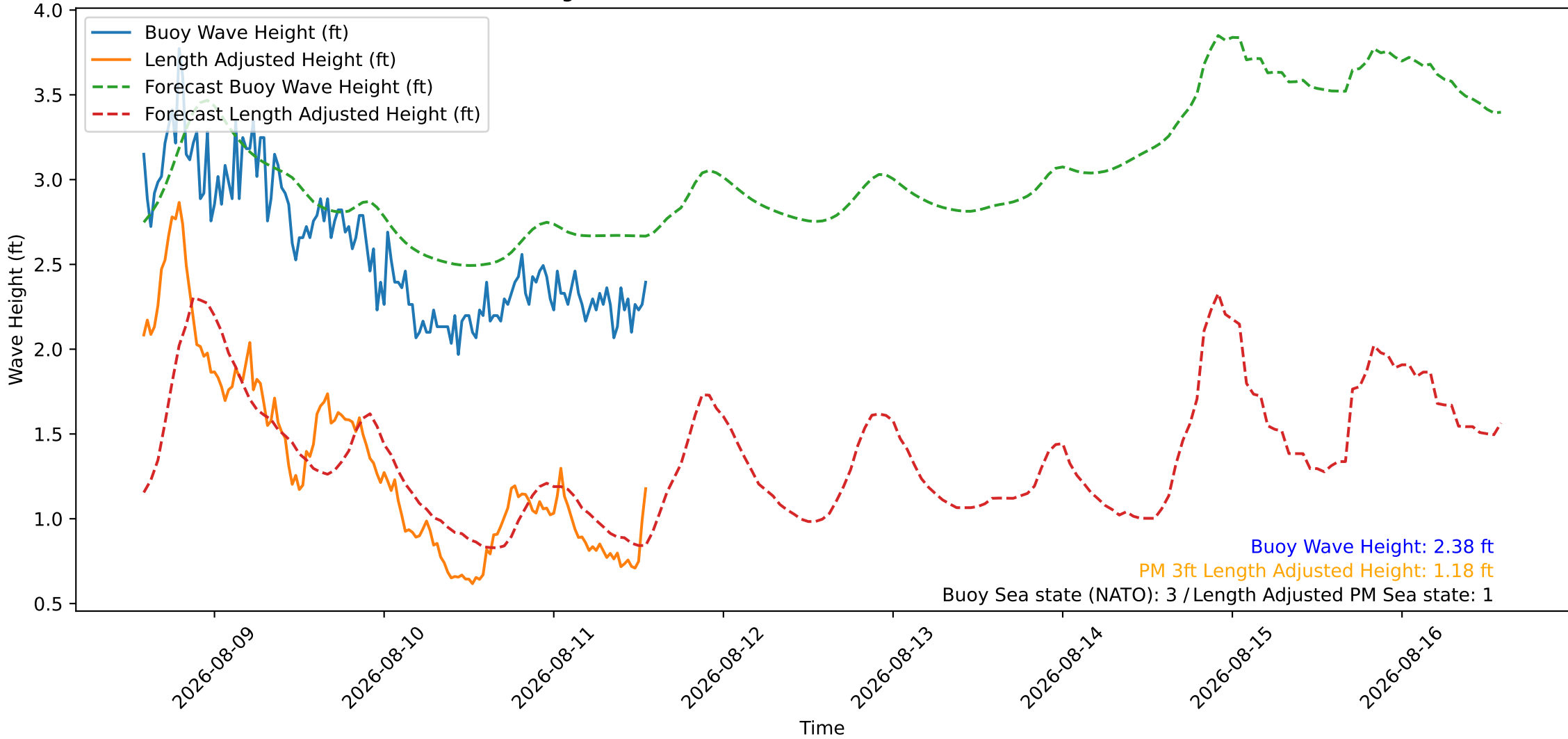
Wave Heights over Time for Green Beach at 2026-08-11 14:01:09
