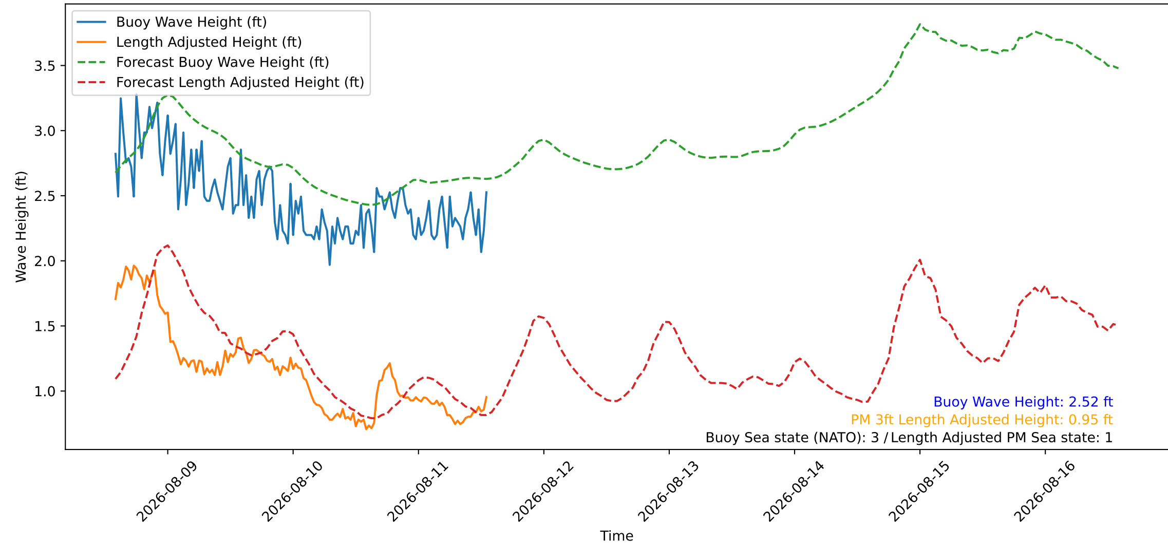
Wave Heights over Time for Oceanside Harbor at 2026-08-11 14:00:26
