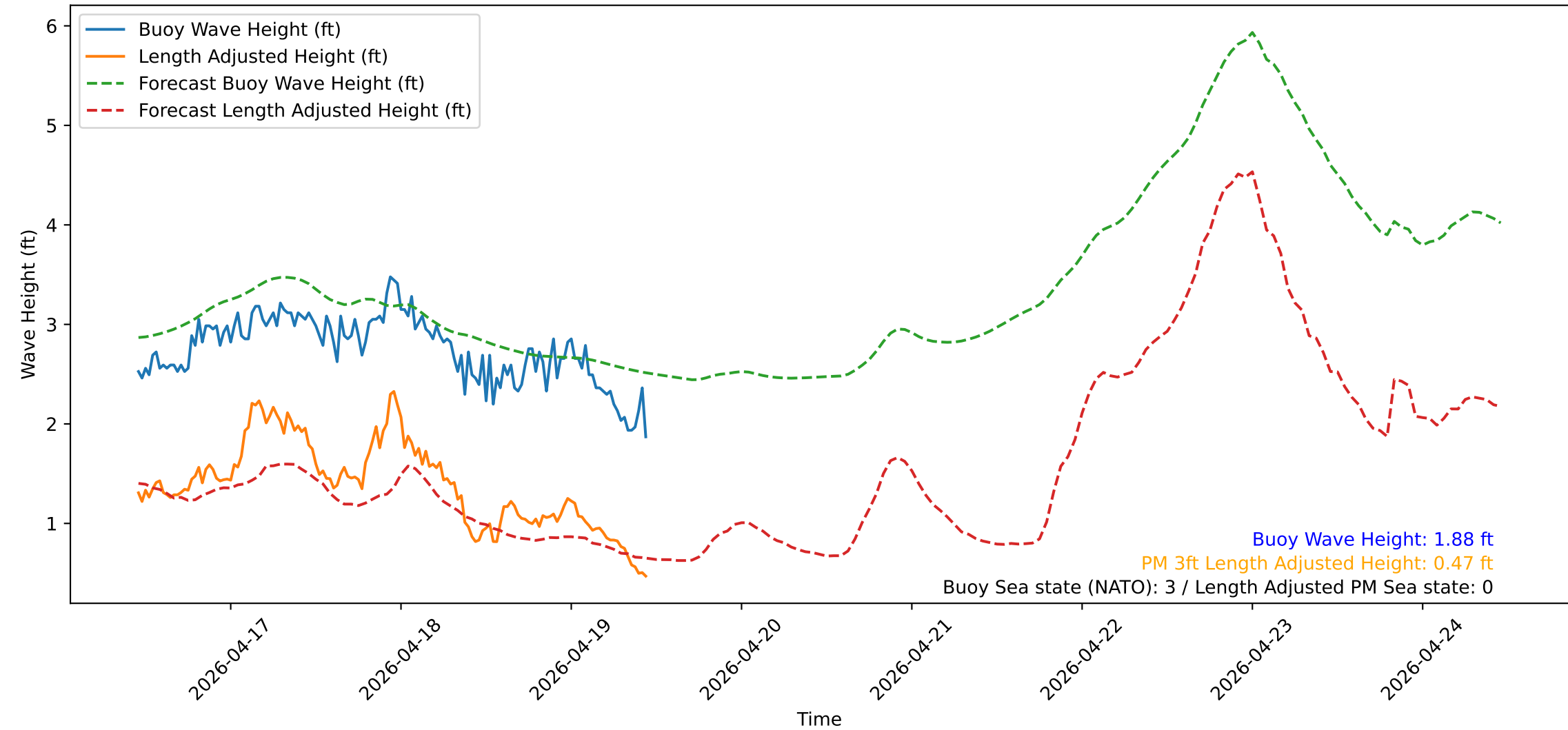
Wave Heights over Time for Green Beach at 2026-04-19 11:11:13
