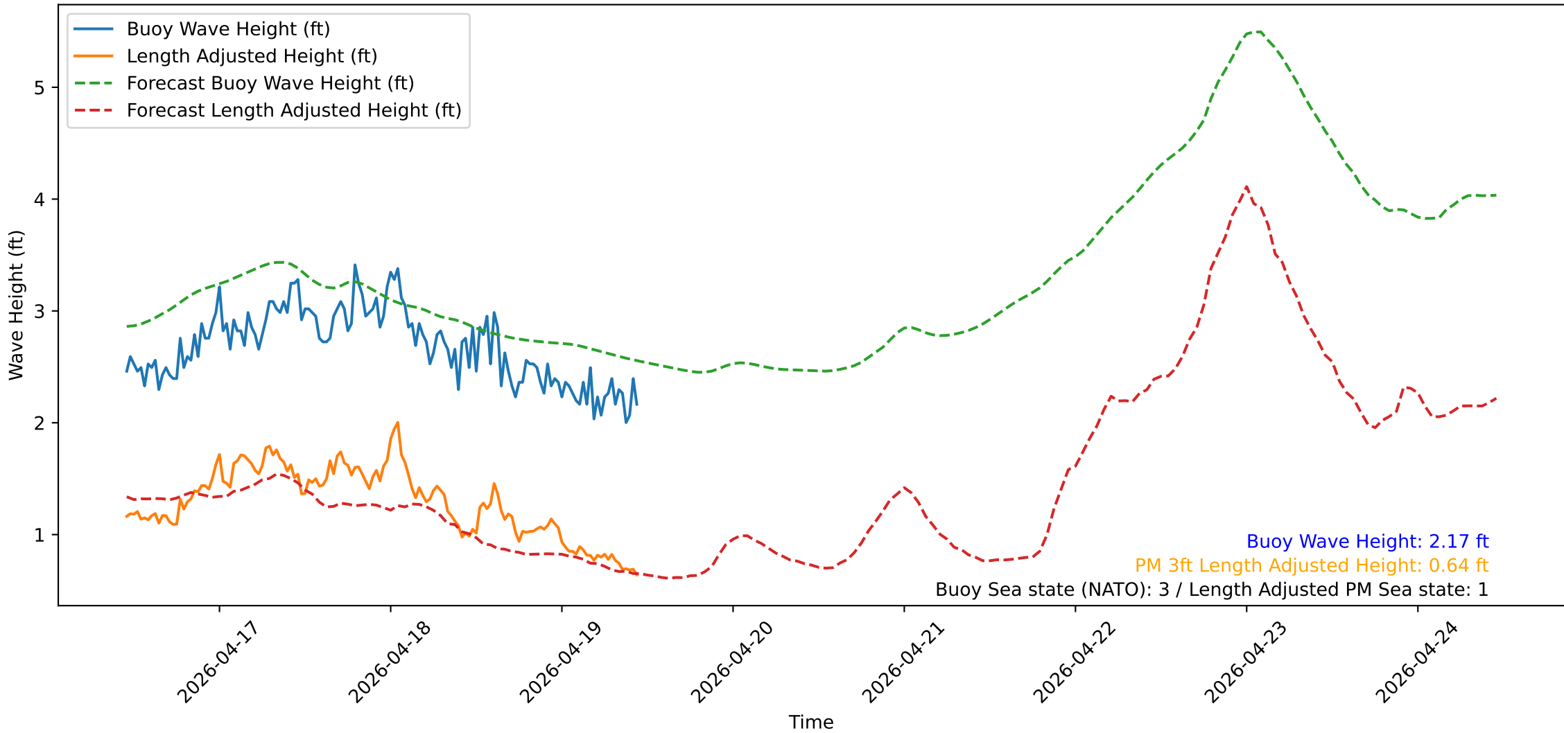
Wave Heights over Time for Oceanside Harbor at 2026-04-19 11:10:31
